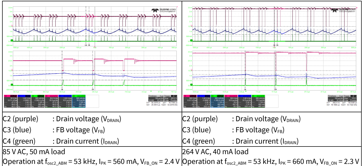
Figure 15 ABM operation
