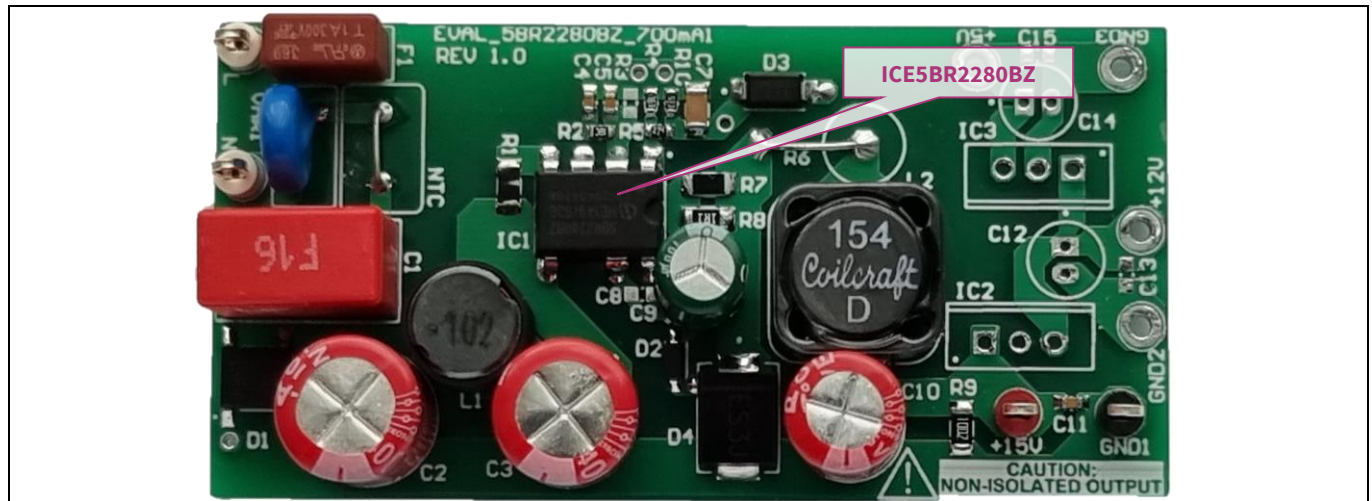
Figure 1 EVAL_5BR2280BZ_700mA1
