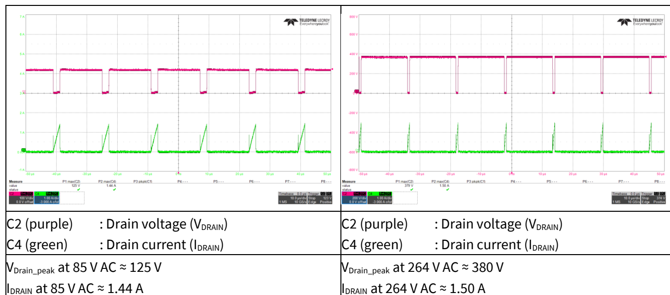
Figure 13 Drain and CS voltage at maximum load
