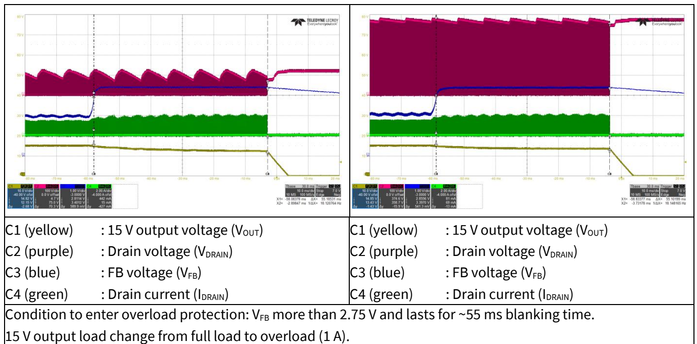
Figure 16 Overload protection
