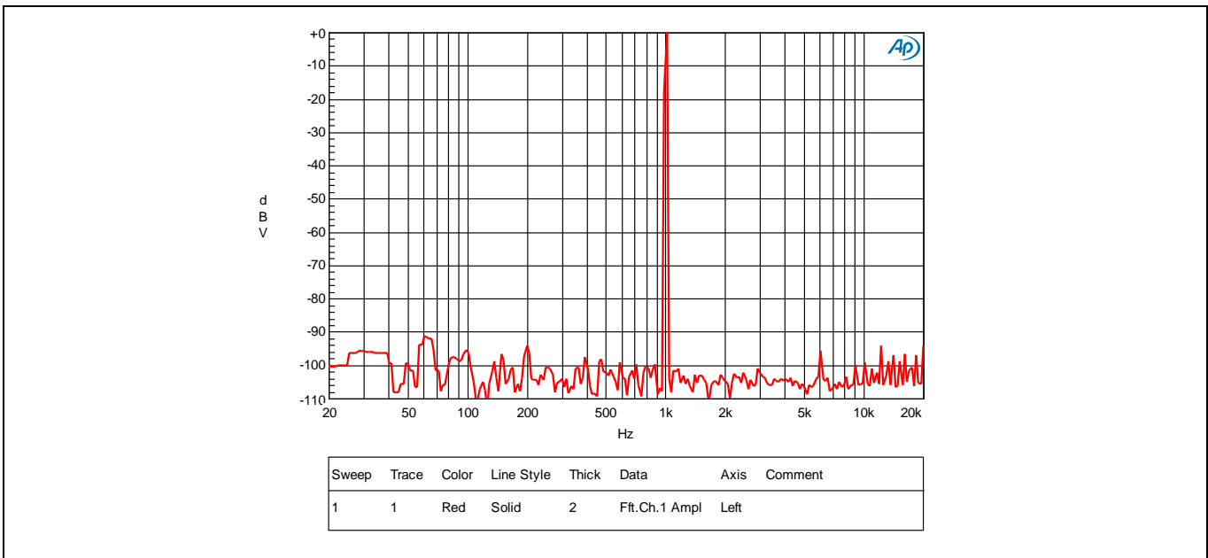
Figure 11 Noise floor with 1 V RMS output 4 Ω load
