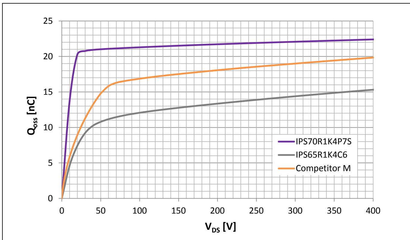
Figure 8 Q_{oss} comparison of 1400 mΩ devices
