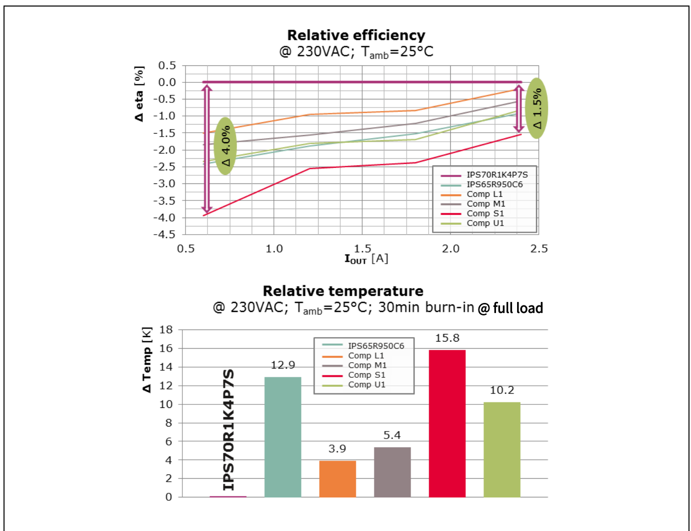
Figure 12 Efficiency and thermal comparison – 12 W customer charger at 25^{\circ}\text{C} ambient and 230 V AC input voltage
