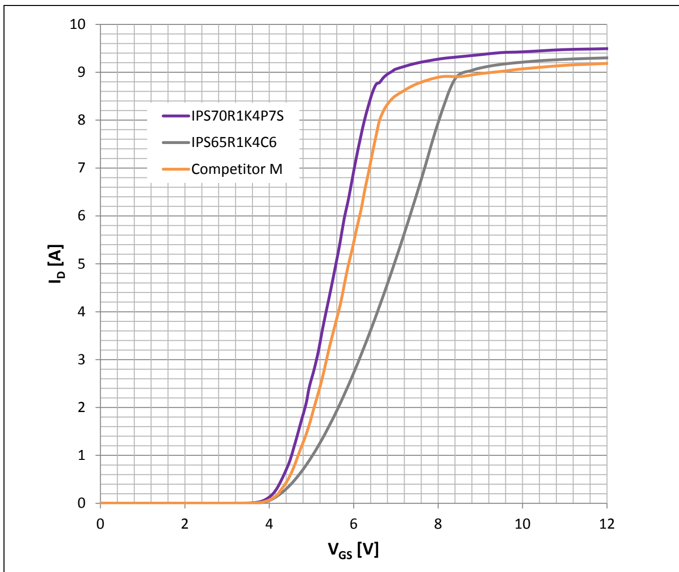
Figure 9 Transfer characteristics comparison of 1400 mΩ devices at 25°C
