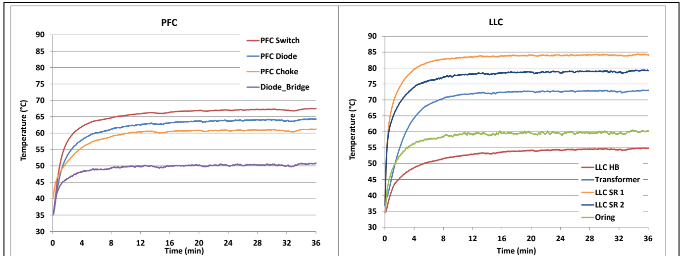
Figure 22 Temperature evolution with operation time in EVAL_1K6W_PSU_G7_DD at nominal input and load conditions, and room temperature.
