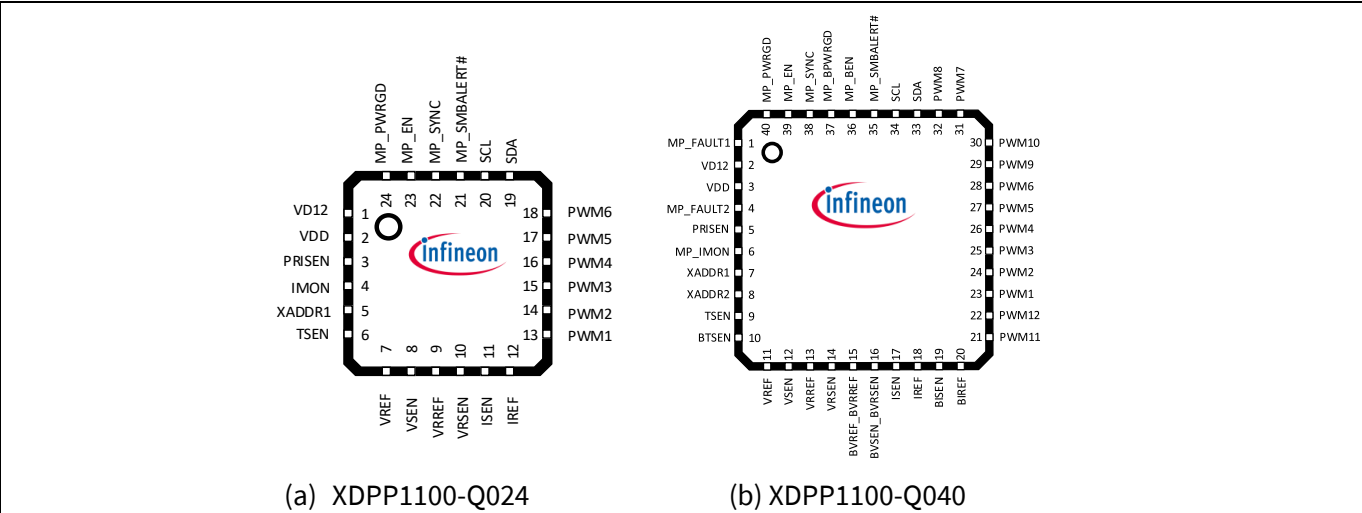
Figure 12 XDPP1100 pin-out
