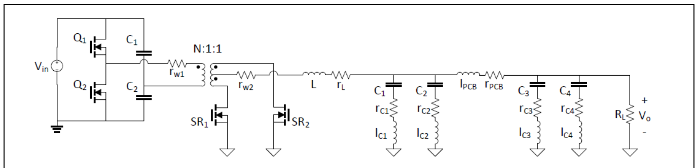
Figure 125 HBCT schematic
