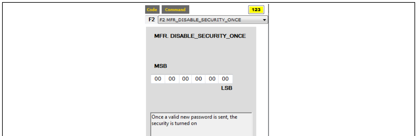
Figure 187 MFR_DISABLE_SECURITY_ONCE
