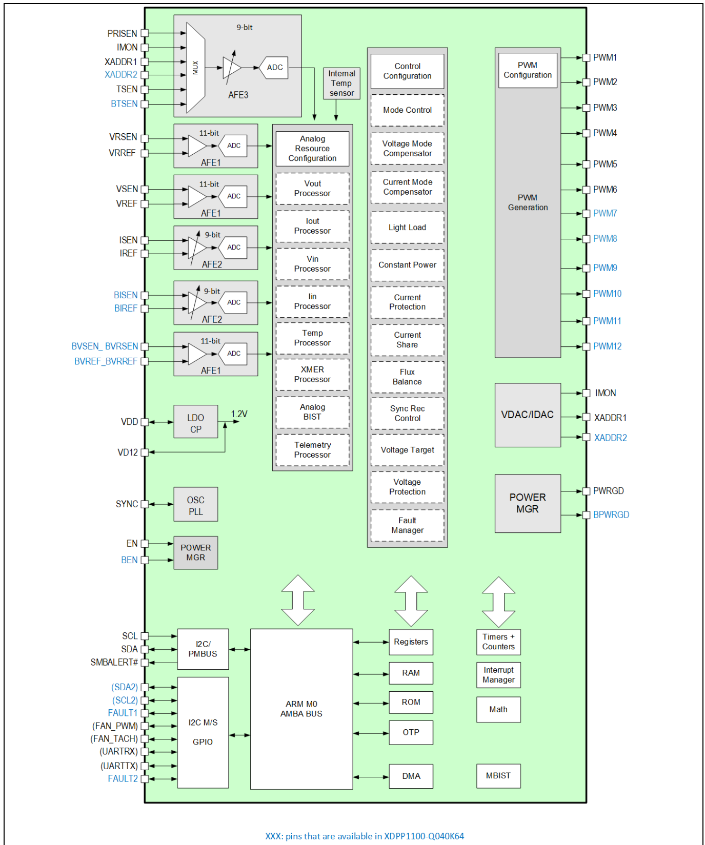
Figure 2 Block diagram
