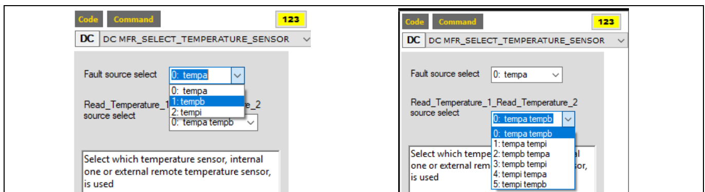
Figure 153 MFR_SELECT_TEMPERATURE_SENSOR command
