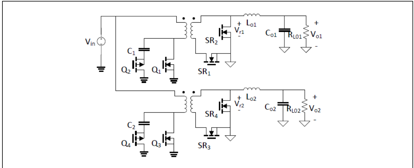
Figure 144 Dual-loop ACF schematic
