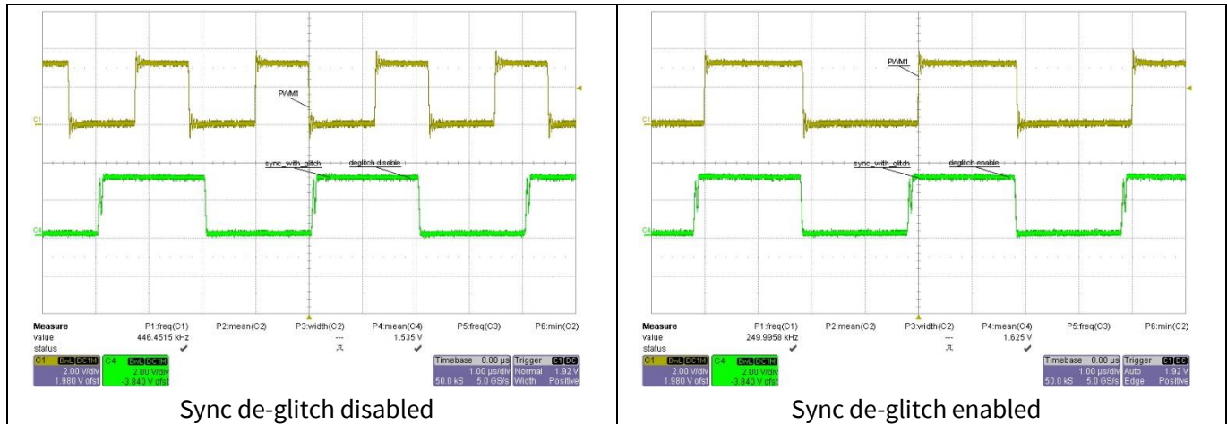
Figure 139 Sync de-glitch waveforms
