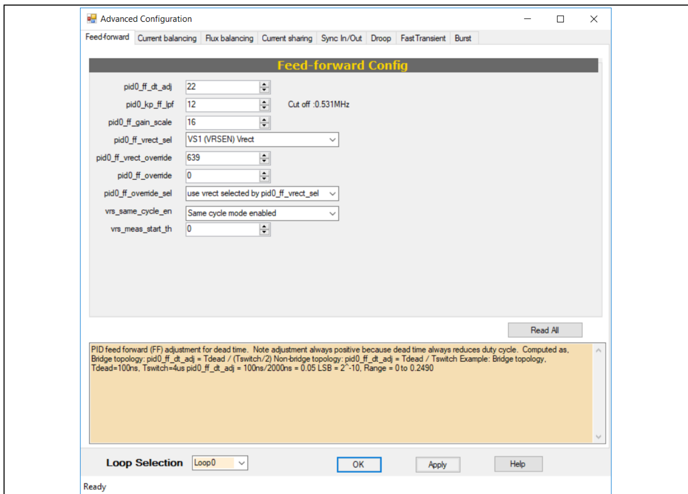
Figure 31 GUI design tools – input voltage feed-forward
