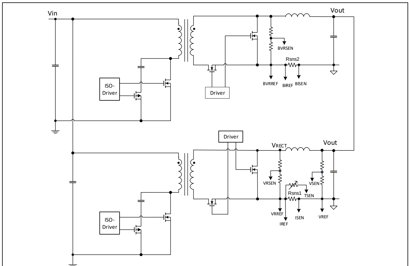
Figure 41 Interleaved ACF
