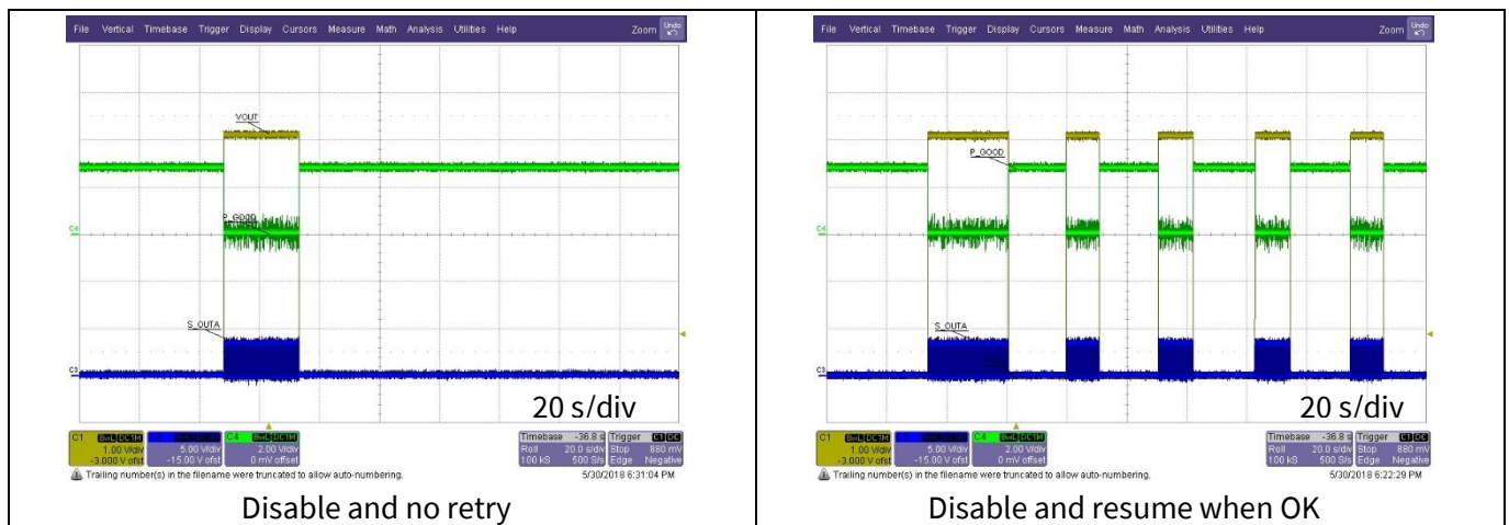
Figure 176 Overtemperature protection waveform (HBCT converter with V_{\text{OUT}} = 5 \text{ V} )
