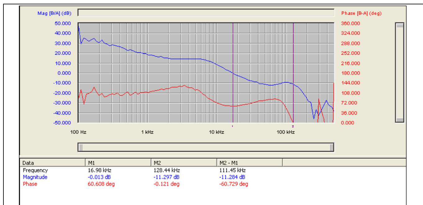
Figure 72 Actual bode plot of the FB-FB converter at 48 V input and 12 V/50 A load
