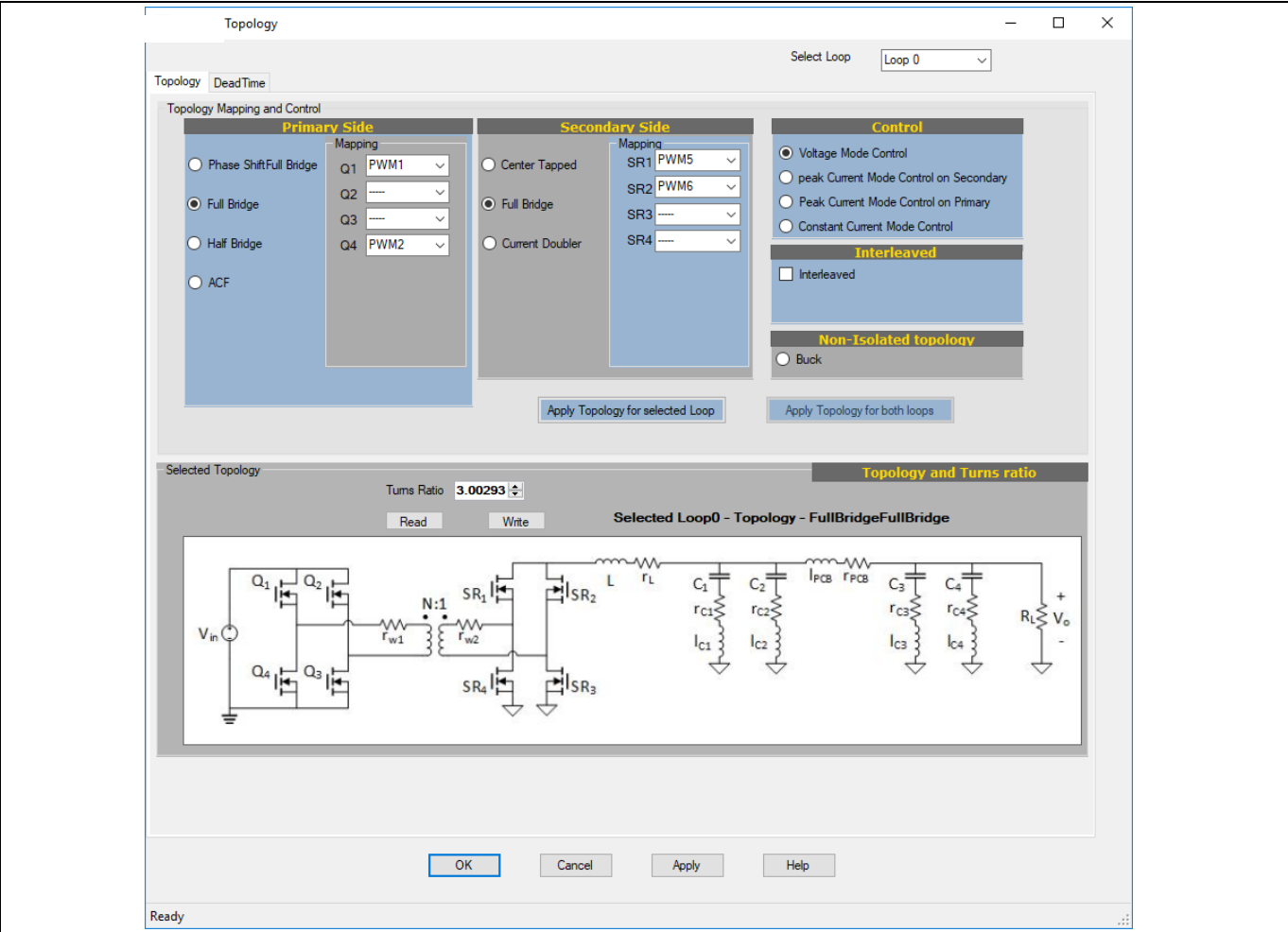
Figure 11 GUI design tool – topology selection and PWM mapping
