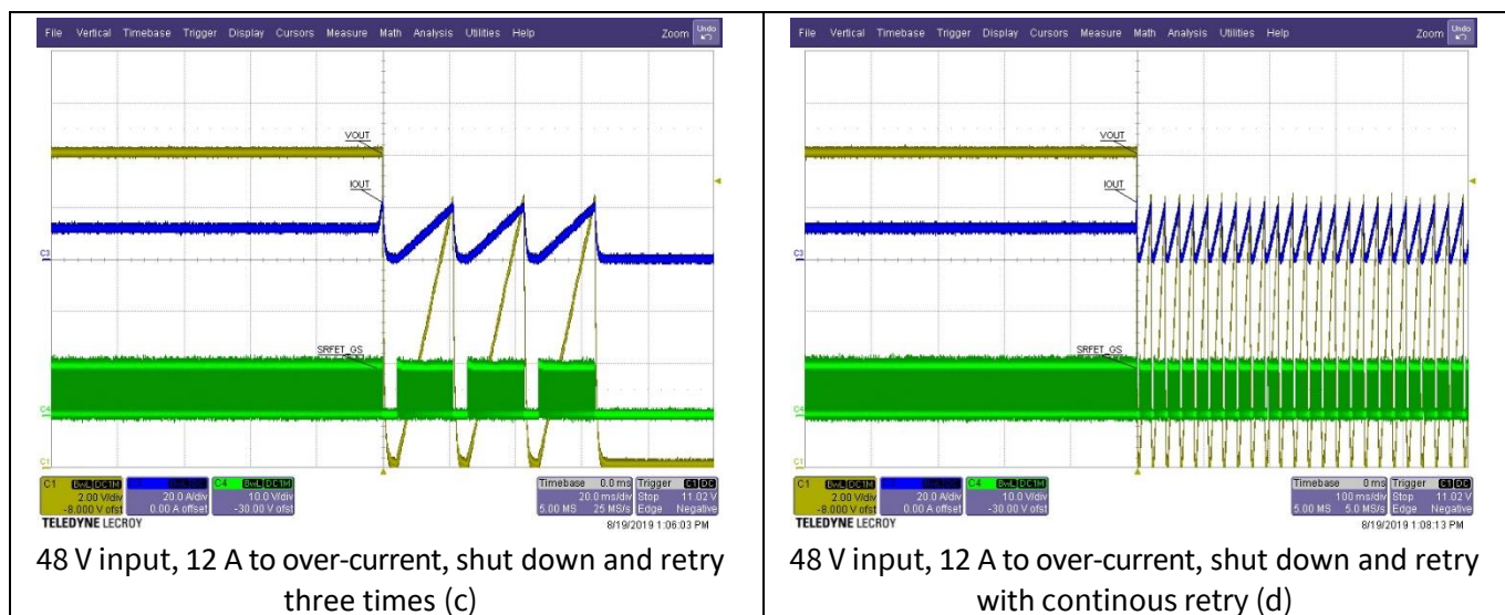
Figure 170 Output OCP waveform
