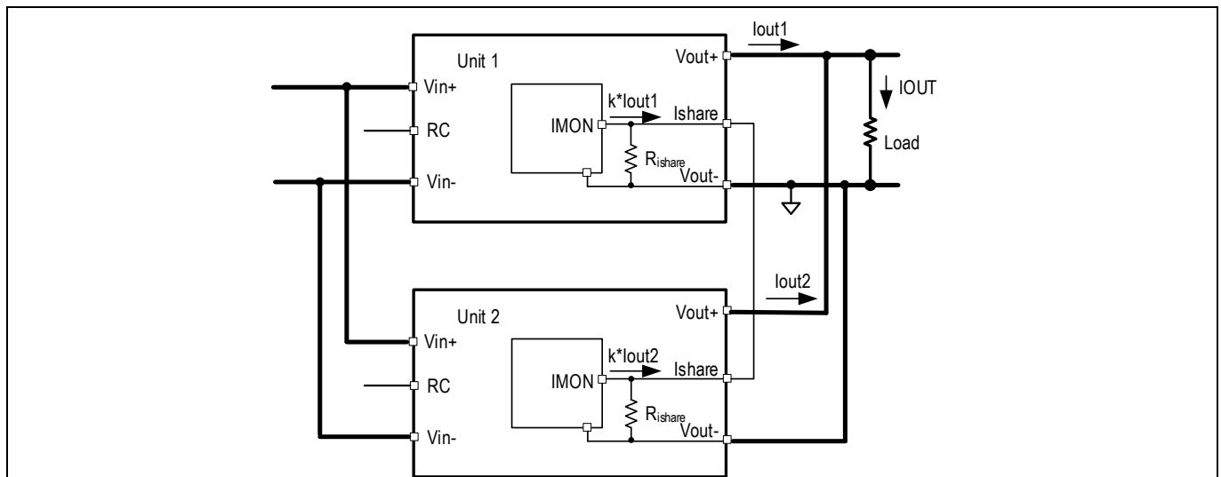
Figure 80 XDPP1100 active current sharing
