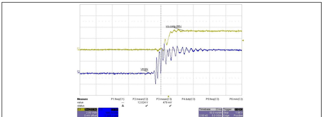
Figure 20 VRS noise
