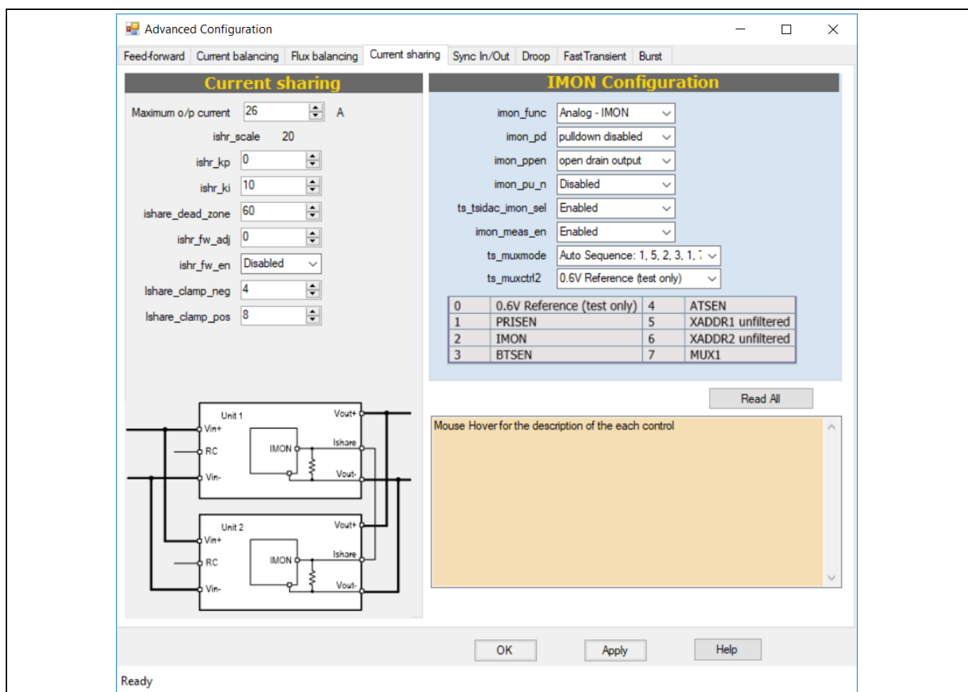
Figure 85 GUI design tool
