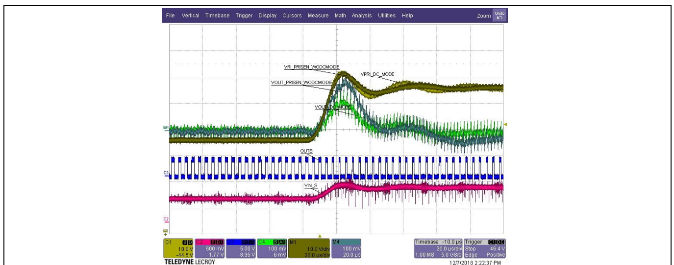
Figure 39 FB-FB, 40 V to 70 V line transient (overshoot reduced from 180 mV to 100 mV)
