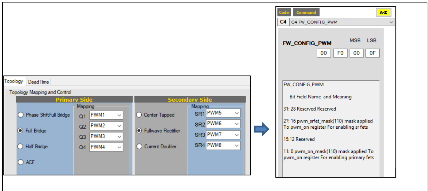
Figure 61 FW_CONFIG_PWM
