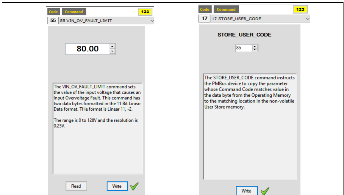
Figure 200 STORE_USER_CODE
