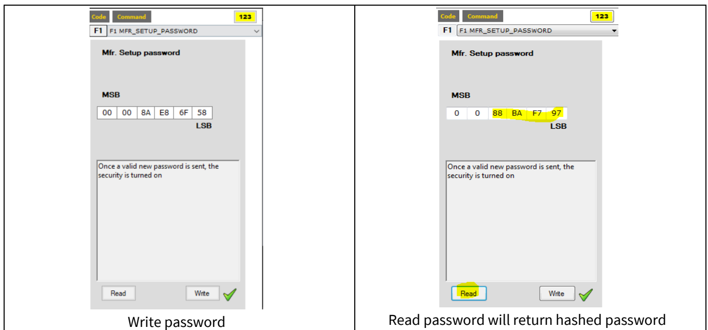
Figure 186 MFR_SETUP_PASSWORD
