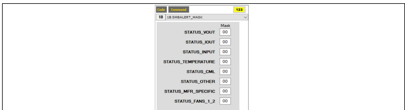
Figure 181 SMBALERT_MASK configuration
