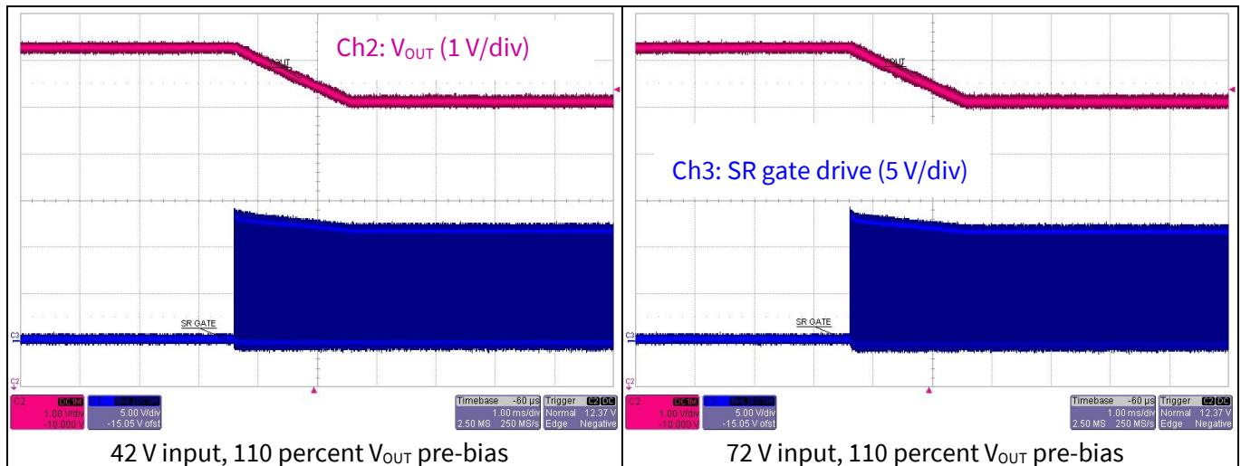
Figure 36 Pre-bias start-up waveforms with pre-bias voltage 13.2 V
