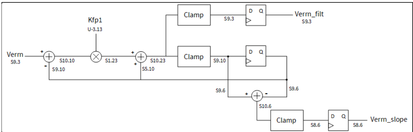
Figure 67 Pre-filter block diagram
