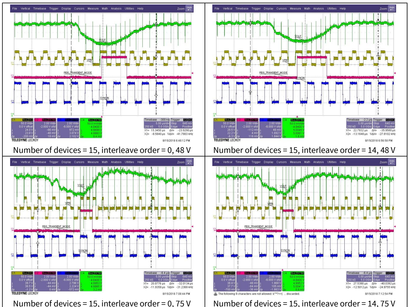
Figure 150 Sync-in test with a step-load transient from 0 to 16.66 A using a 0.3 Ω resistor
