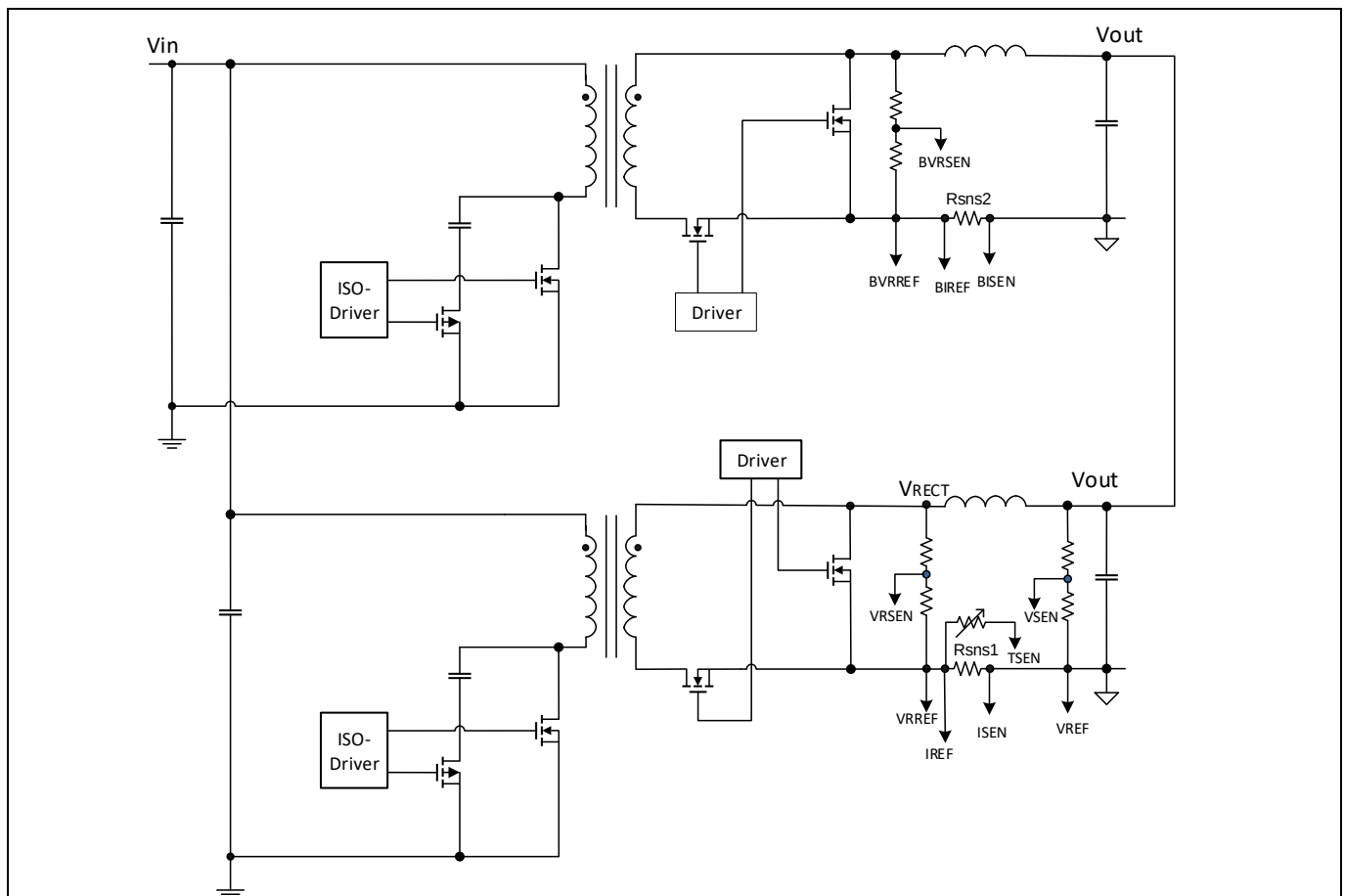
Figure 9 Interleaved ACF
