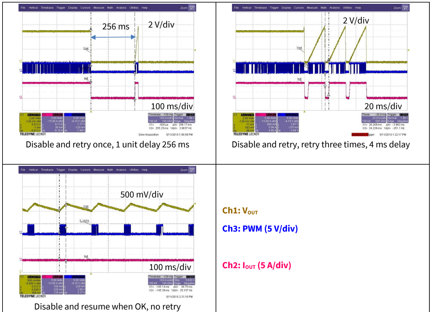
Figure 164 Output OVP waveform ( V_{OUT} = 5\text{ V} , OVP fault threshold = 5.8\text{ V} , OVP warning threshold = 5.5\text{ V} )
