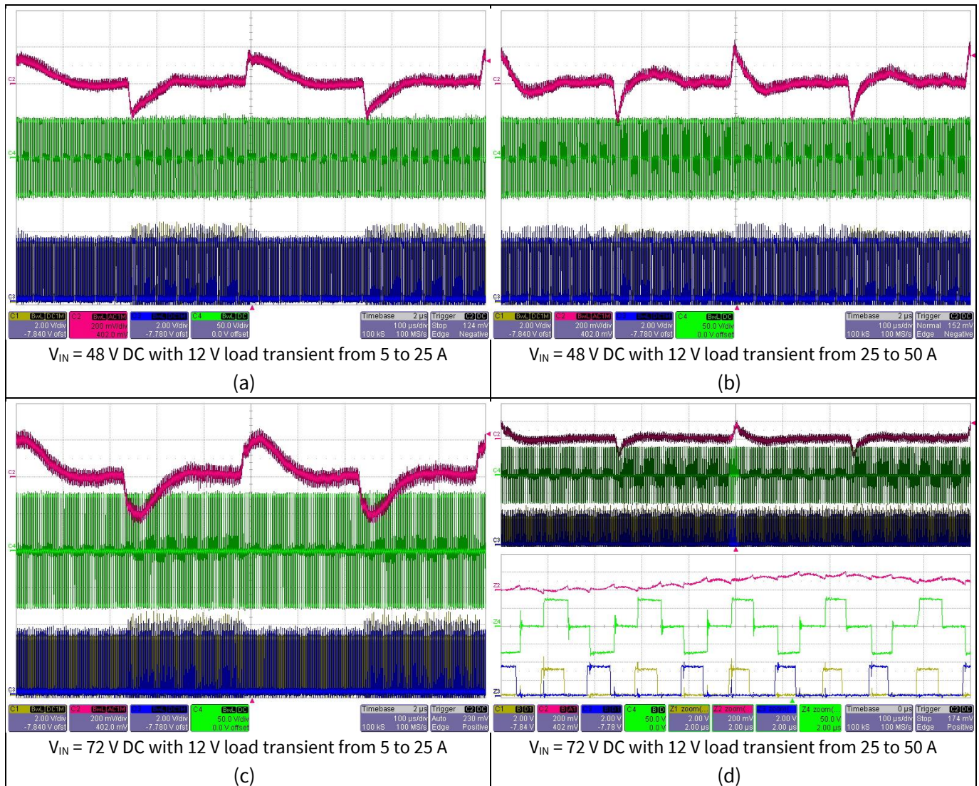
Figure 106 Output transient waveforms with flux balance enabled
