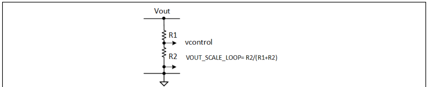
Figure 23 VOUT_SCALE_LOOP definition
