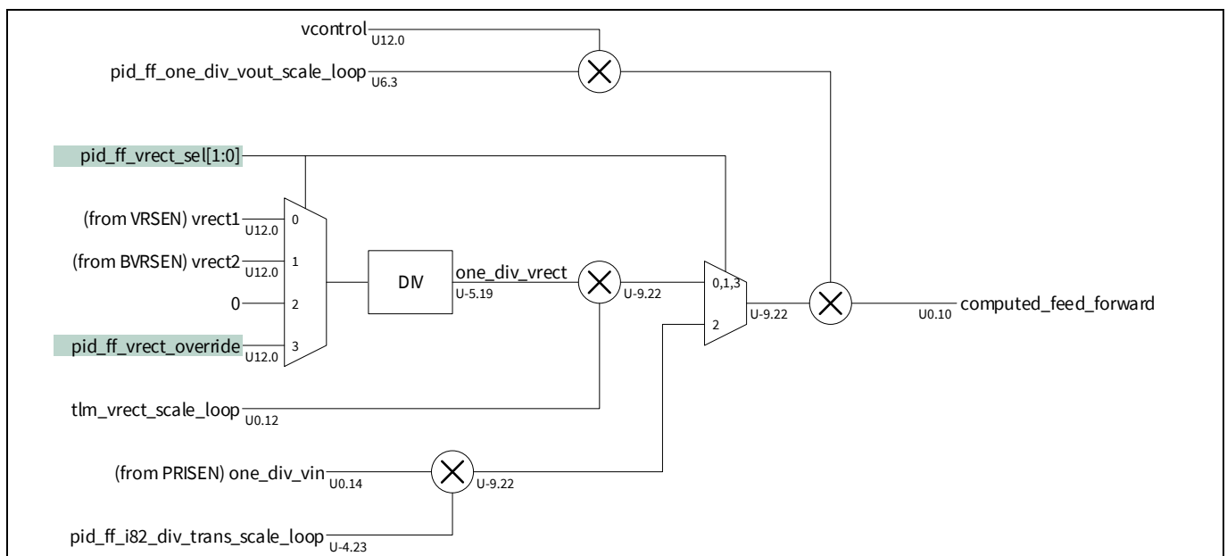
Figure 22 XDPP1100 feed-forward computation
