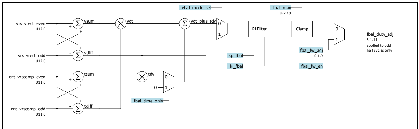
Figure 95 XDPP1100 flux balancing block diagram
