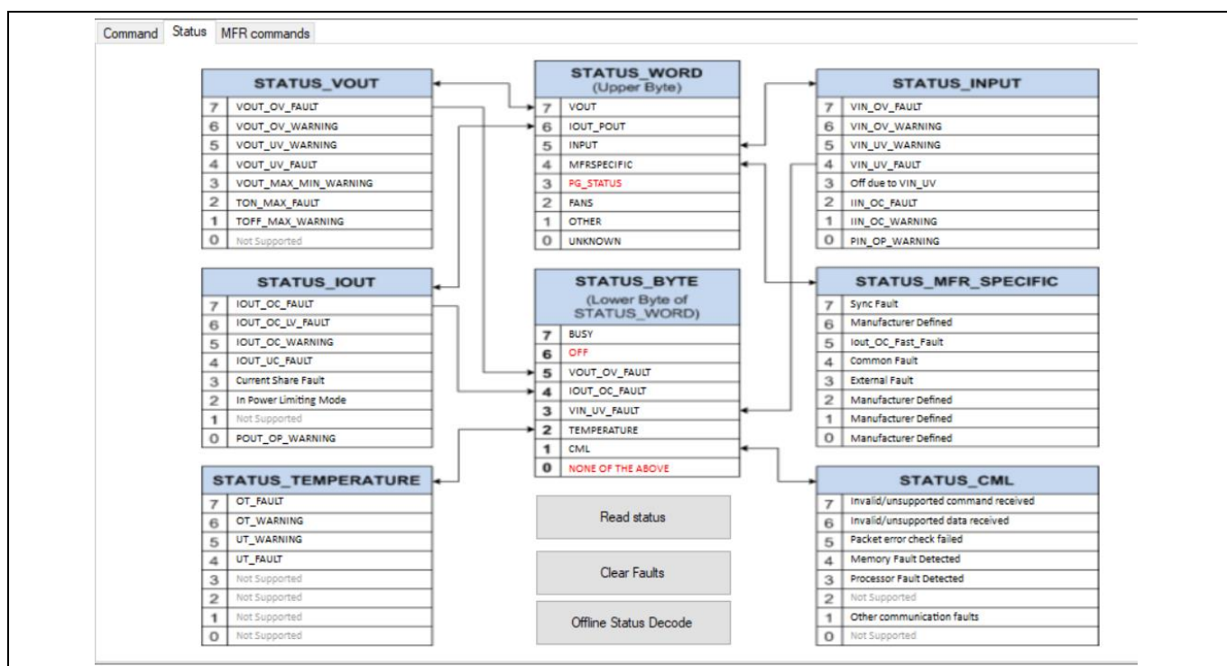
Figure 177 GUI status report
