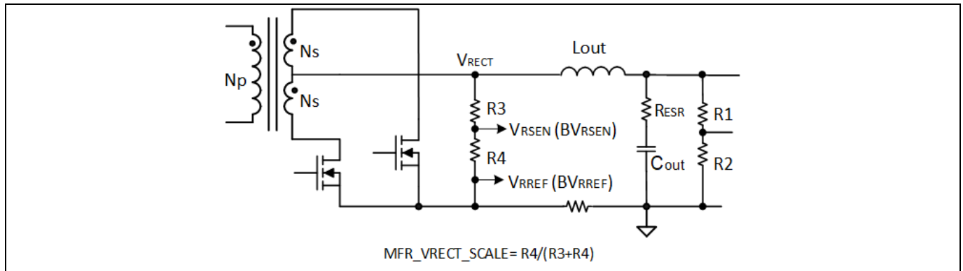
Figure 24 MFR_VRECT_SCALE definition
