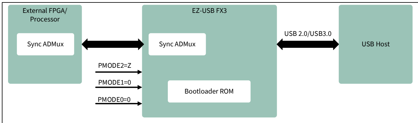
Figure 7 System diagram for synchronous ADMux boot
