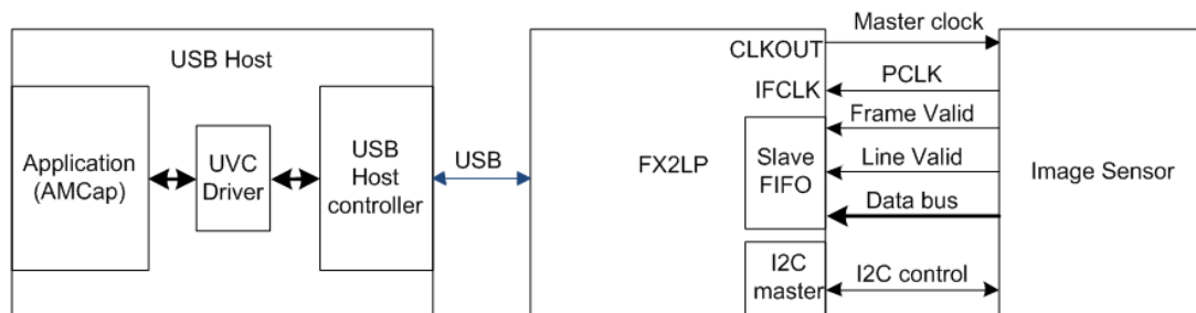
Figure 8. UVC Camera Design Using FX2LP
