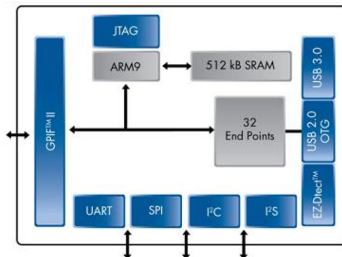
Figure 2. FX3 Block Diagram
