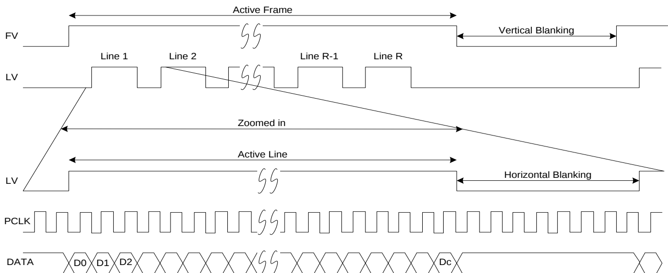
Figure 6. Image Sensor Interface Timing Diagram
