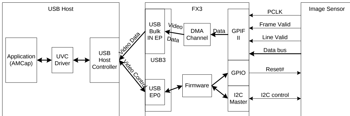
Figure 9. UVC Camera Implementation Using FX3
