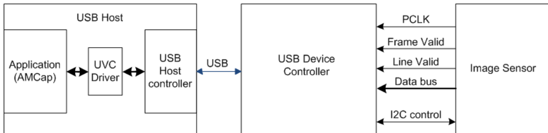
Figure 7. USB Camera Block Diagram
