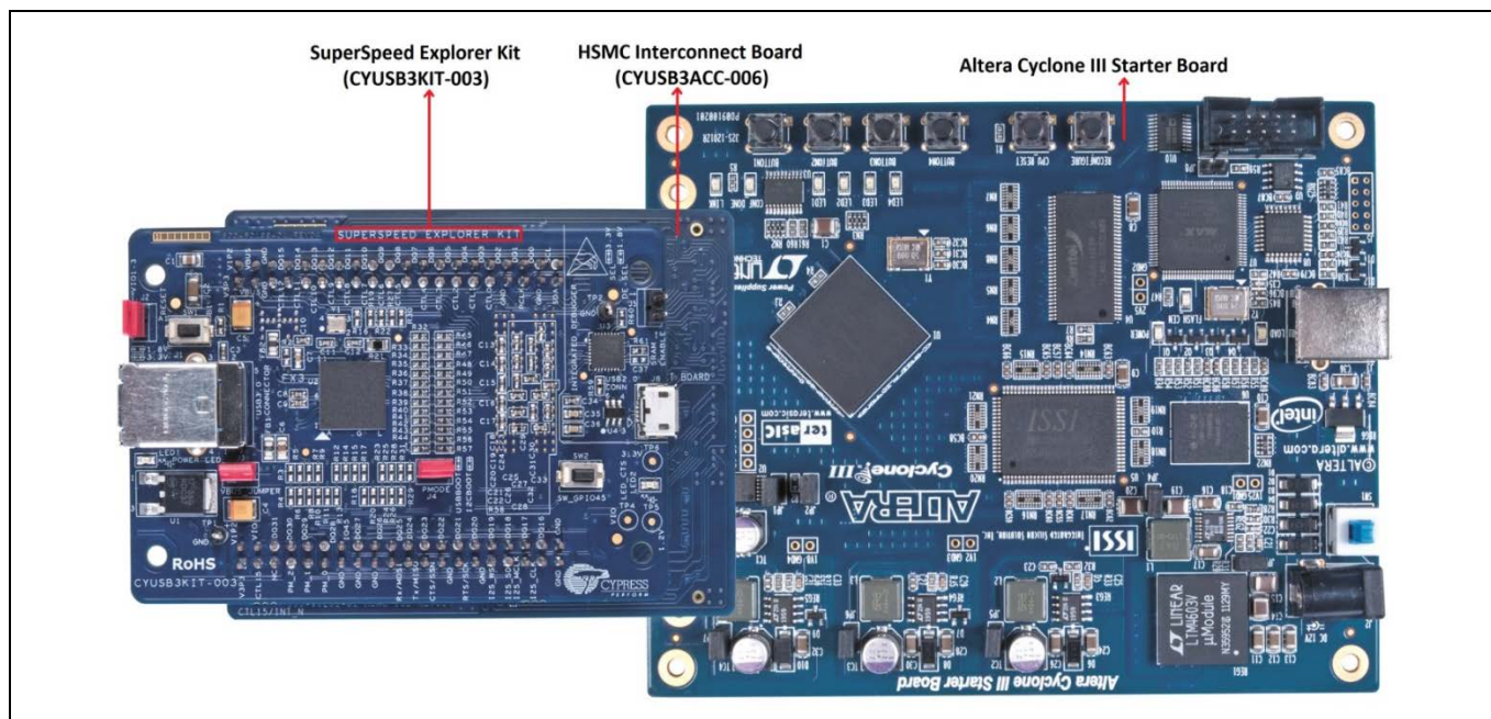
Figure 38 英飞凌 SuperSpeed Explorer 套件通过 HSMC 互联电路板与 Altera Cyclone III 入门电路板相连
