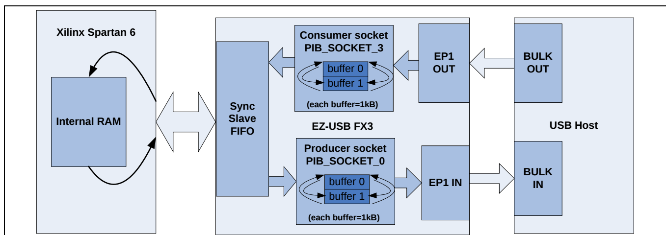
Figure 17 回送传输的设置
