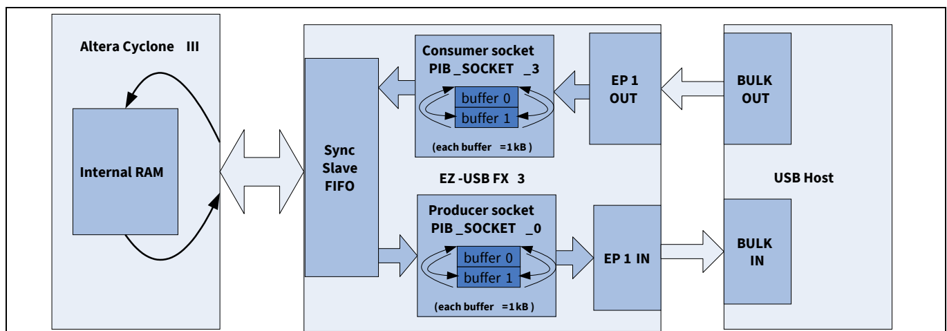
Figure 40 回送传输设置
