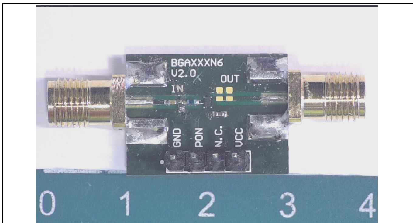
Figure 25 Evaluation board Option B (overview)
