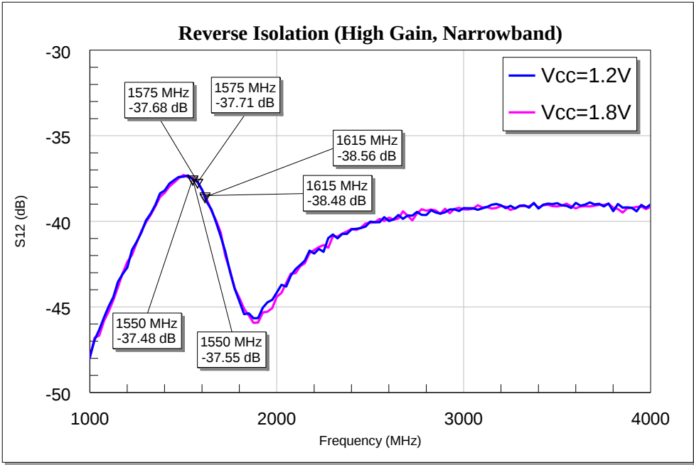
Figure 11 Reverse Isolation of BGA123L4 for GNSS Applications
