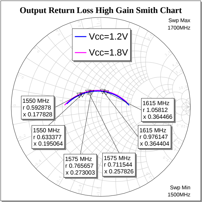
Figure 10 Output Return Loss (Smith Chart) of BGA123L4 for GNSS Applications
