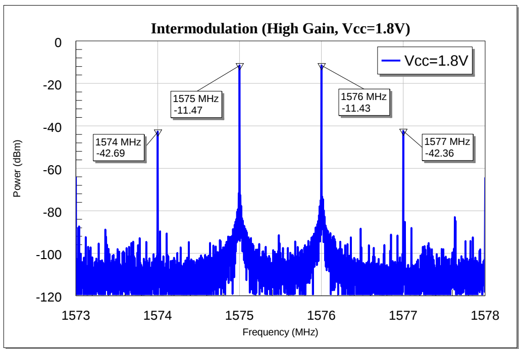
Figure 18 Third-order Interception Point (1.8V) of BGA123L4 for GNSS Applications (Output referred)
