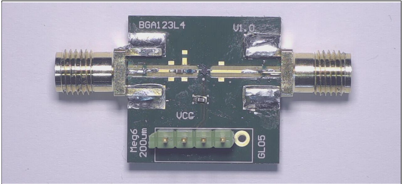
Figure 21 Photo Picture of Evaluation Board (overview)
