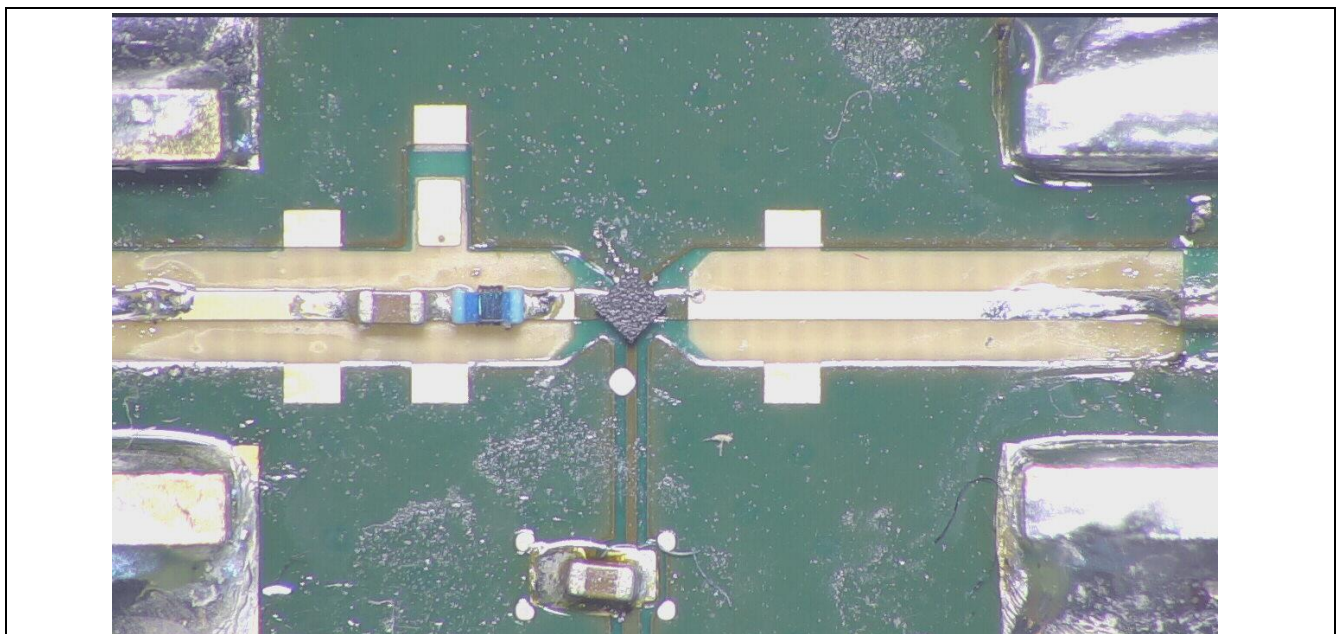
Figure 22 Photo Picture of Evaluation Board (detailed view)
