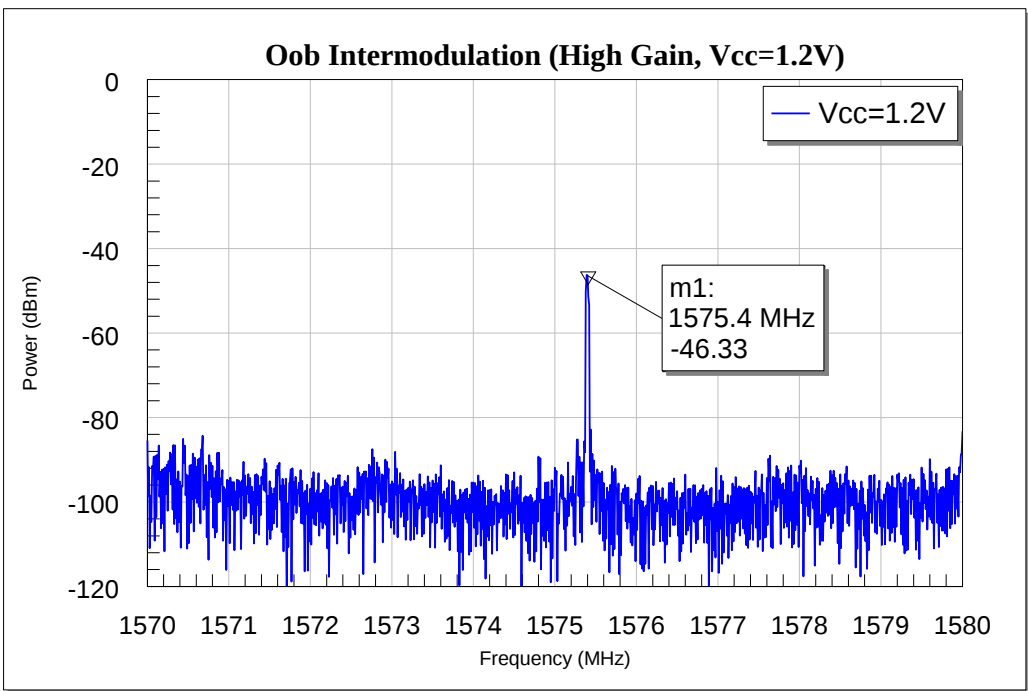
Figure 19 Out-of-band Third-order Intermodulation (1.2V) of BGA123L4 for GNSS Applications (Output referred)
