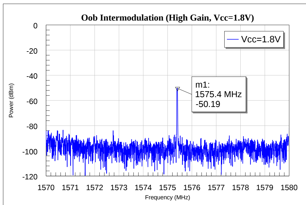
Figure 20 Out-of-band Third-order Intermodulation (1.8V) of BGA123L4 for GNSS Applications (Output referred)
