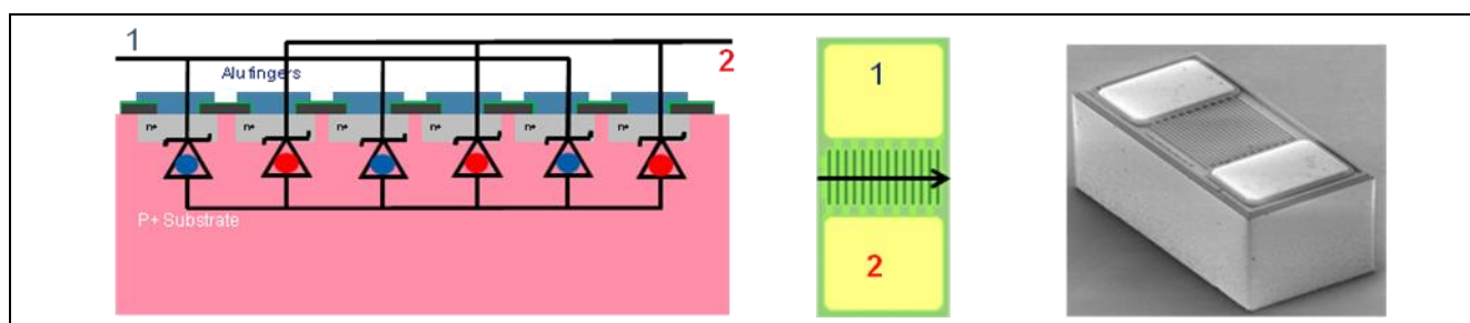
Figure 4 Internal structure of ESD200-B1-CSP0201 / ESD202-B1-CSP01005 (lateral ESD diode design)
