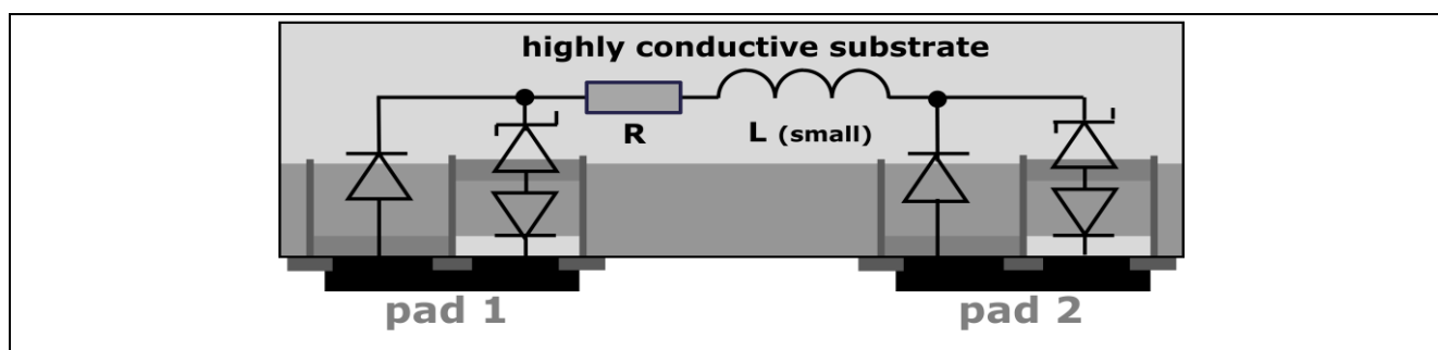
Figure 8 Internal structure of ESD108-B1-CSP0201 / ESD119-B1-W01005
