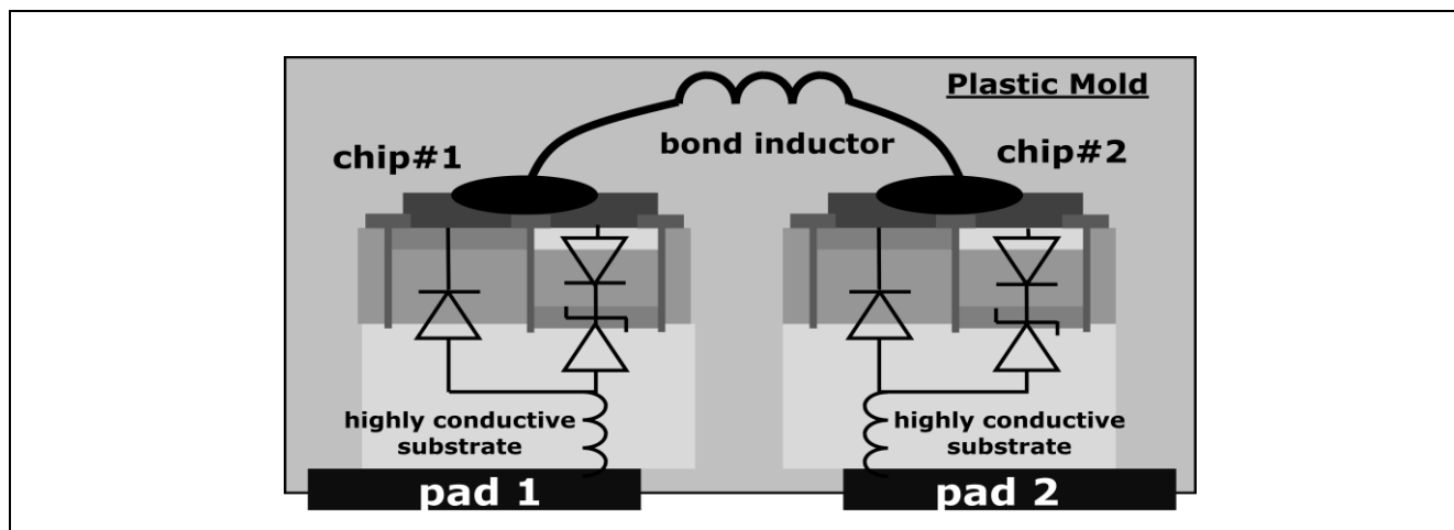
Figure 7 Internal structure of ESD112-B1-02Series
