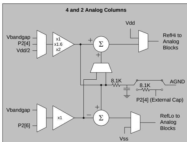
Figure 8. Analog Reference Generator
