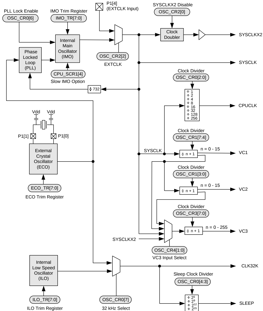
Figure 9. Comprehensive Diagram of PSoC Digital Clock System
