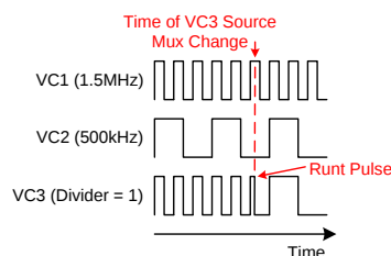
Figure 6. Glitches When Changing VC3 Source
