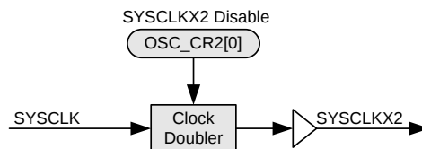
Figure 7. Sysclk*2 Clock Tree
