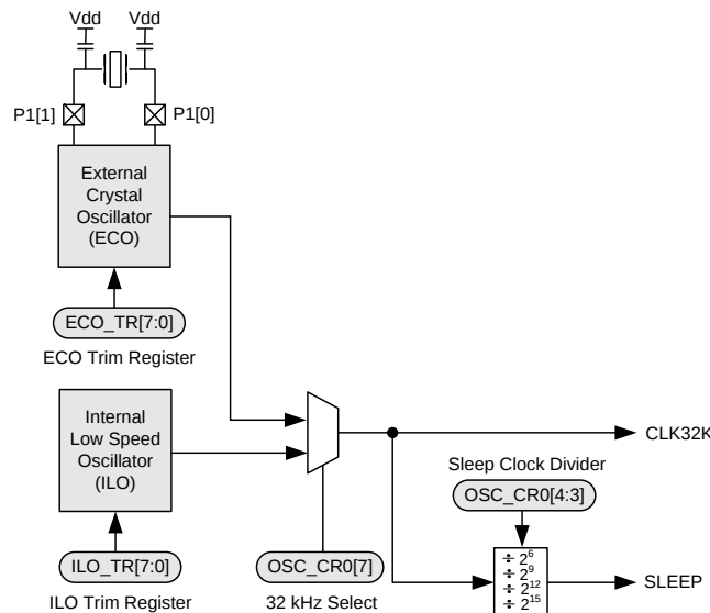
Figure 4. CLK32K and SLEEP Clocks
