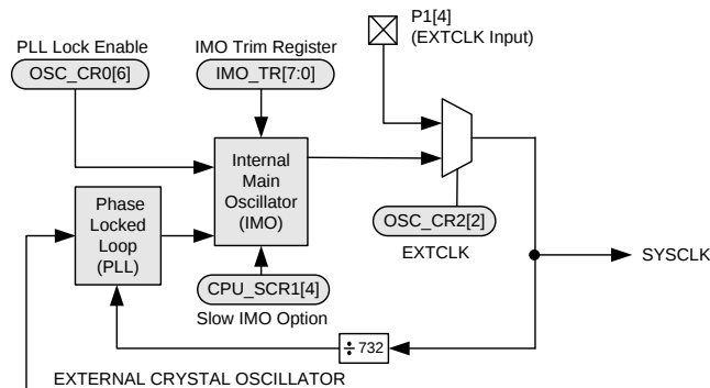
Figure 2. SysClk Clock Tree
