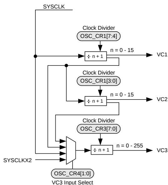
Figure 5. VC1, VC2, VC3 Clock Tree
