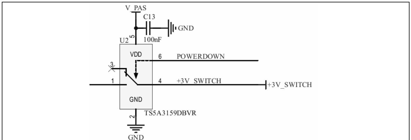
Figure 7 Switch for controlling the 3.3 V supply
