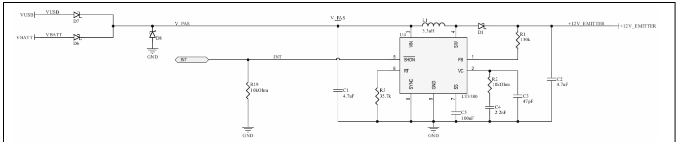
Figure 6 Schematic of the power circuit for the IR emitter
