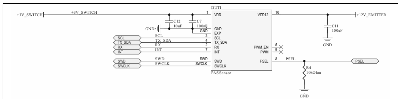
Figure 10 XENSIV™ PASCO2V01 sensor
