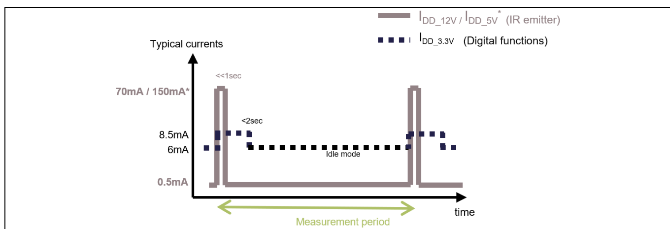
Figure 3 Principle of the current consumption
