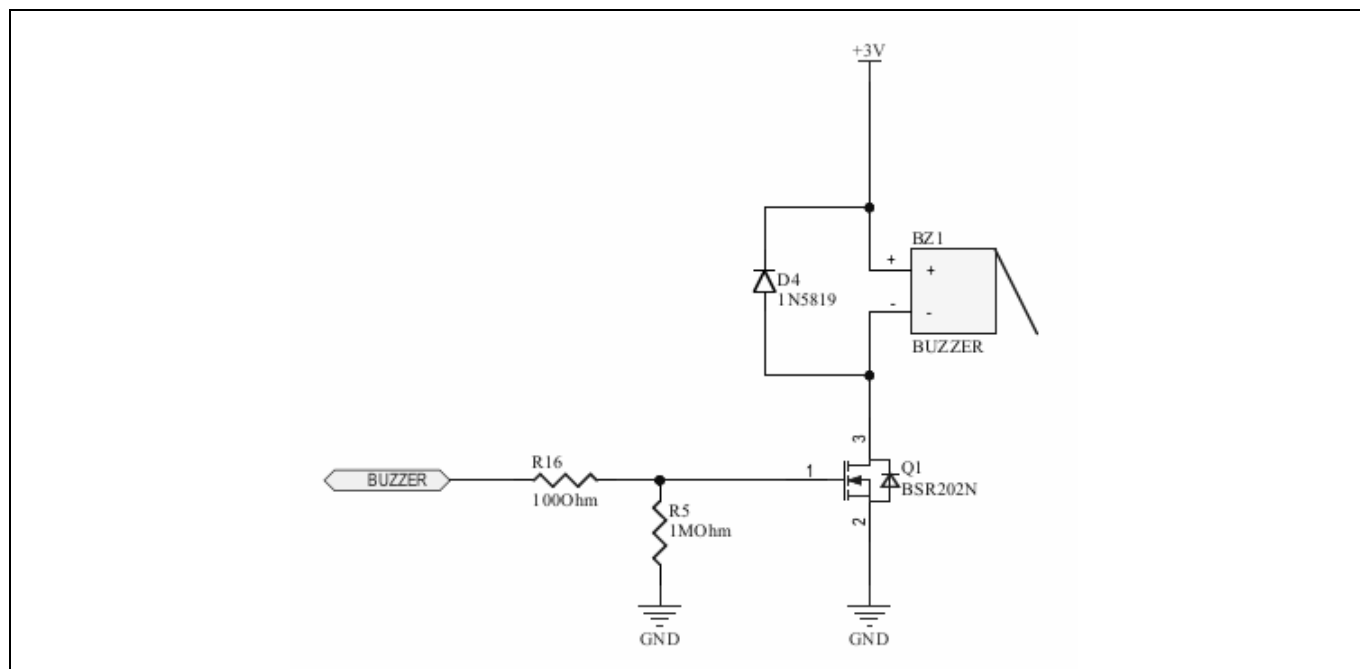
Figure 12 Buzzer circuit
