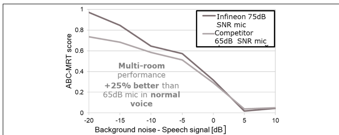
Figure 8 ABC-MRT score for cross-room scenario
