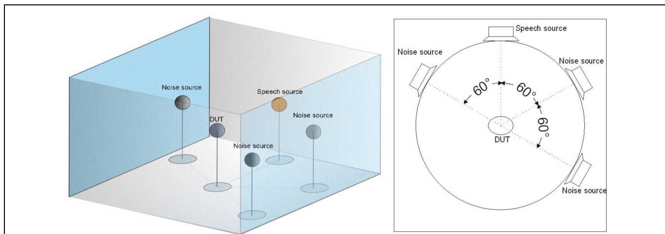
Figure 6 Test environment
