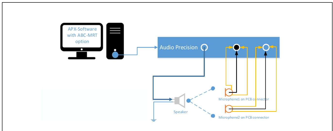
Figure 5 Overview of audio precision interface
