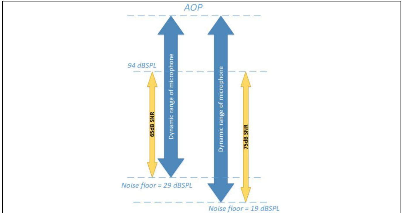
Figure 3 Relation between SNR and self-noise (noise floor) of the microphone
