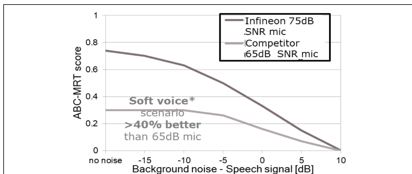
Figure 7 ABC-MRT score for whisper/soft-voice scenario
