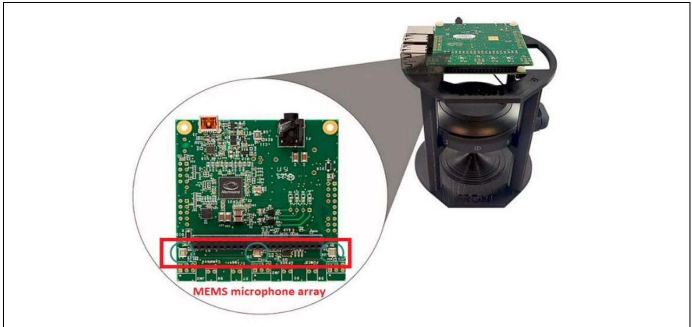
Figure 1 Interior of a smart speaker with a linear microphone array
