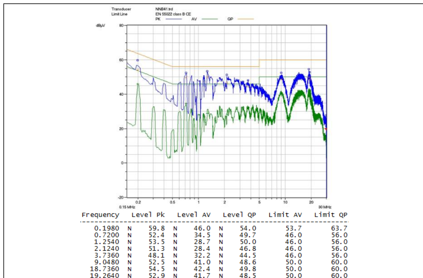
Figure 16 Conducted emissions (neutral) at 230 V AC and maximum load
