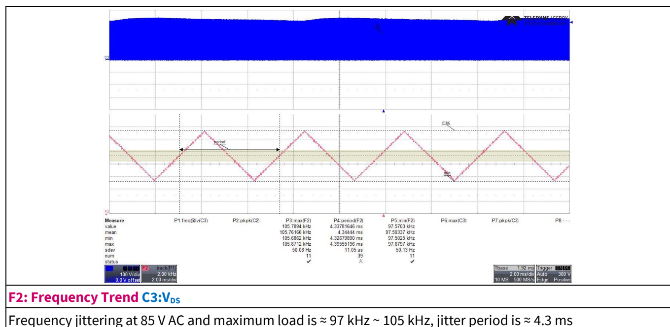
Figure 21 Frequency jittering
