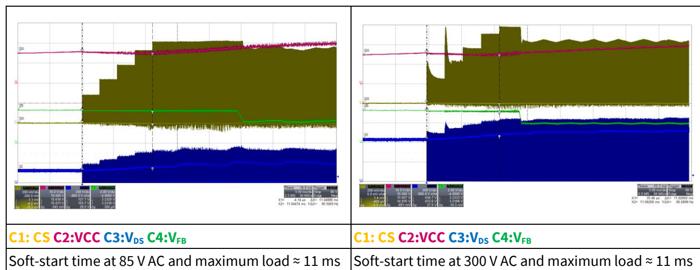
Figure 19 Soft-start
