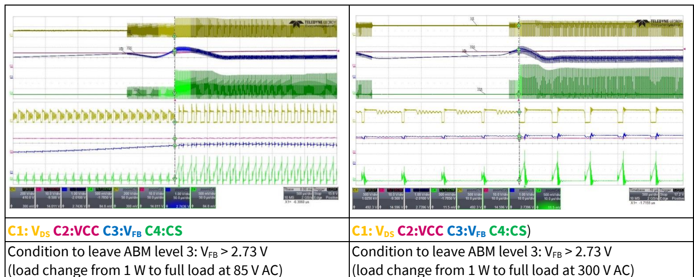
Figure 27 Leaving ABM
