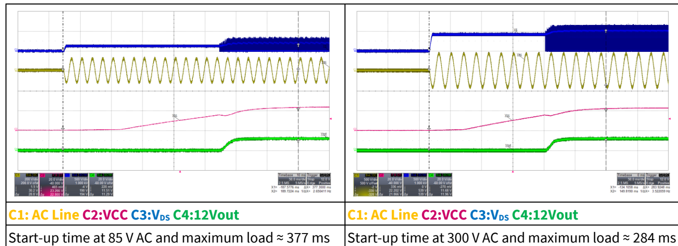
Figure 18 Start-up
