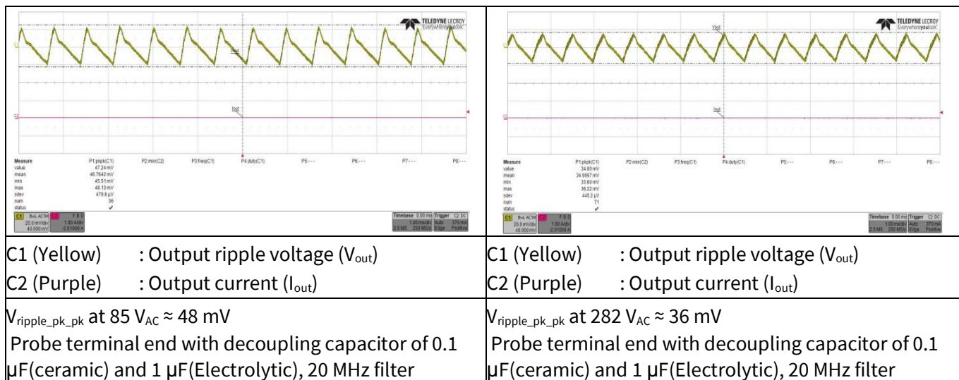
Figure 24 Output ripple voltage at burst mode 1 W load
