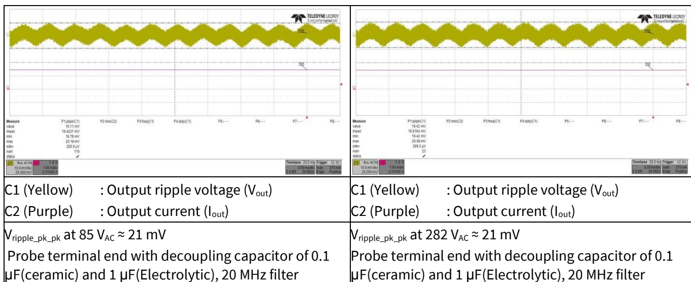
Figure 23 Output ripple voltage at maximum load
