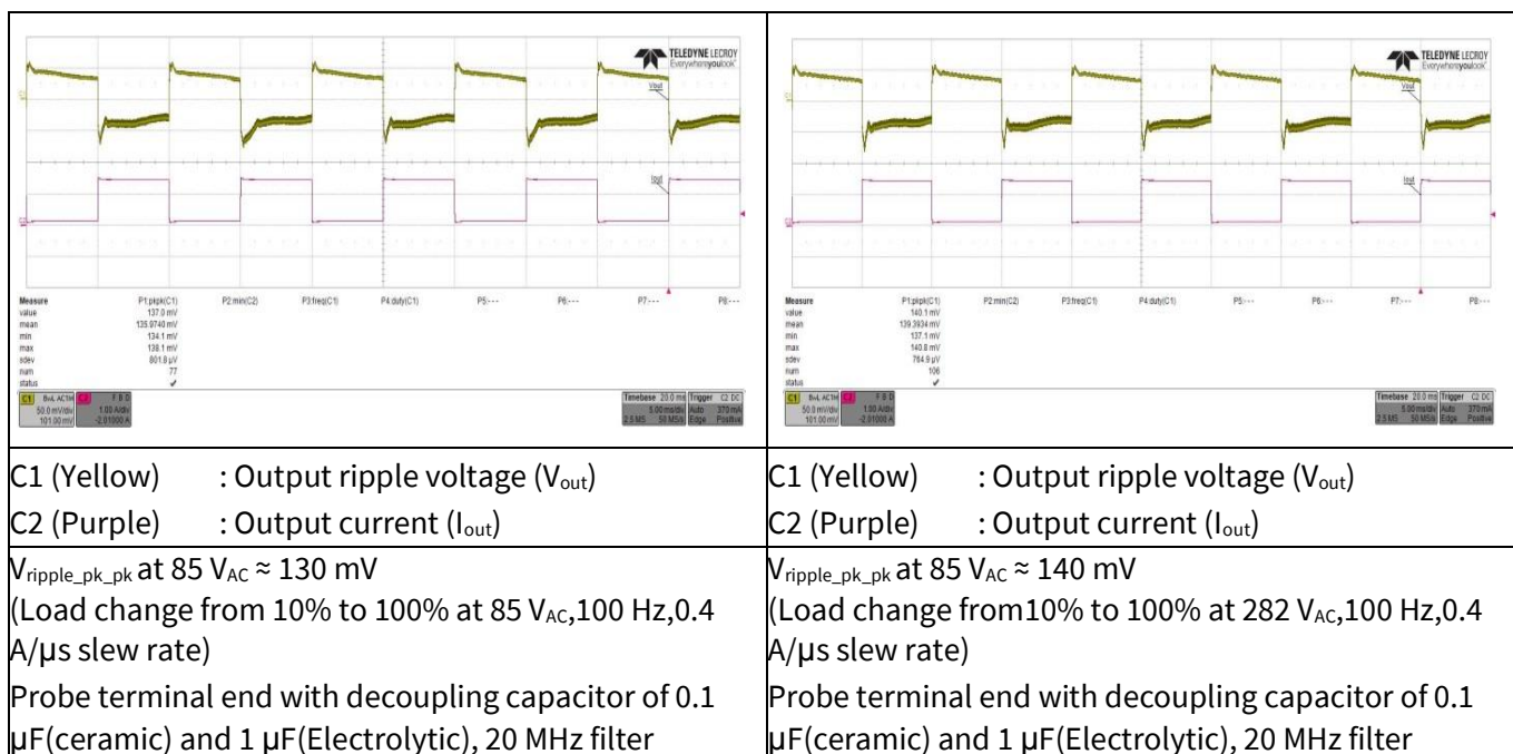
Figure 22 Load transient response
