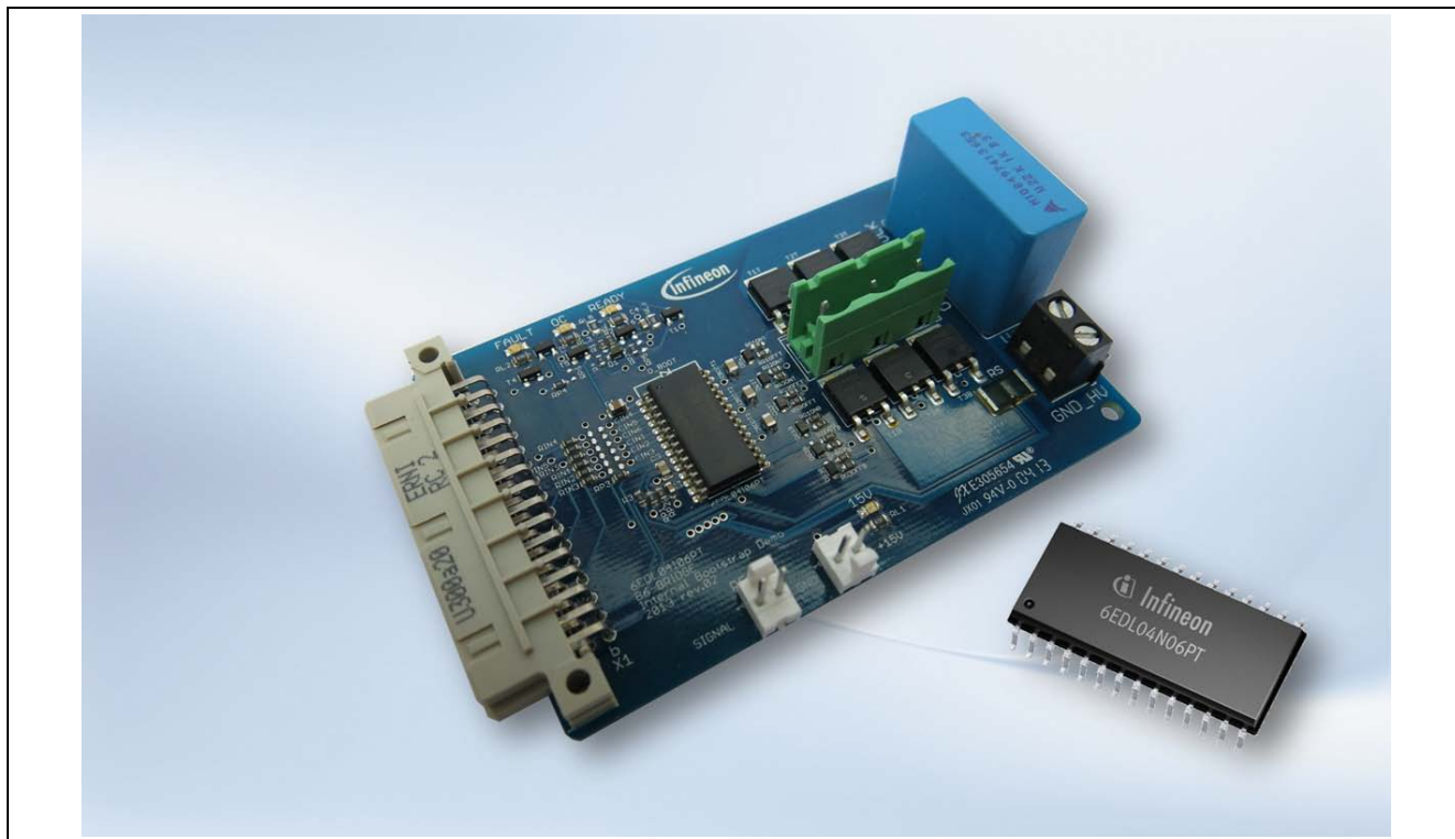
图1 EVAL-6EDL04I06PT 俯视图
