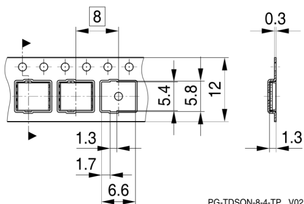
PG-TDSON-8-4-TP V02
