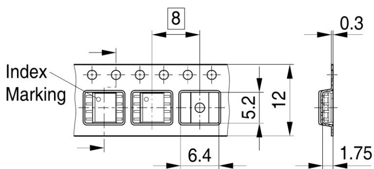
PG-DSO-8-16, -24, -25, -28, -31, -33, -36, -44, -49-TP V09
