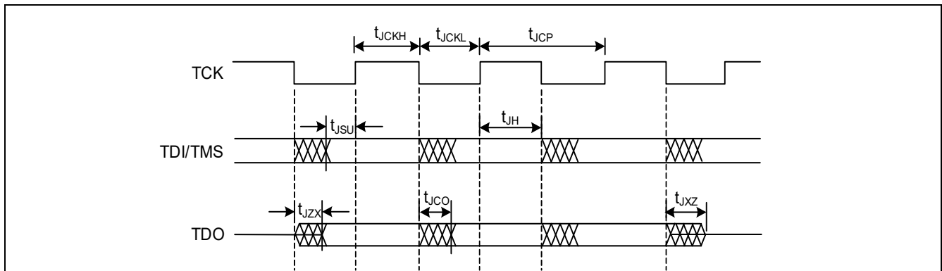
Figure 26-21 JTAG specifications
