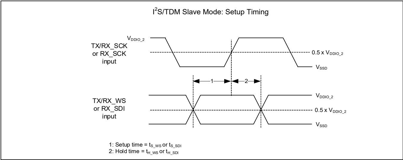
Figure 26-42 Slave setup
