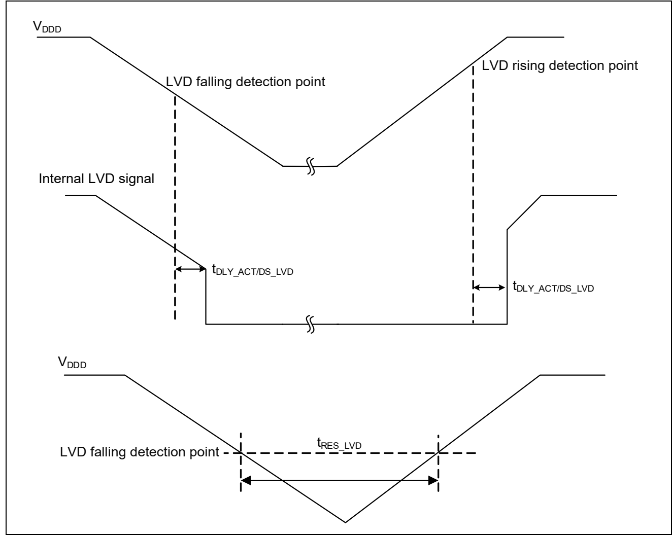
Figure 26-20 LVD specifications
