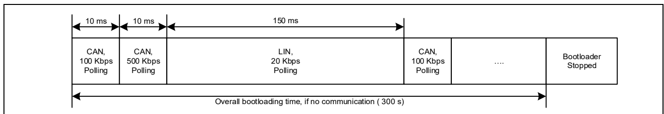
Figure 29-1 Bootloading sequence
