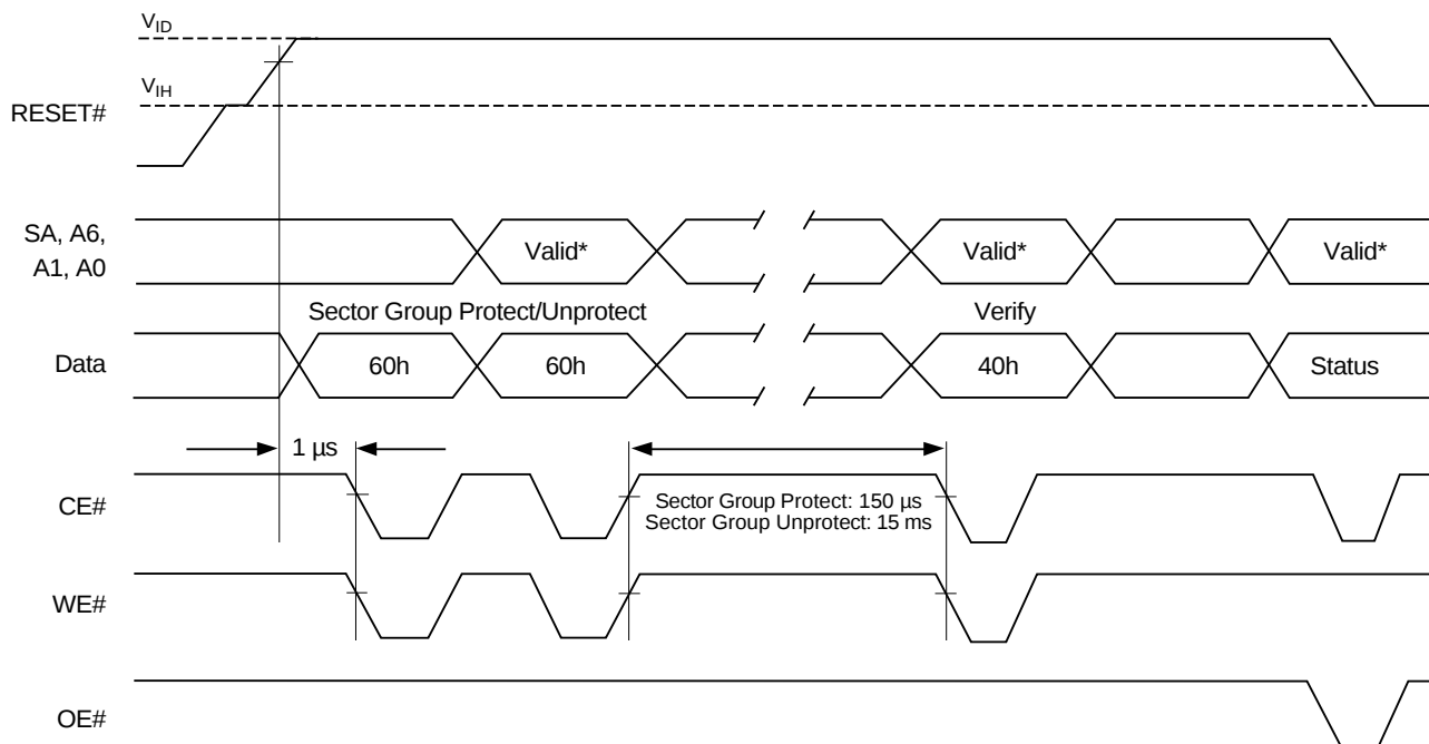
Figure 17.4 Sector/Sector Block Protect and Unprotect Timing Diagram [61]
