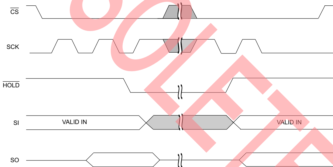
Figure 14. \overline{HOLD} Operation [2]
