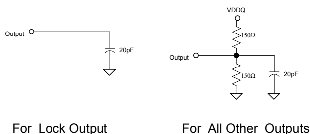
Figure 2. For Lock Output and all other Outputs
