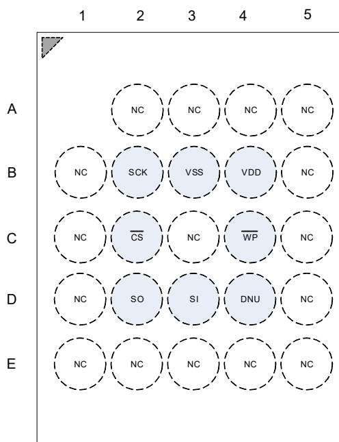
Figure 1. 24-ball FBGA Pinout
