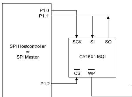
Figure 3. System Configuration without SPI Port
