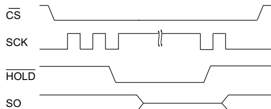
Figure 19. \overline{\text{HOLD}} Operation
