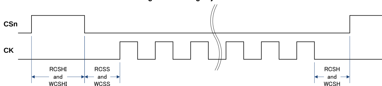
Figure 3-4 Timing Adjustment
