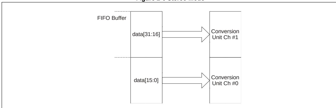
Figure 2-6 Stereo Mode
