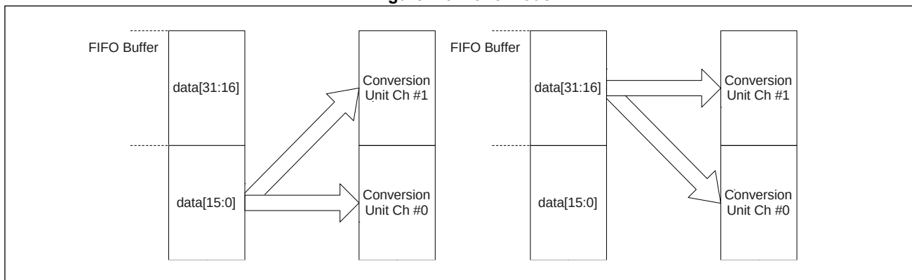
Figure 2-5 Mono Mode
