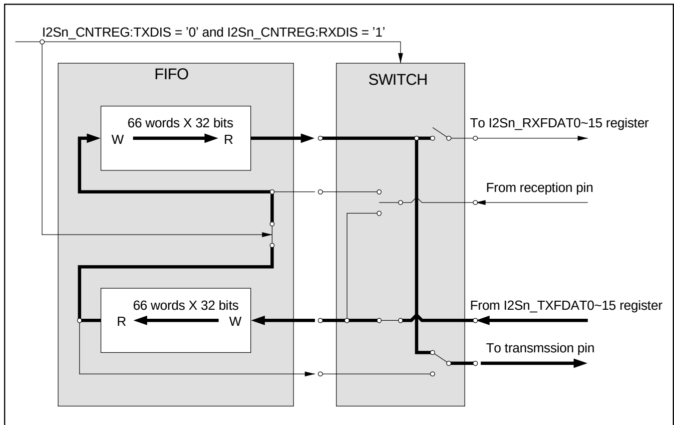
Figure 3-6 Transmission Only Mode Data Flow
