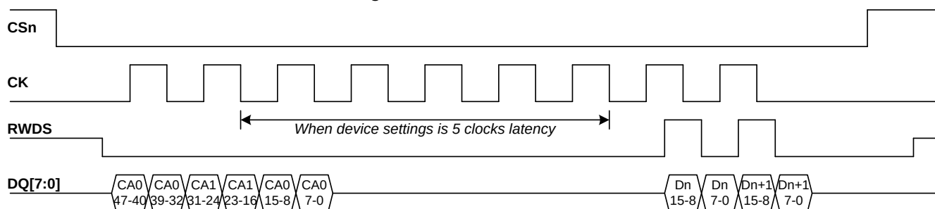
Figure 3-1 Read Waveform
