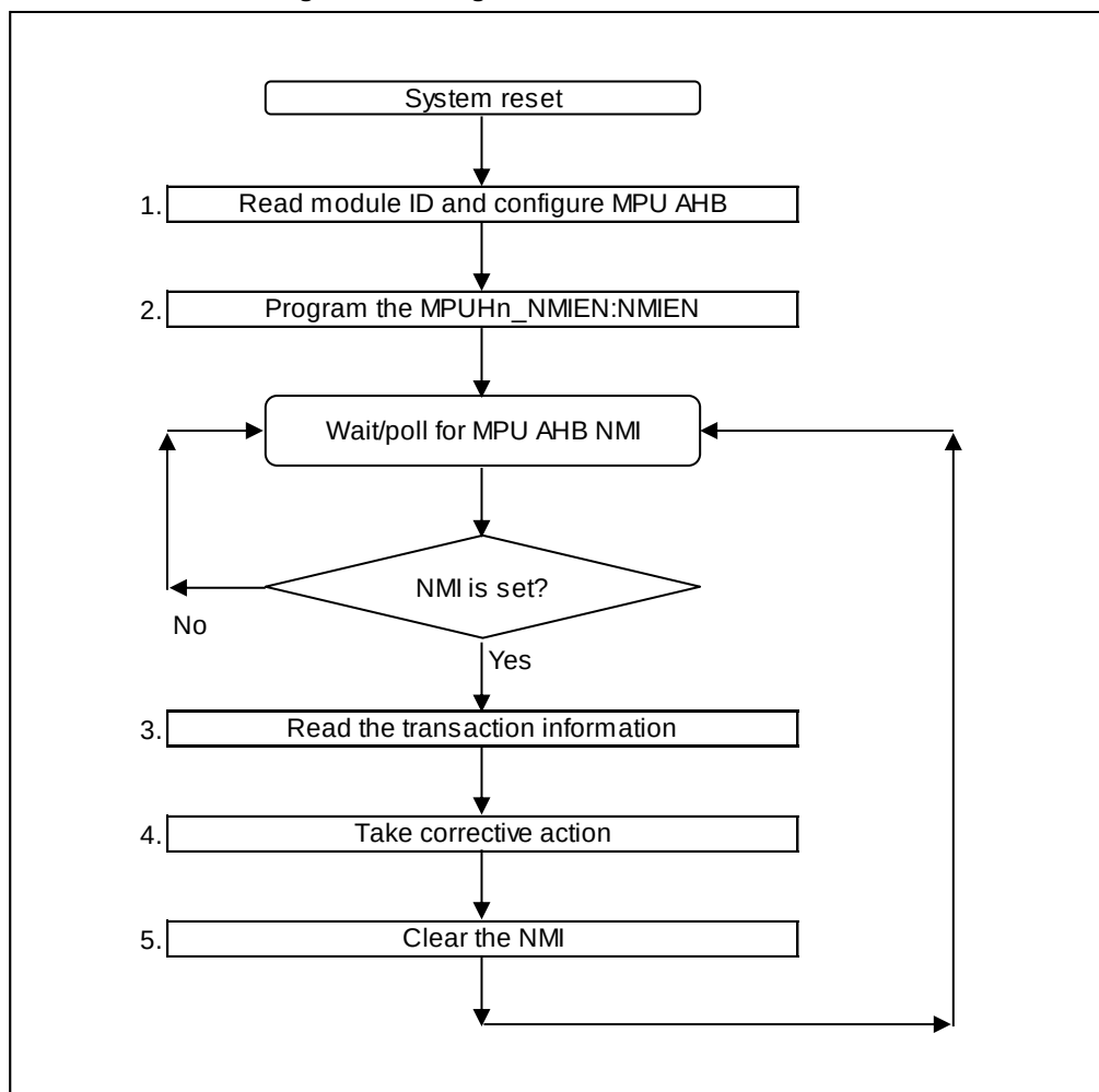
Figure 5-1 Programmer's Flowchart
