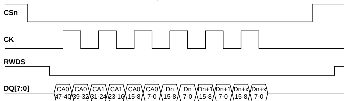
Figure 3-2 Write Waveform
