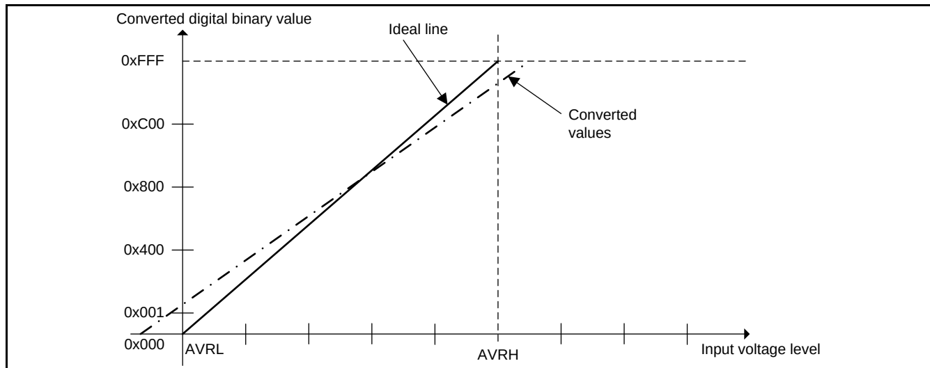
Figure 3-12 Example of Converted Digital Value Dependence on Input Voltage Level
