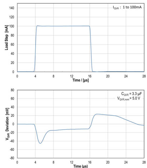
QVR Dynamic Load Response (1mA to 100mA) ( V_{QVR,nom} = 5.0 \text{ V} )
