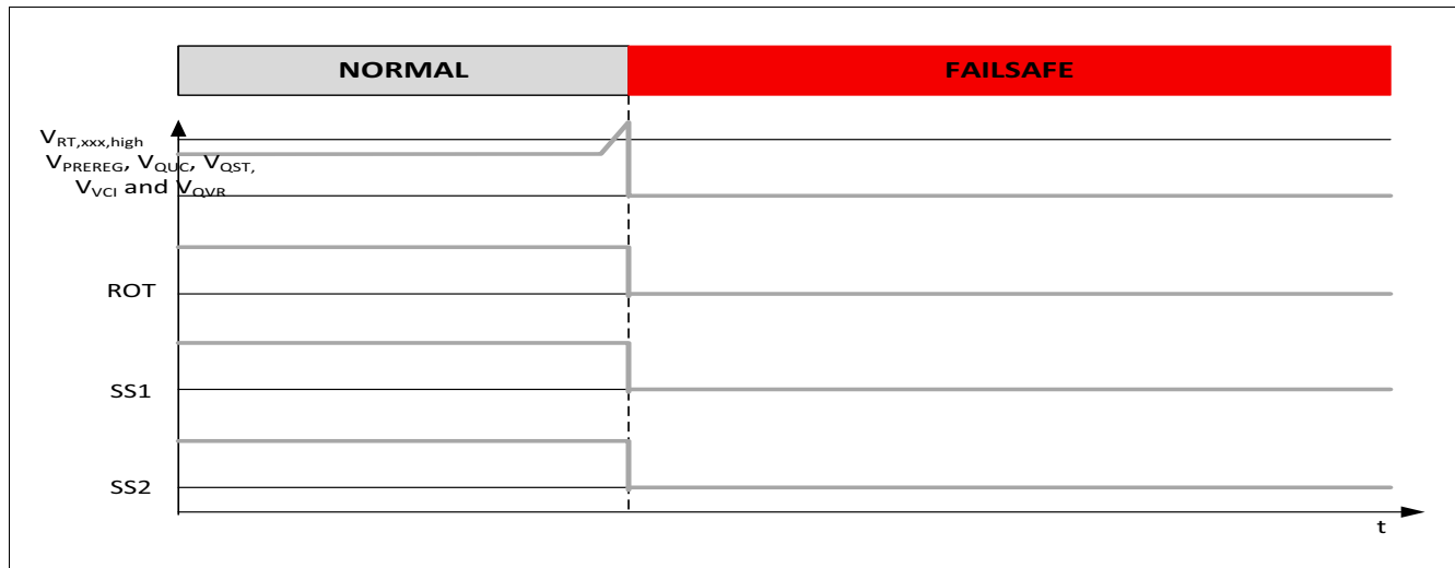
Figure 52 Transition from NORMAL to FAILSAFE state
