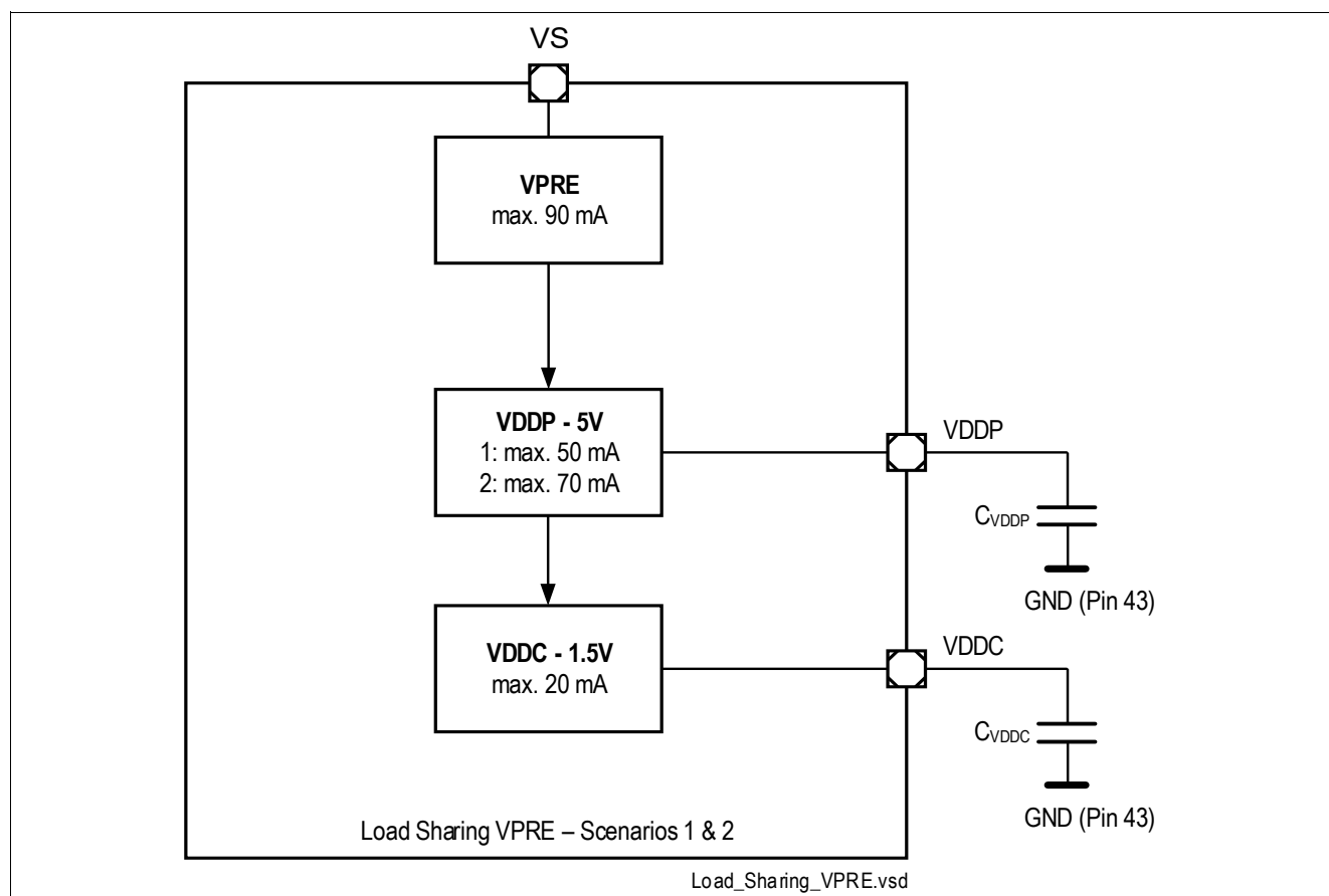
Figure 41 Load Sharing Scenario of VPRES and VDDP Regulator
