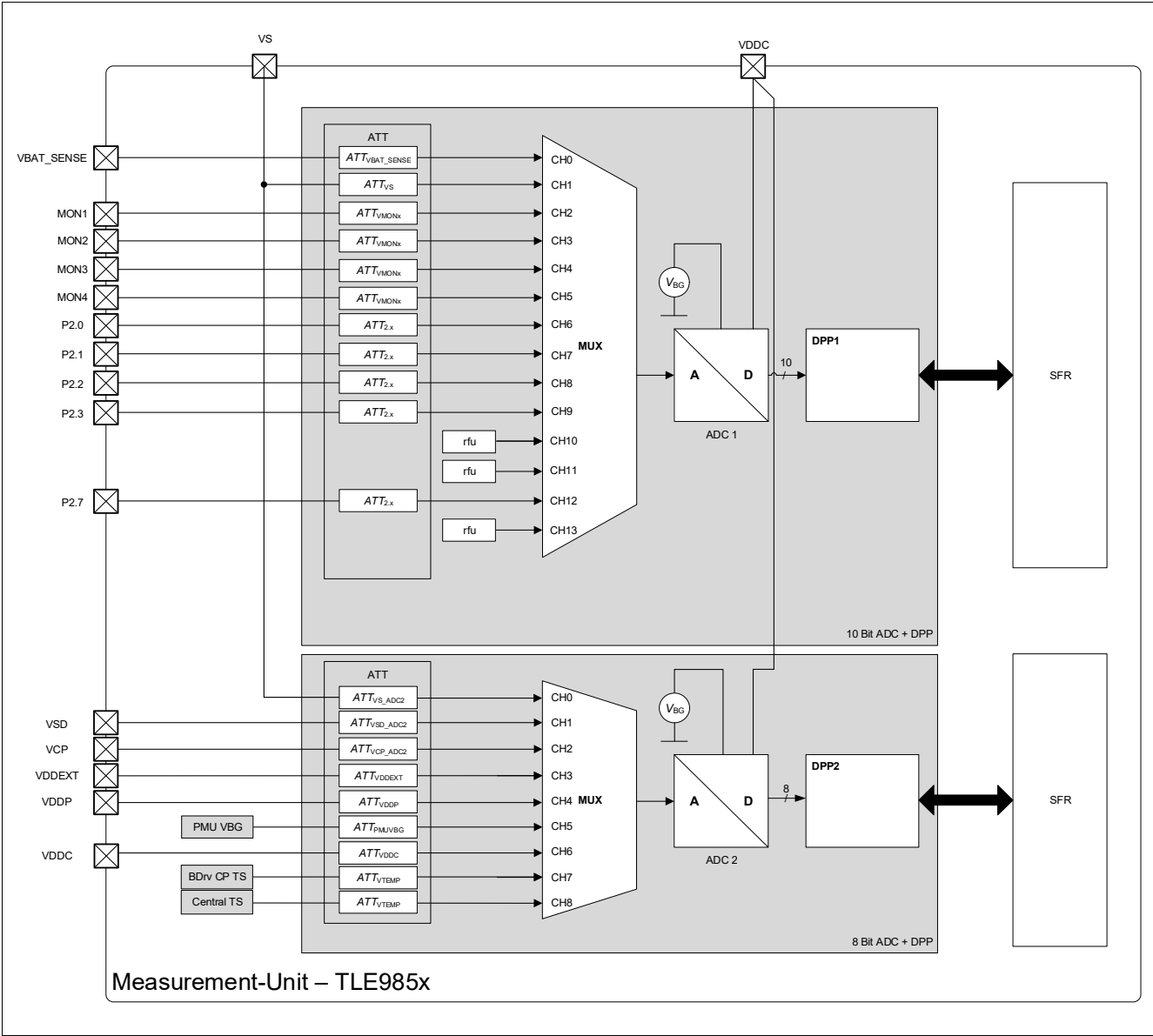
Figure 27 Measurement Unit-Overview
