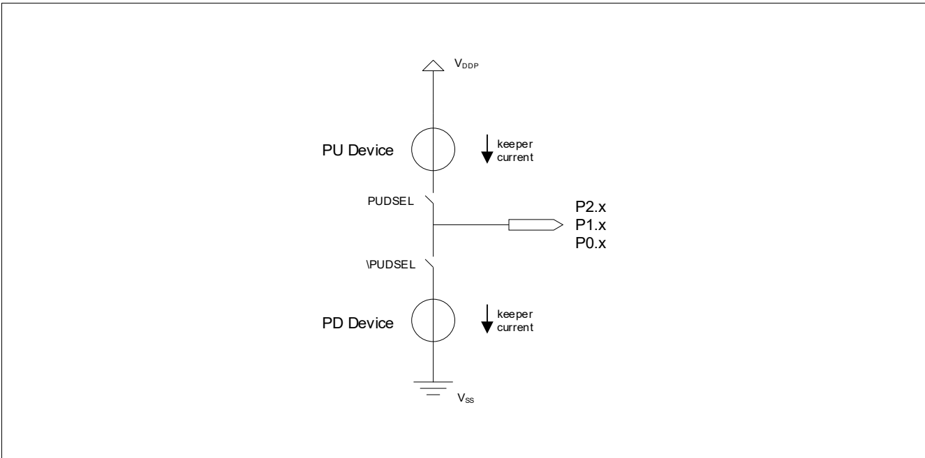
Figure 42 Pull-Up/Down Device
