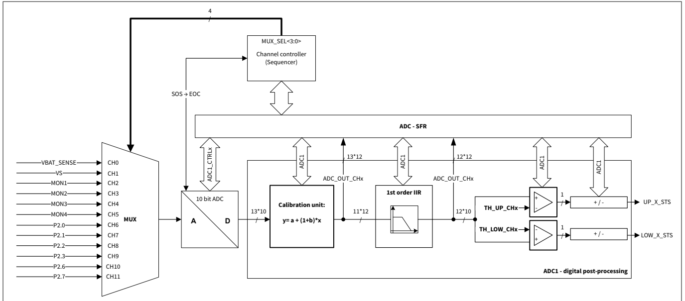
Figure 32 Module block diagram
