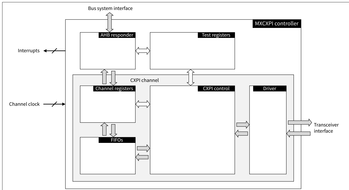
Figure 28 MXCXPI block diagram
