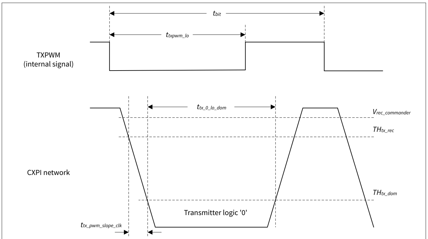
Figure 49 Waveforms for logic value '0'
