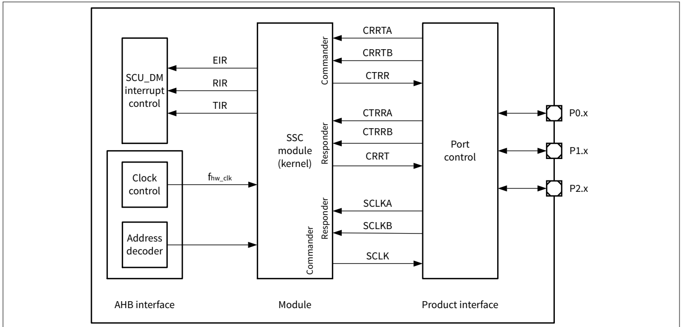
Figure 29 SSC interface diagram
