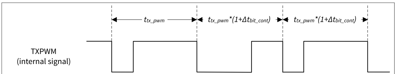
Figure 57 TXPWM falling edge transmitter jitter
