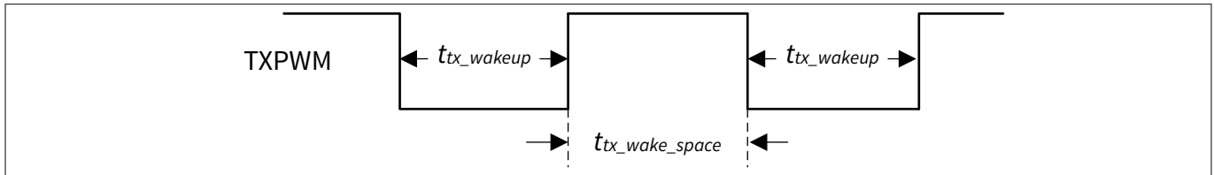
Figure 55 Wake-up pulse generated by responder node
