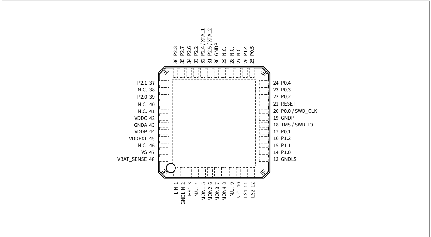
Figure 3 Device pinout, TLE9844QXC
