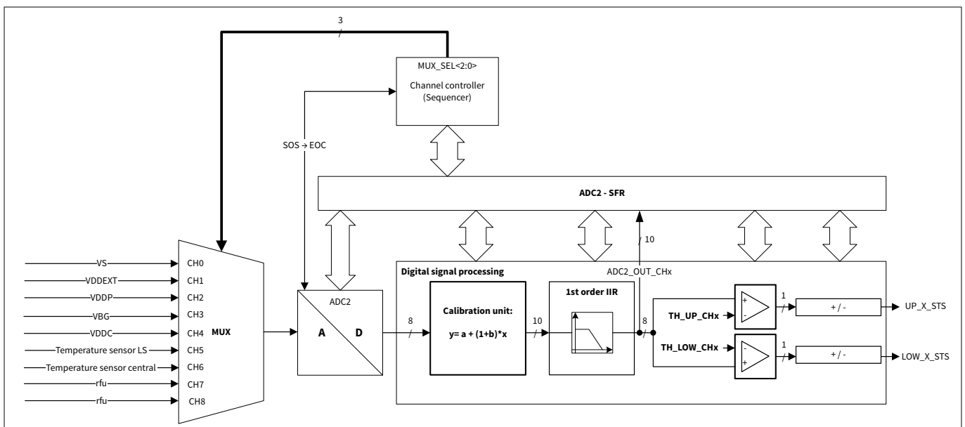
Figure 31 Module block diagram
