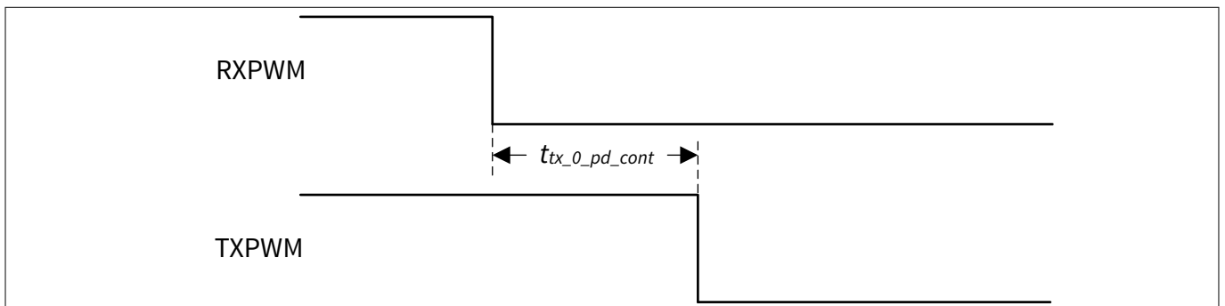
Figure 52 Transmitter propagation delay for logic value '0' (responder node)
