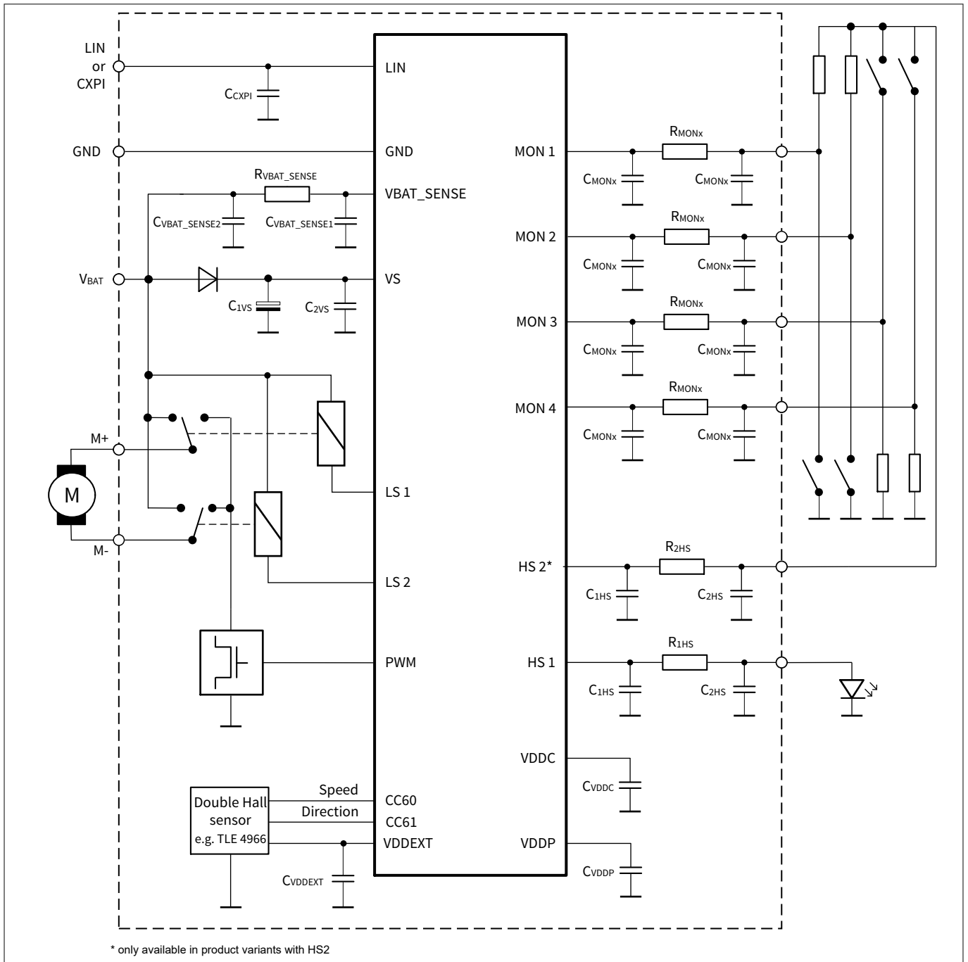
Figure 36 Simplified application diagram example
