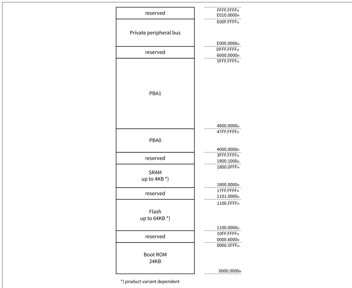
Figure 16 TLE9844QXC memory map
