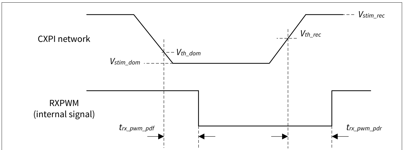
Figure 45 Receiver propagation delay
