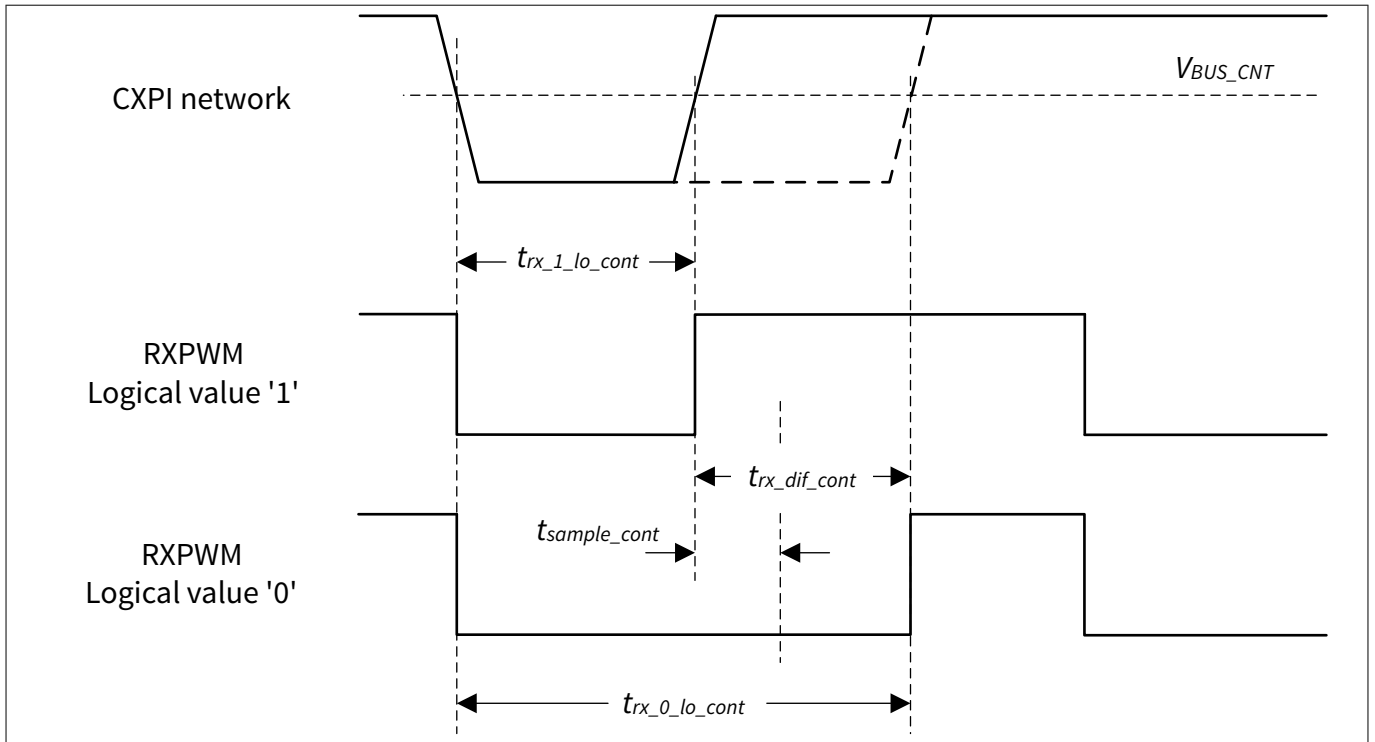
Figure 50 Width difference of LO levels
