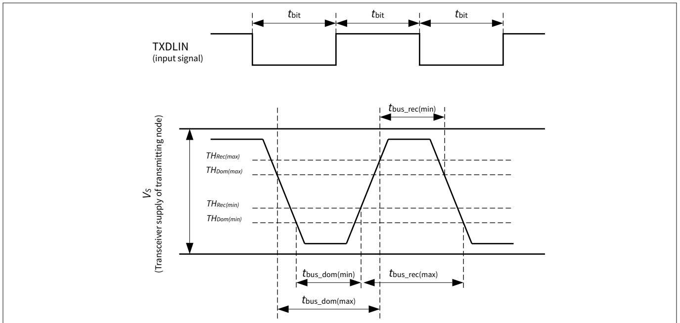
Figure 42 LIN network timing parameters
