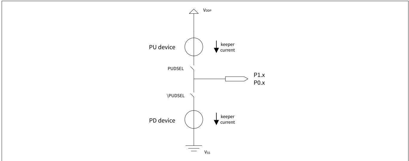
Figure 38 Pull-up/down device
