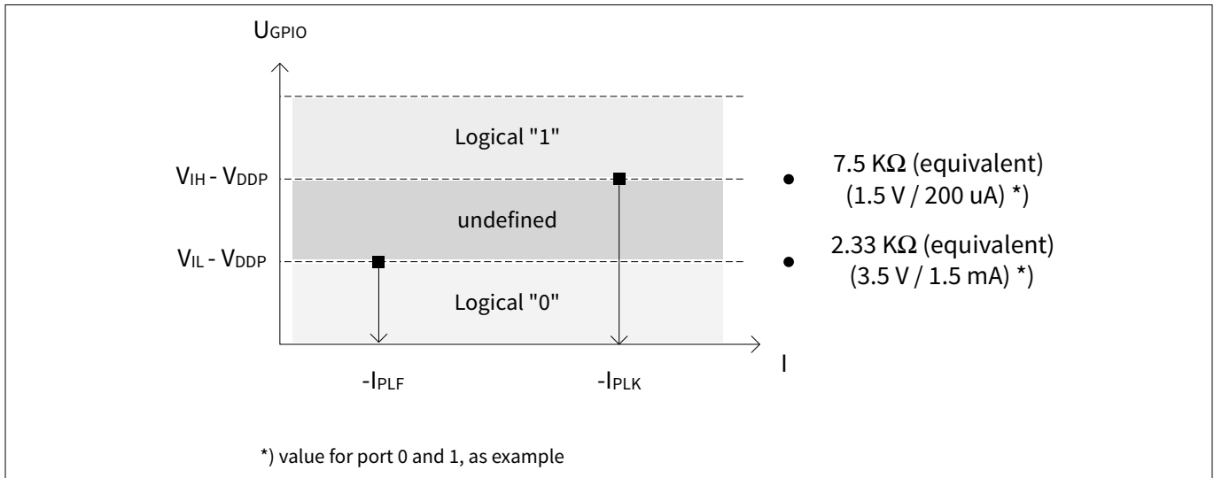
Figure 39 Pull-up keep and forced current
