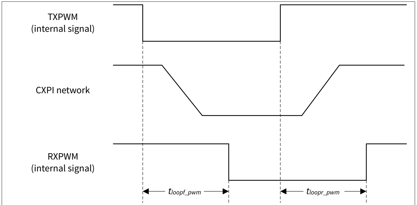
Figure 46 Loop delay
