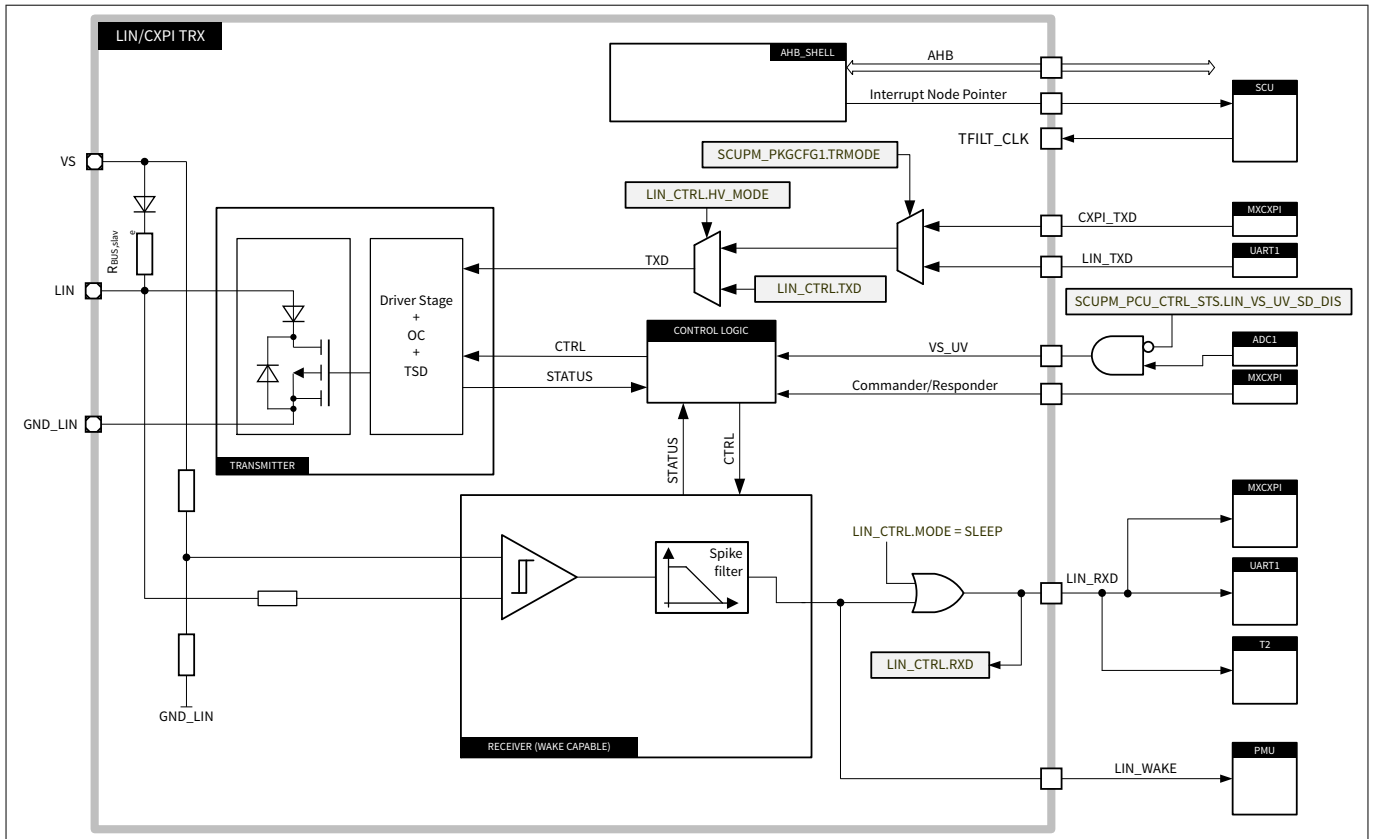
Figure 27 CXPI transceiver block diagram
