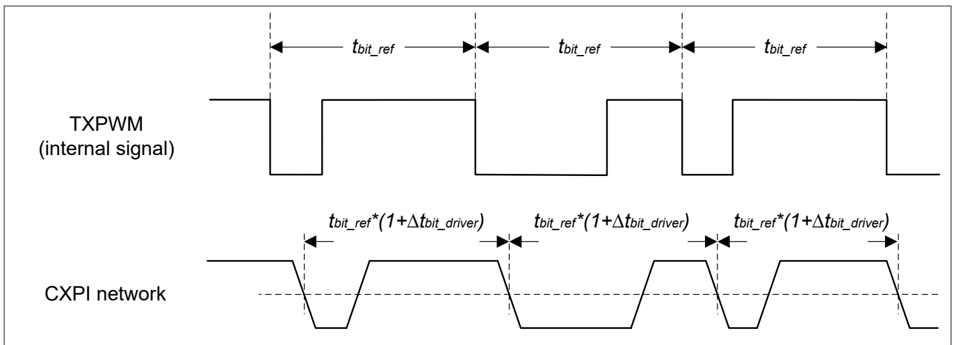
Figure 51 Network falling edge transmitter jitter
