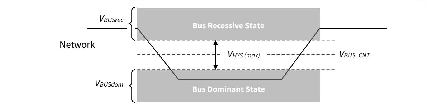
Figure 47 Definition of bus states
