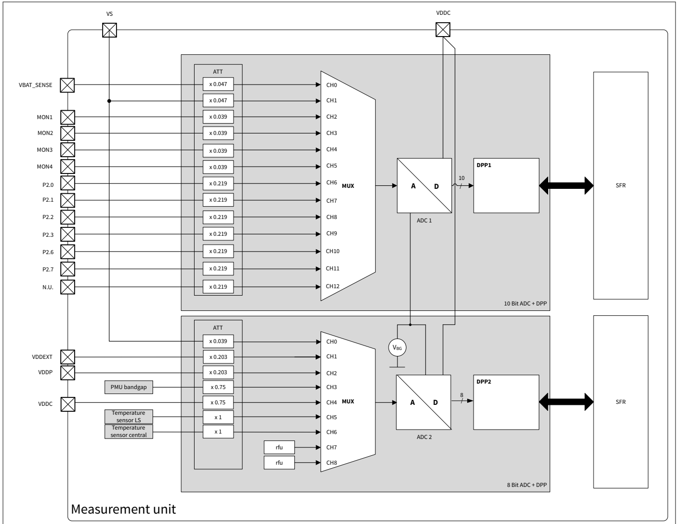
Figure 30 TLE9844QXC measurement unit overview
