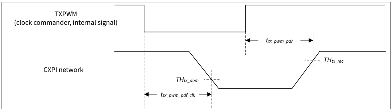
Figure 43 Transmitter propagation delay (clock commander)
