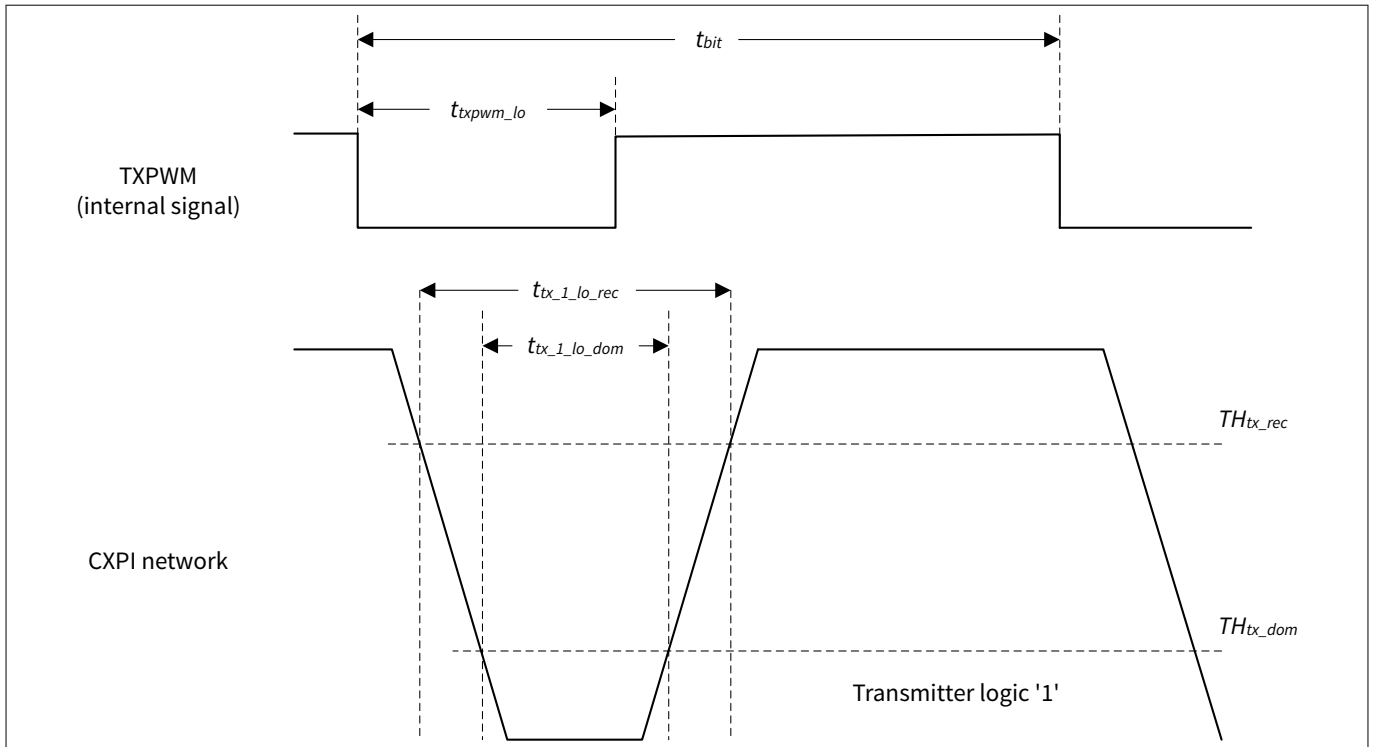
Figure 48 Waveforms for logic value '1'
