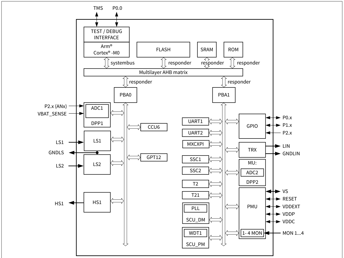
Figure 2 Block diagram, TLE9844QXC
