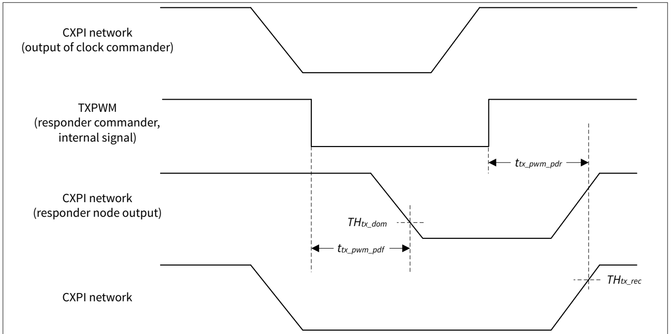
Figure 44 Transmitter propagation delay (responder node)
