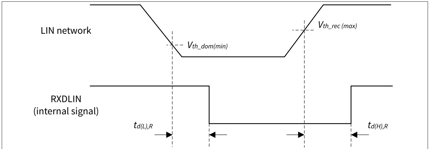
Figure 41 Receiver propagation delay
