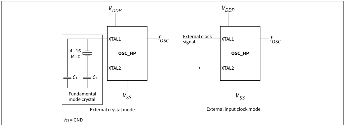
Figure 10 OSC_HP external circuit
