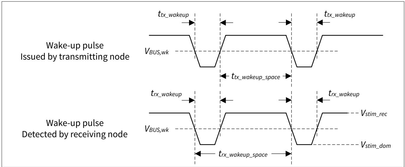
Figure 54 Network wake-up pulse waveforms
