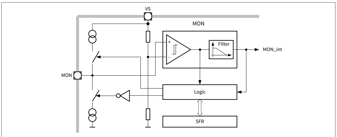
Figure 33 Monitoring input block diagram
