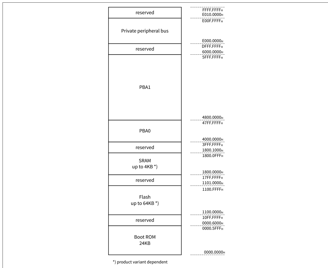
Figure 16 TLE9844-2QX memory map
