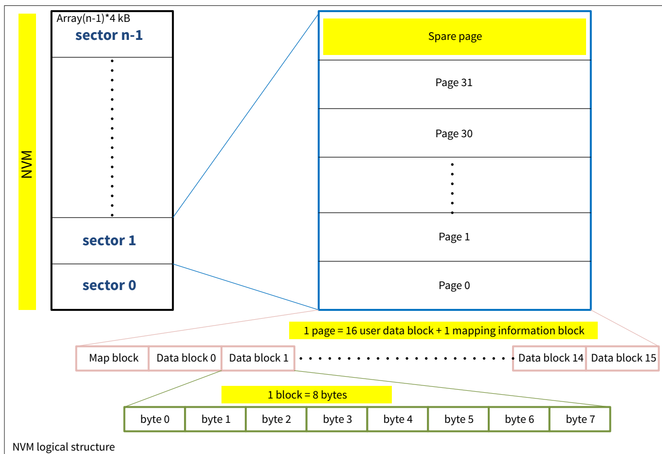
Figure 18 Logical structure of the NVM core
