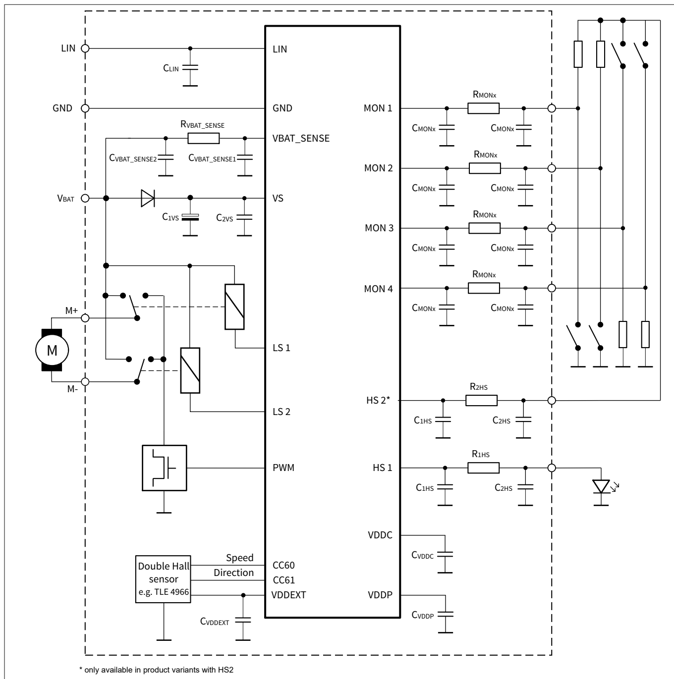
Figure 1 Typical application
