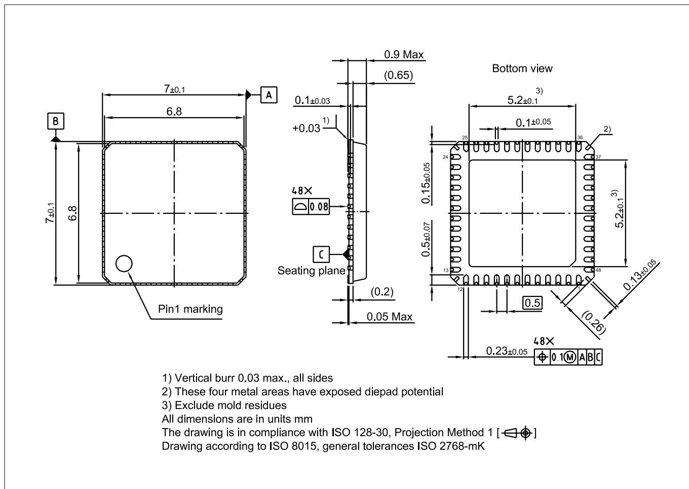
Figure 43 Package outline VQFN-48-31 (with LTI) and VQFN-48-37 (UD step only) 2)
