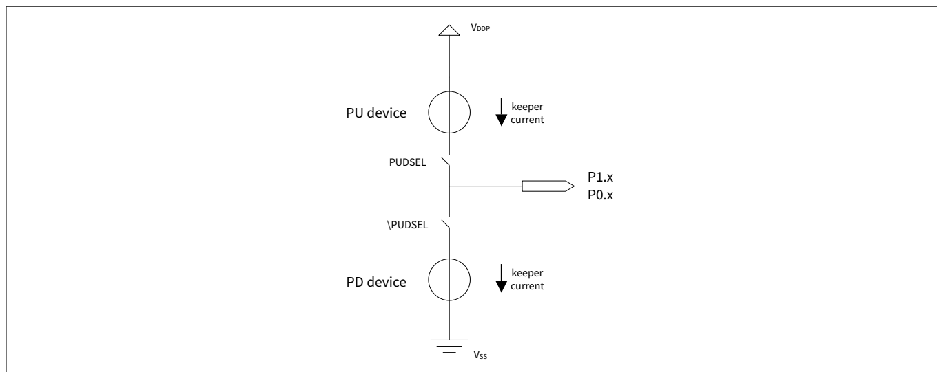
Figure 36 Pull-up/down device
