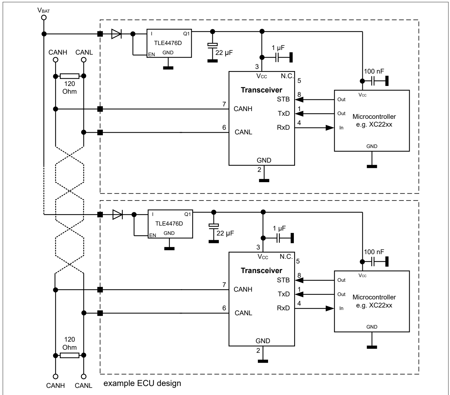
Figure 14 Application circuit
