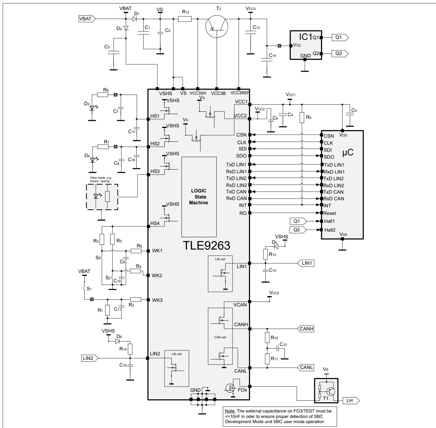
Figure 59 Simplified Application Diagram
