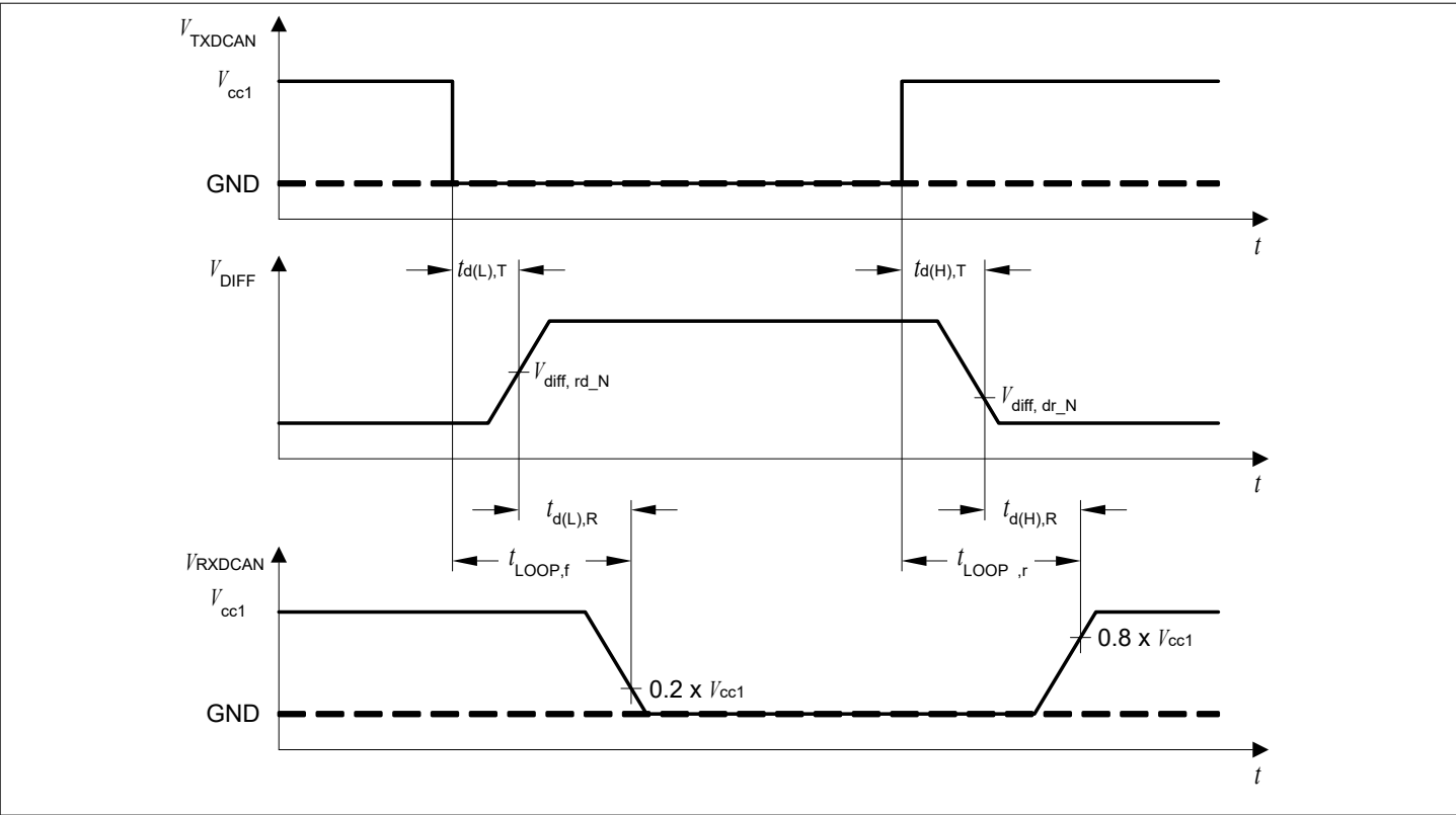
Figure 35 Timing Diagrams for Dynamic Characteristics
