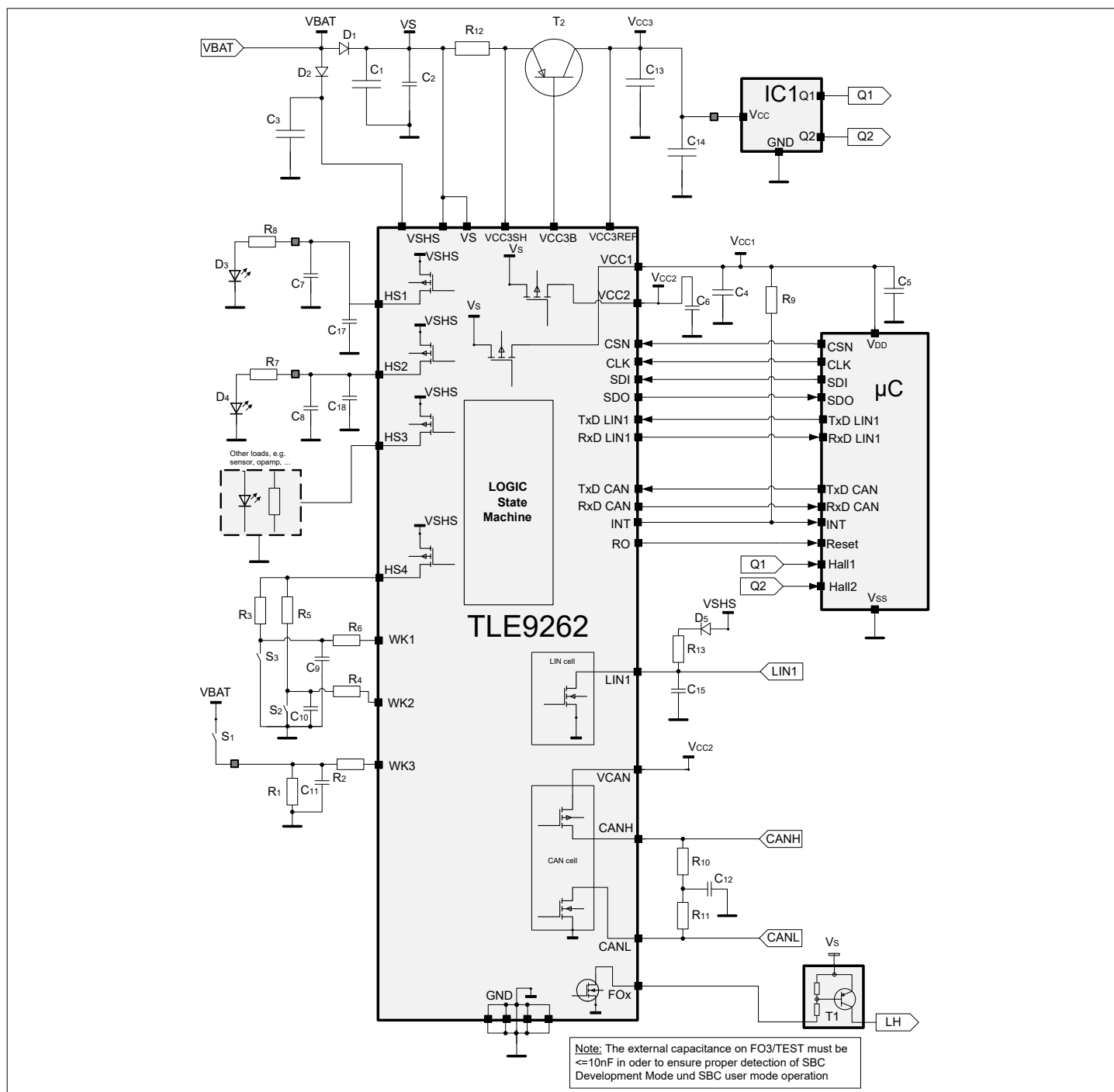
Figure 64 Simplified Application Diagram
