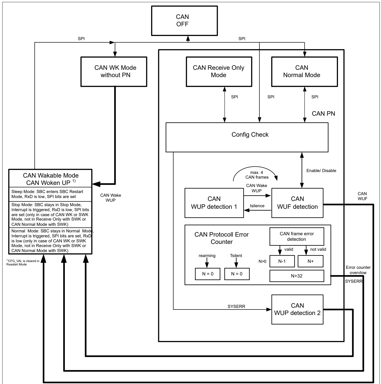
Figure 11 CAN Selective Wake State Diagram
