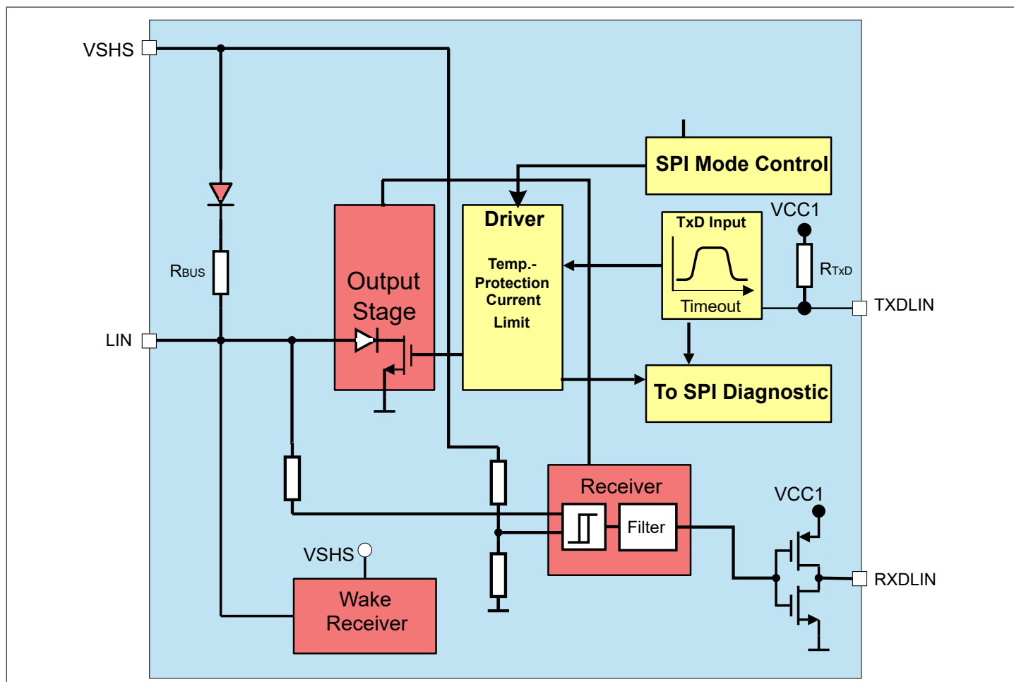
Figure 37 Block Diagram
