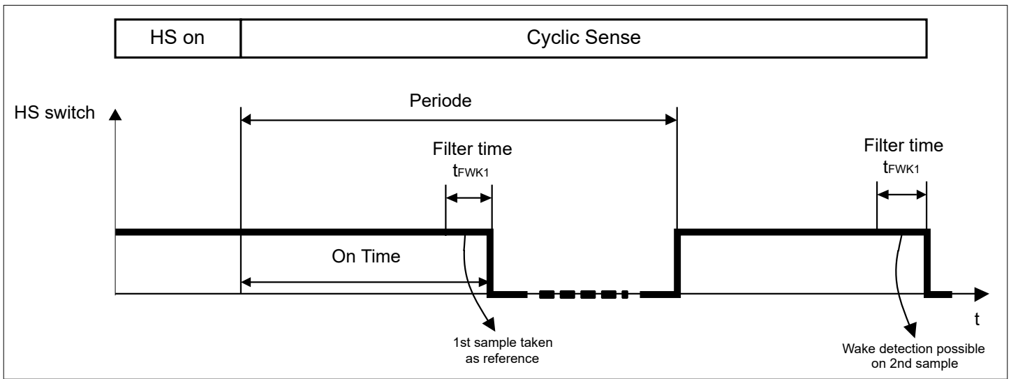
Figure 7 Wake Input Timing
