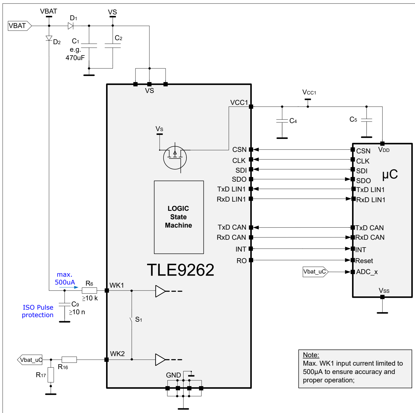
Figure 65 Simplified Application Diagram with the Alternate Measurement Function via WK1 and WK2
