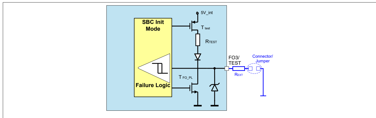
Figure 66 Hint for Increasing the Robustness of pin FO3/TEST during Debugging or Programming
