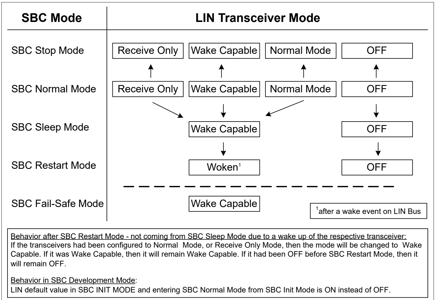
Figure 38 LIN Mode Control Diagram
