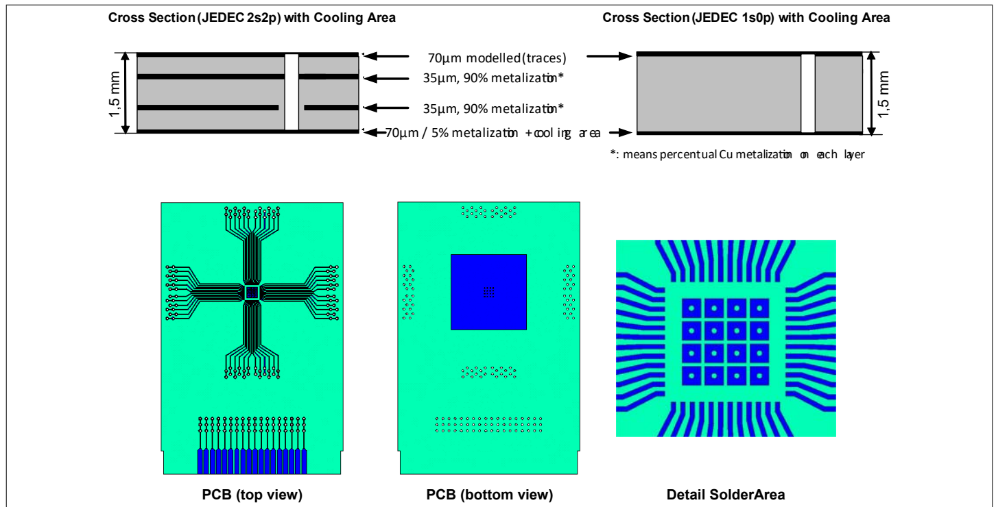
Figure 68 Board Setup
