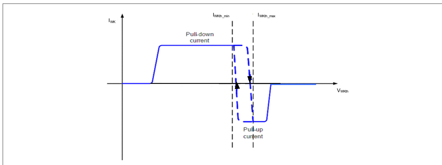
Figure 45 Illustration for Pull-Up / Down Current Sources with Automatic Switching Configuration
