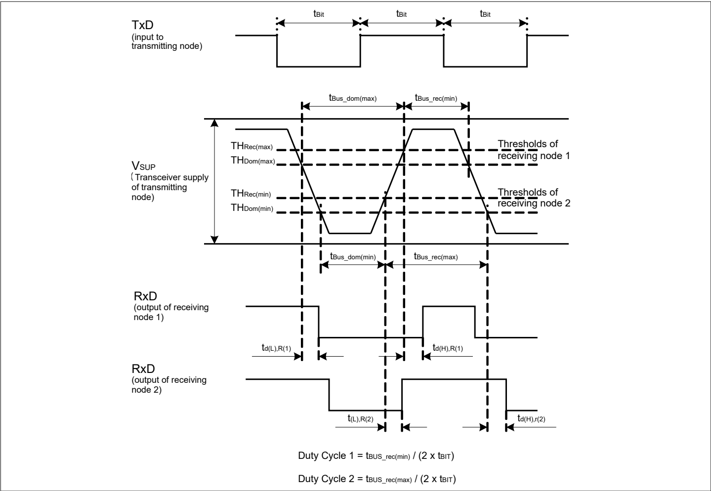
Figure 42 Timing Diagram for Dynamic Characteristics
