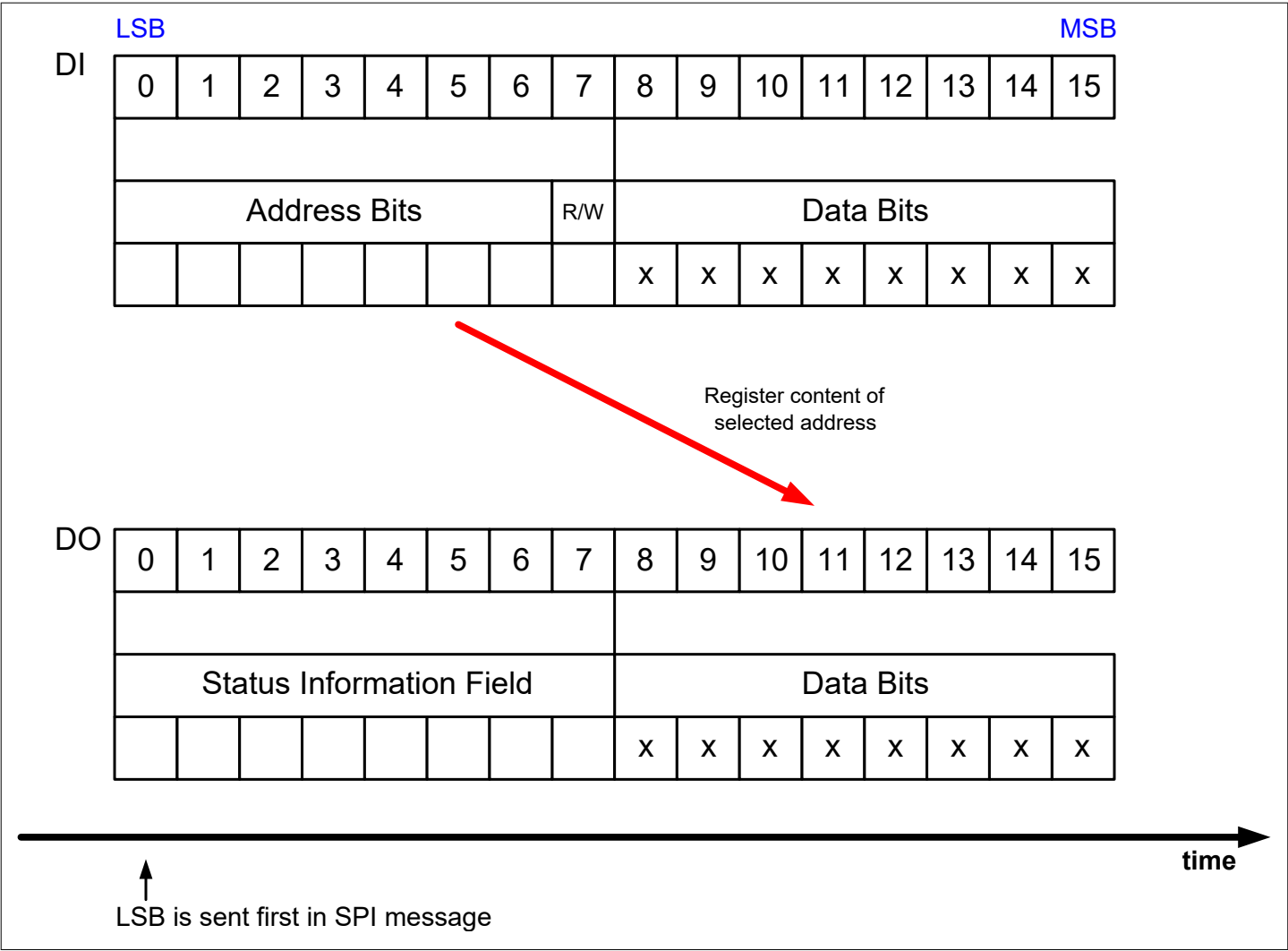
Figure 60 SPI Operation Mode
