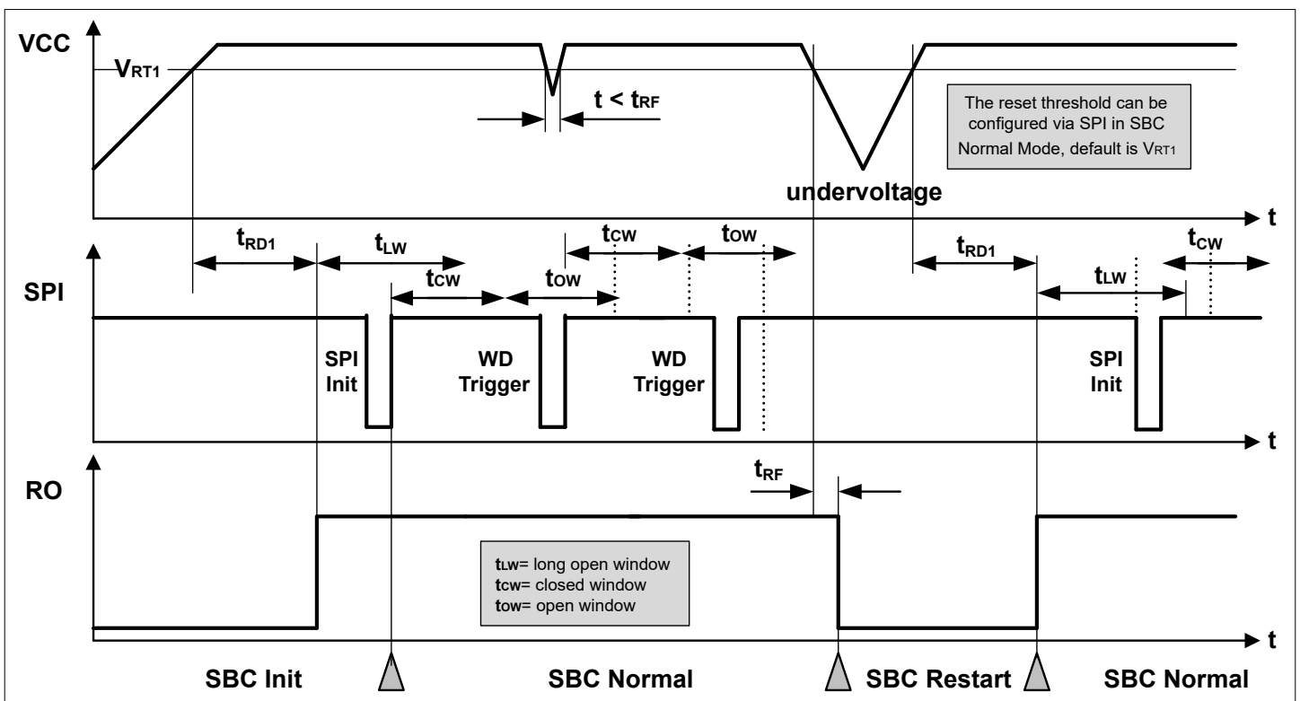
Figure 52 Reset Timing Diagram
