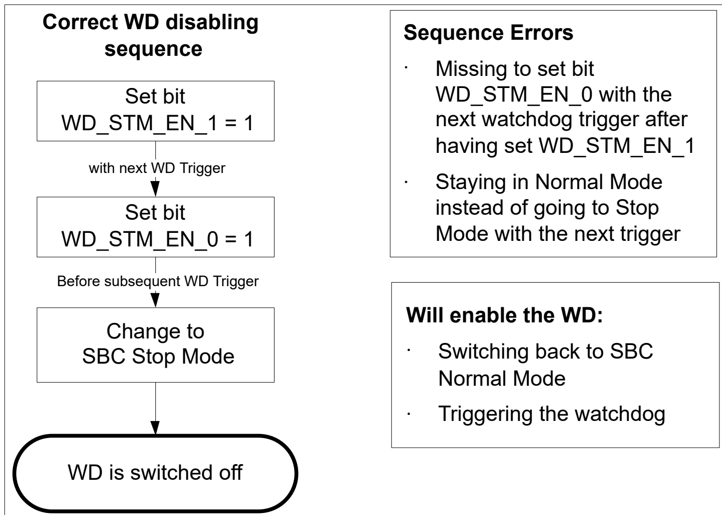
Figure 55 Watchdog disabling sequence in SBC Stop Mode
