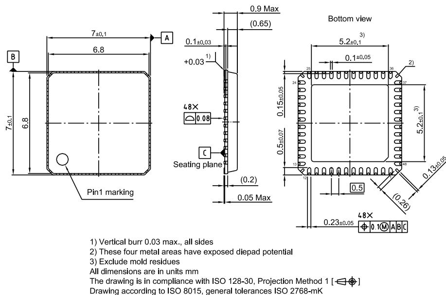
Figure 69 PG-VQFN-48
