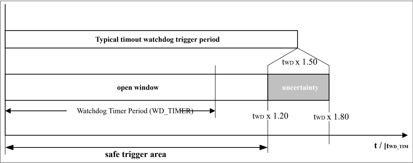
Figure 53 Time-out Watchdog Definition
