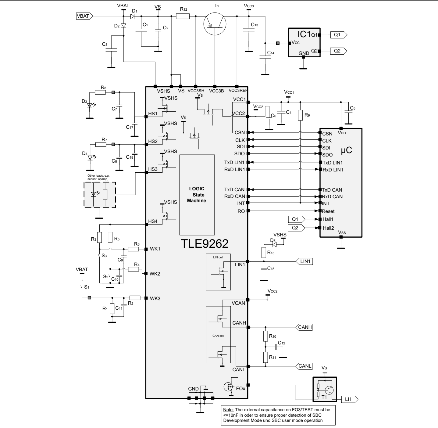
Figure 64 Simplified Application Diagram
