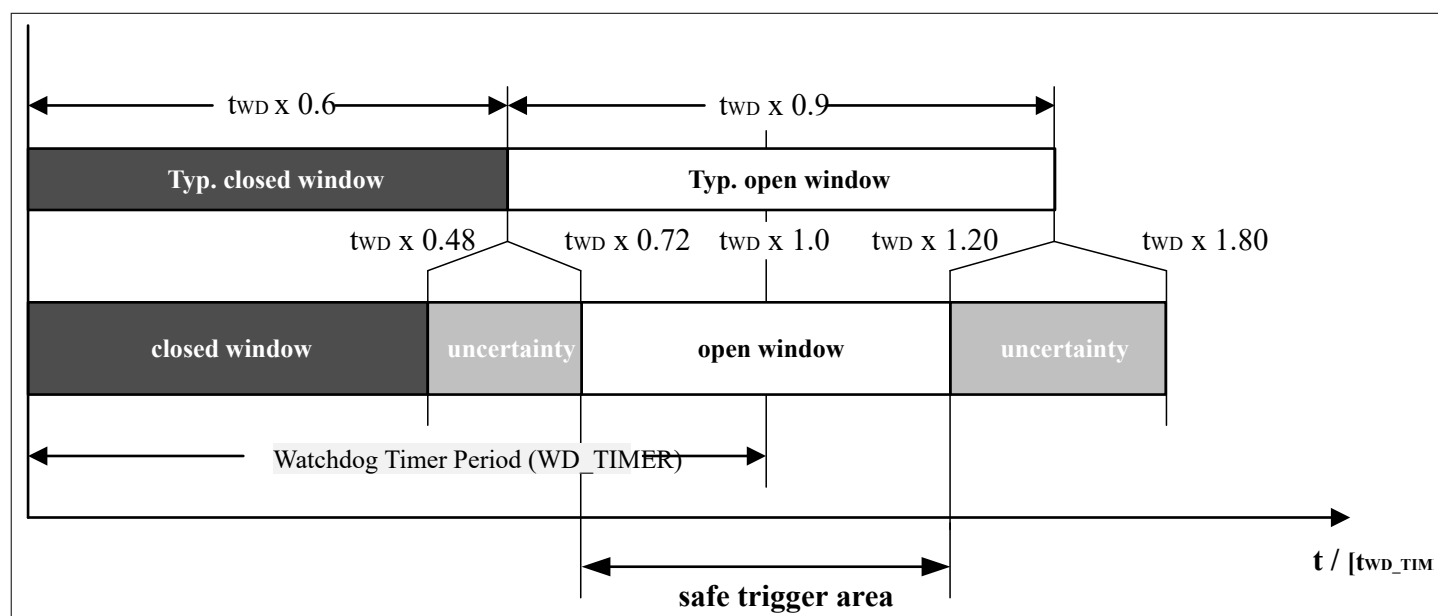
Figure 54 Window Watchdog Definition
