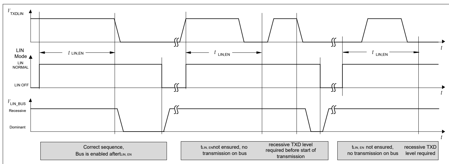
Figure 39 LIN Transceiver Enabling Sequence
