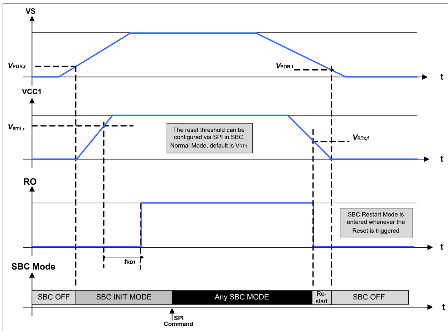
Figure 56 Ramp up / down example of Supply Voltage
