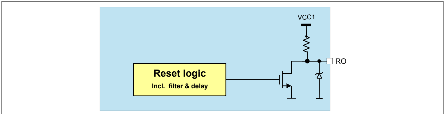
Figure 51 Reset Block Diagram
