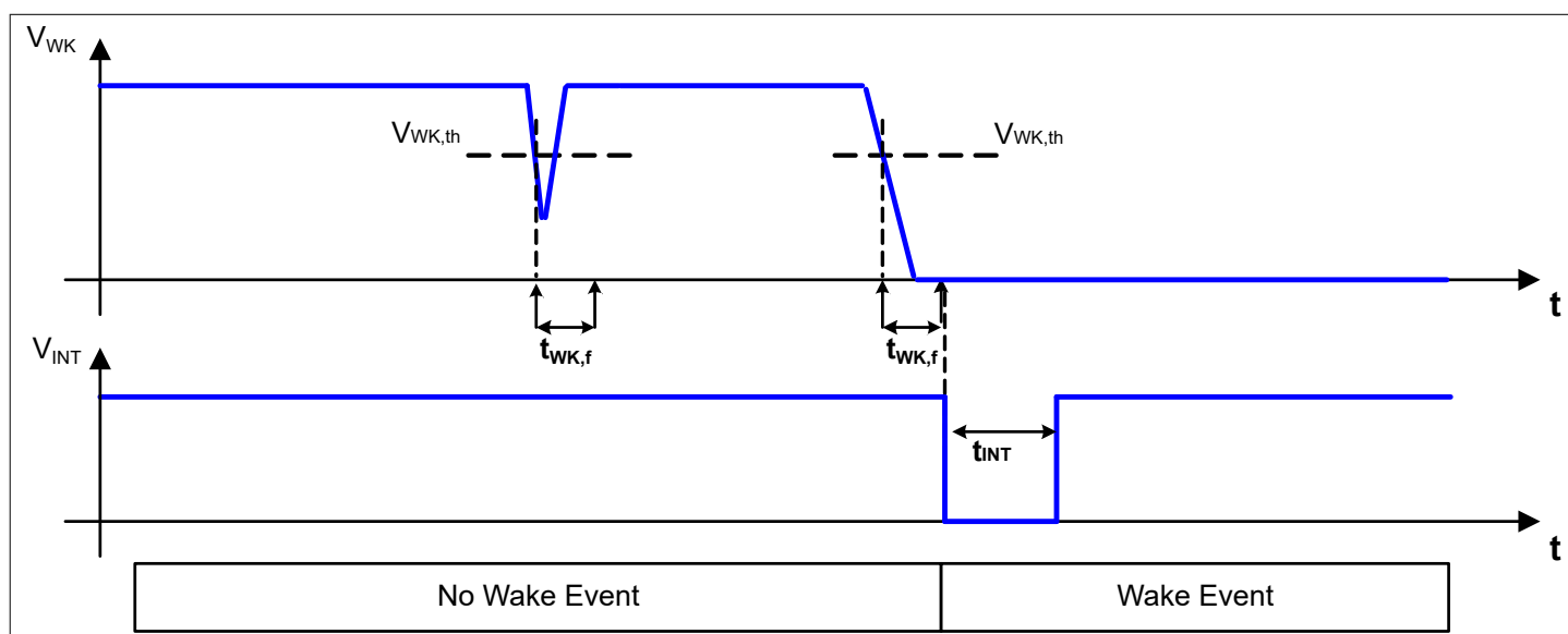
Figure 44 Wake-up Filter Timing for Static Sense
