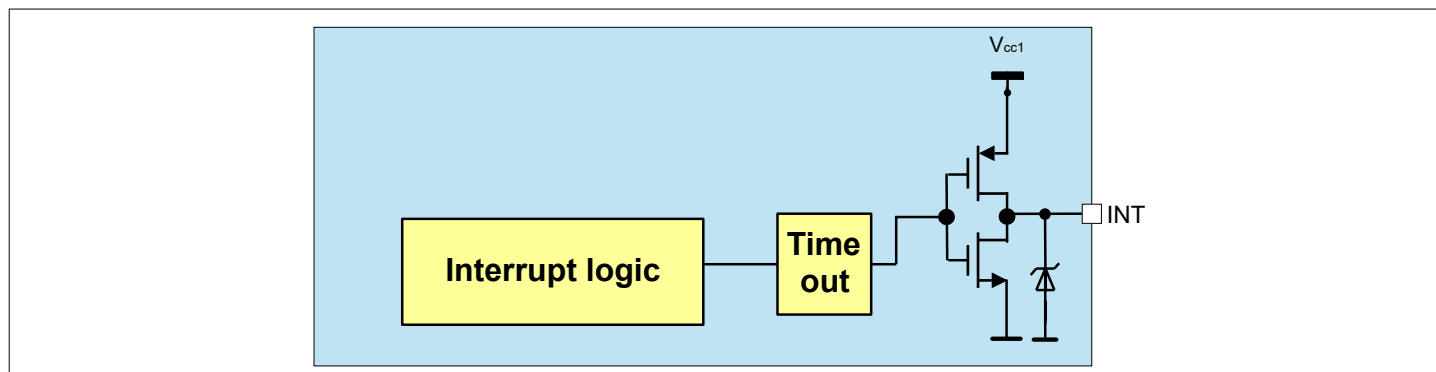
Figure 47 Interrupt Block Diagram
