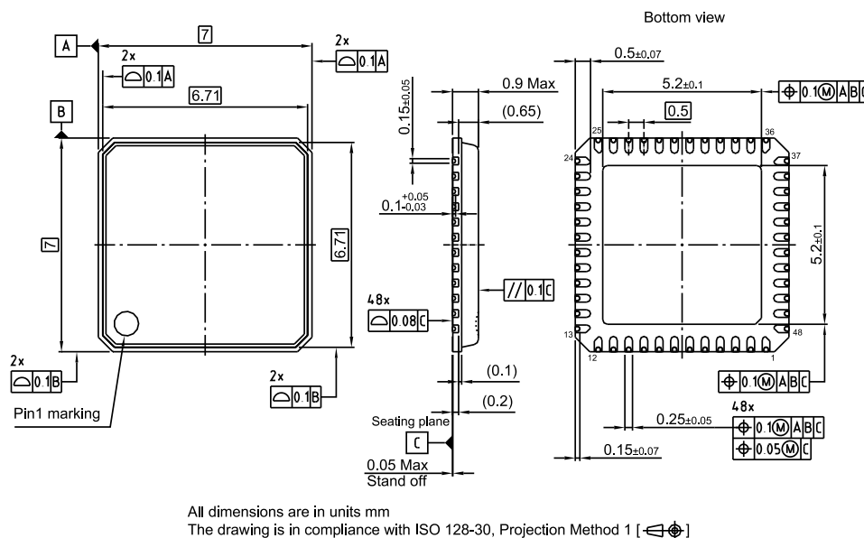
Figure 70 PG-VQFN-48
