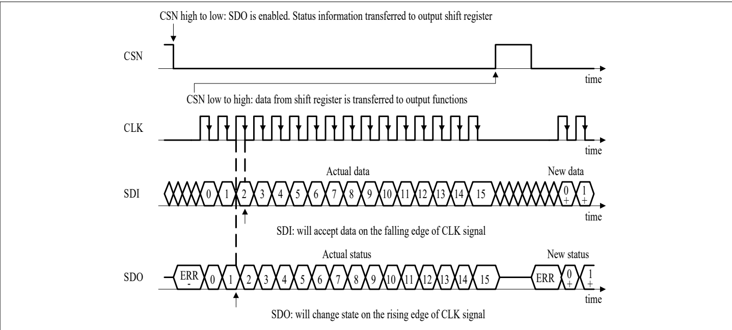
Figure 59 SPI Data Transfer Timing (note the reversed order of LSB and MSB shown in this figure compared to the register description)
