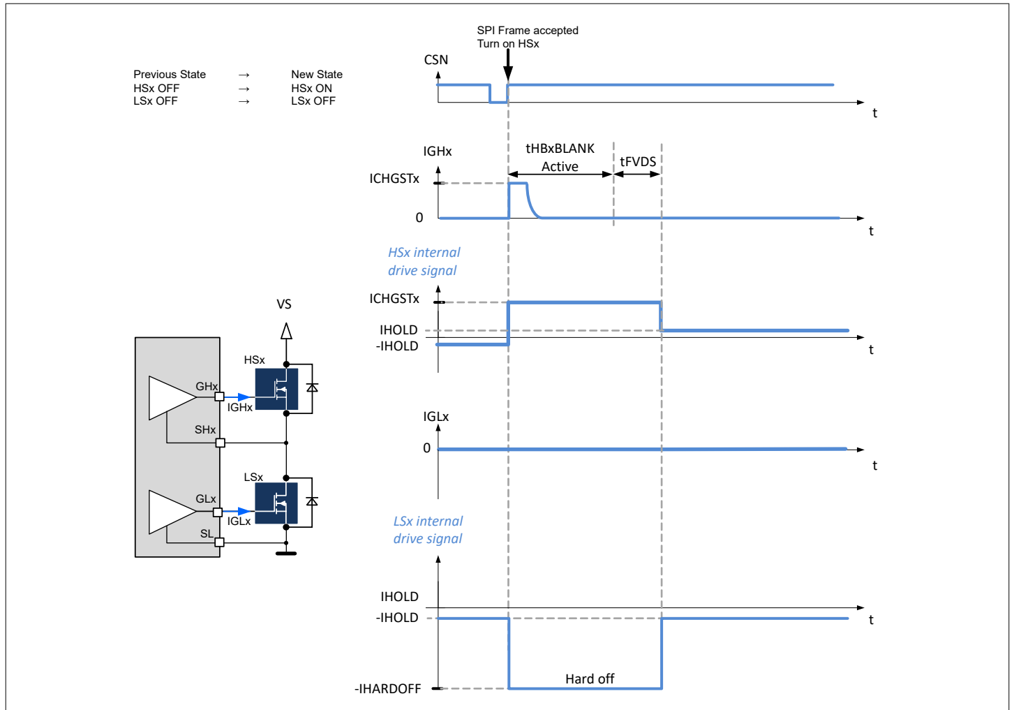
Figure 8 Turn-on of a high-side MOSFET without cross-current protection
