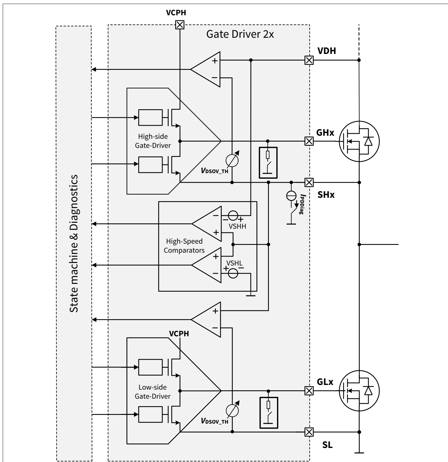
Figure 8 Simplified block diagram: gate driver
