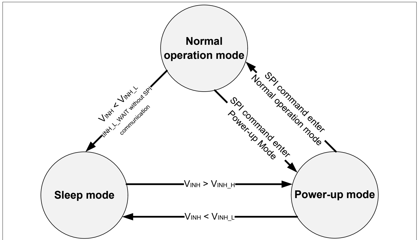
Figure 3 State diagram
