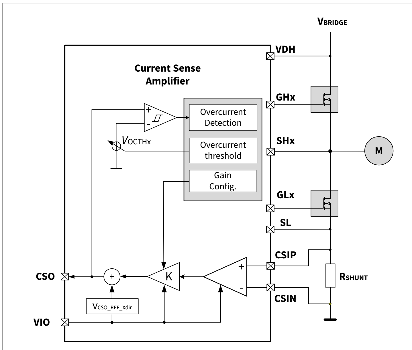
Figure 15 Simplified block diagram: CSA Module
