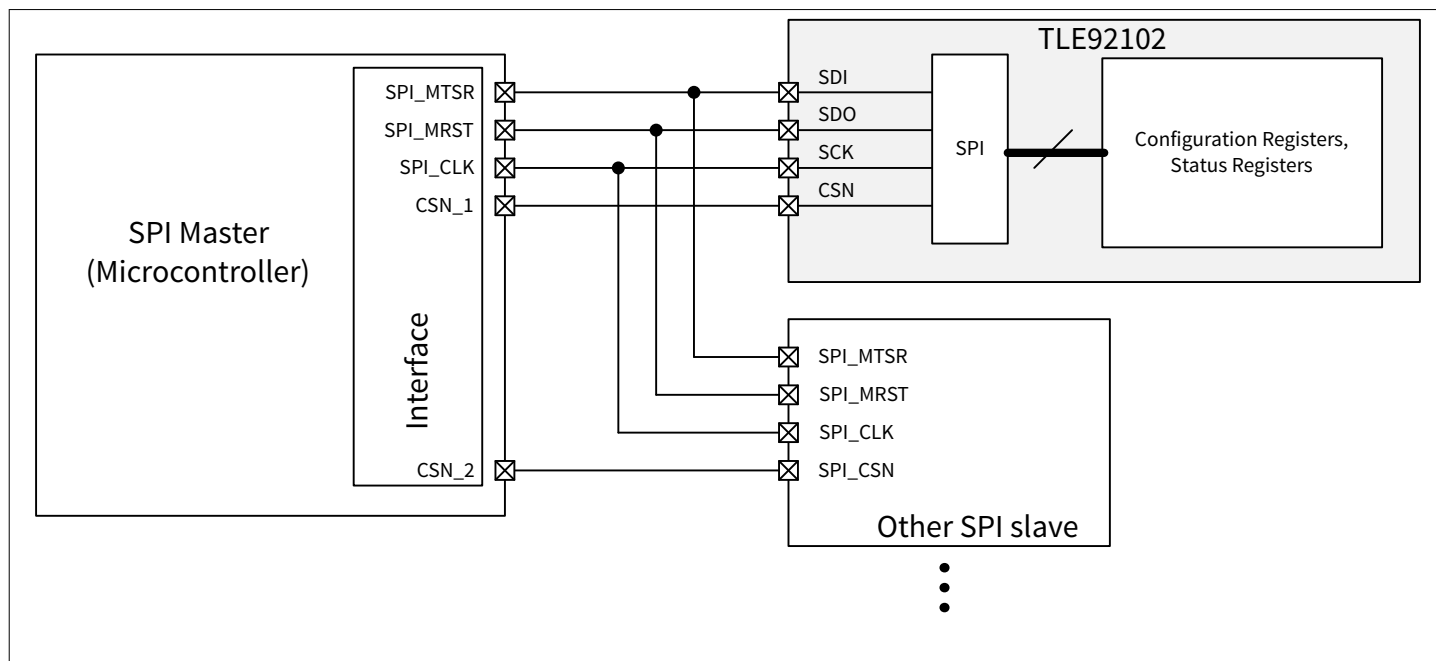
Figure 16 Simplified block diagram: SPI
