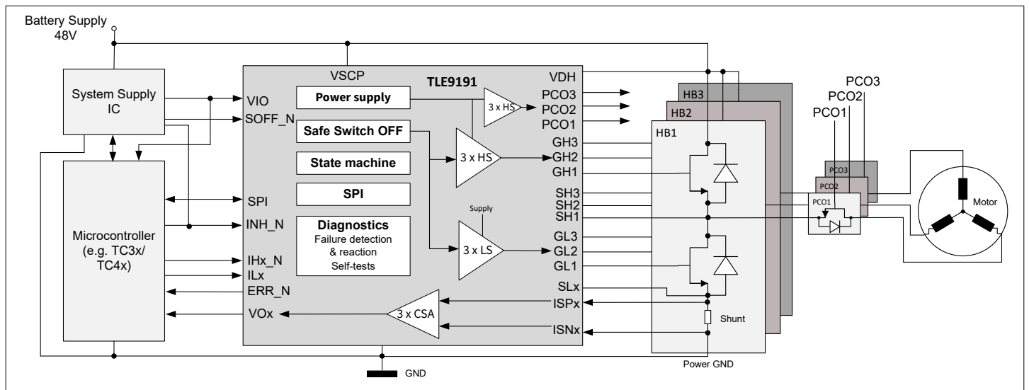
Simplified application diagram
