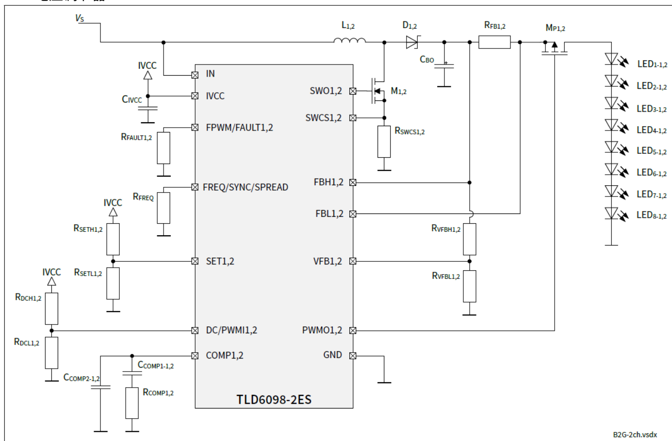
Figure 1 Application diagram
