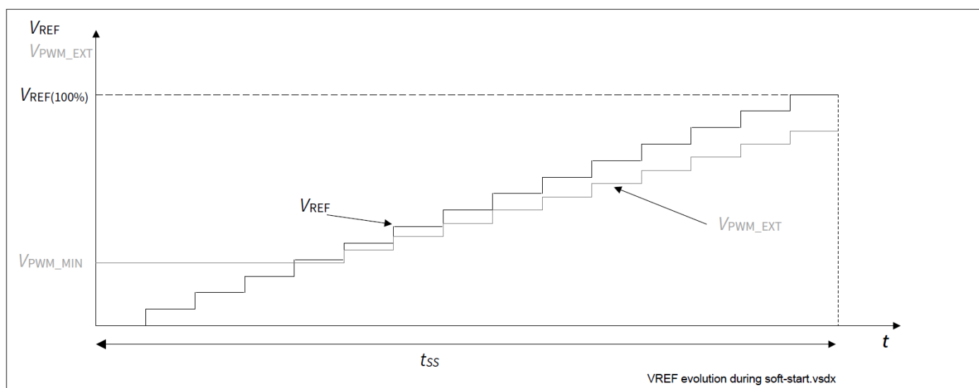
Figure 5 V_{REF} and V_{PWM\_EXT} waveforms during the soft start routine without analog output adjustment
