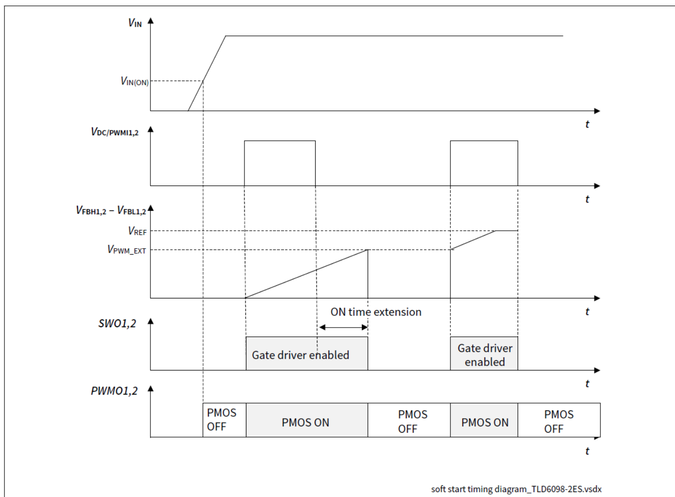
Figure 4 Soft start timing diagram (the linear waveform of VVFBH-VVFBFBL is an example of possible scenario)
