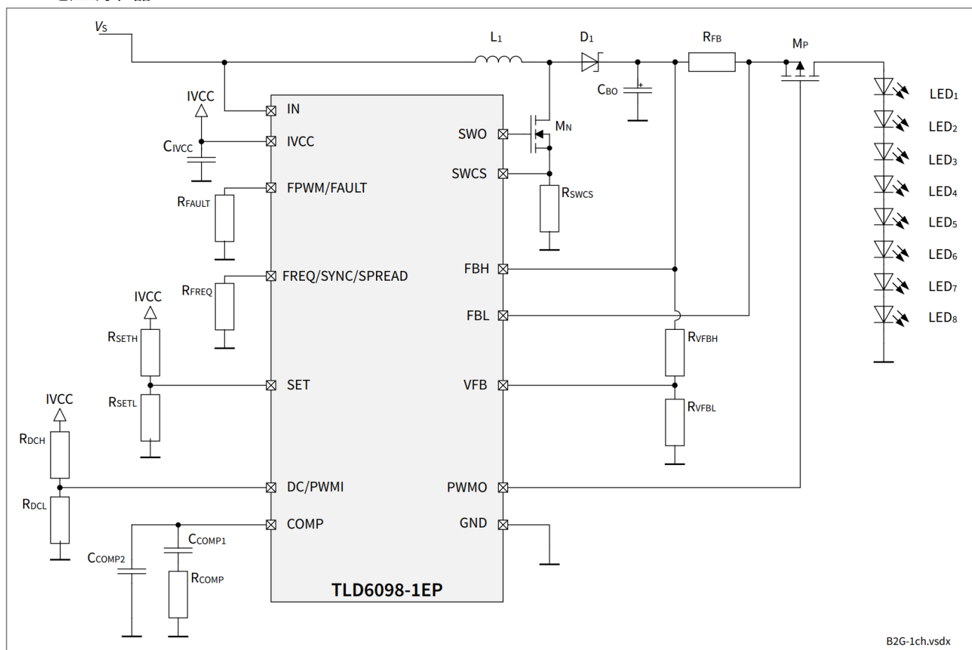
Figure 1 Application diagram
