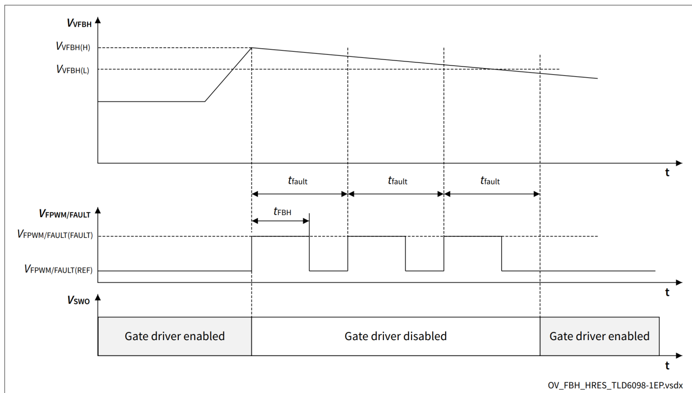
Figure 19 Timing diagram during overvoltage on FBH detection with R_{FPWM/FAULT(H)} used on FPWM/FAULT pin
