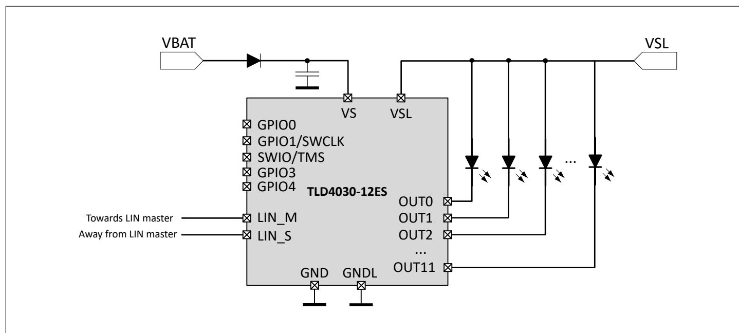
Figure 2 Application block diagram (simplified)
