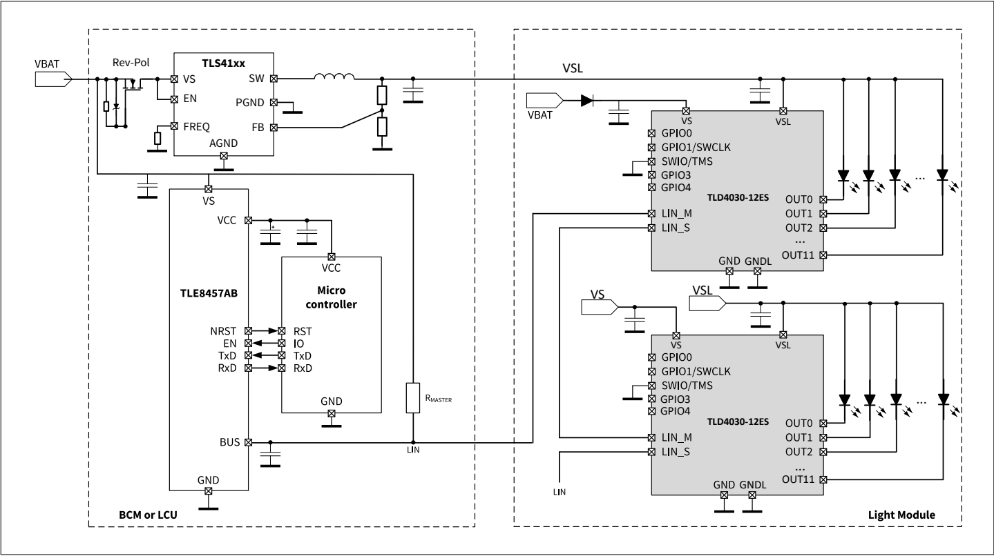
Figure 11 Application diagram
