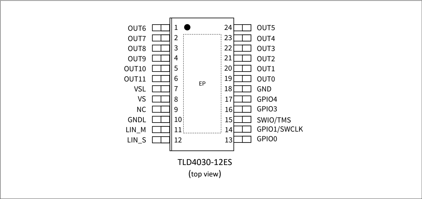
Figure 4 TLD4030-12ES pinout
