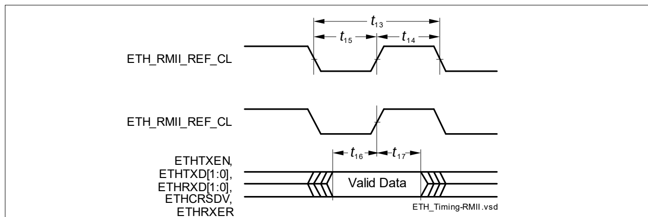
Figure 3-20 ETH RMII Signal Timing
