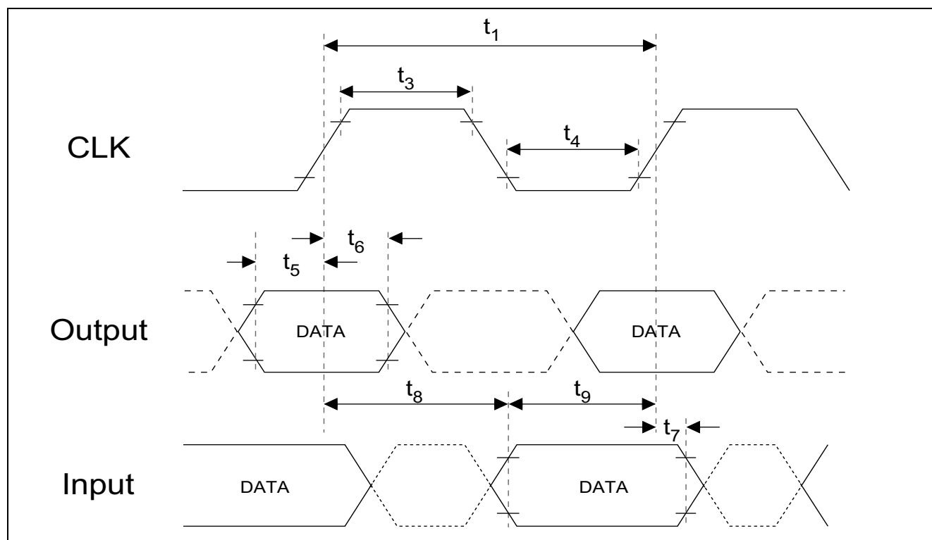
Figure 3-24 SDMMC Timing
