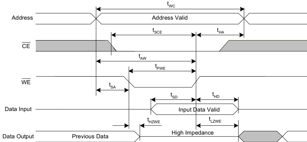
Figure 7. SRAM Write Cycle No. 2 ( \overline{\text{CE}} Controlled) [18, 19, 20]
