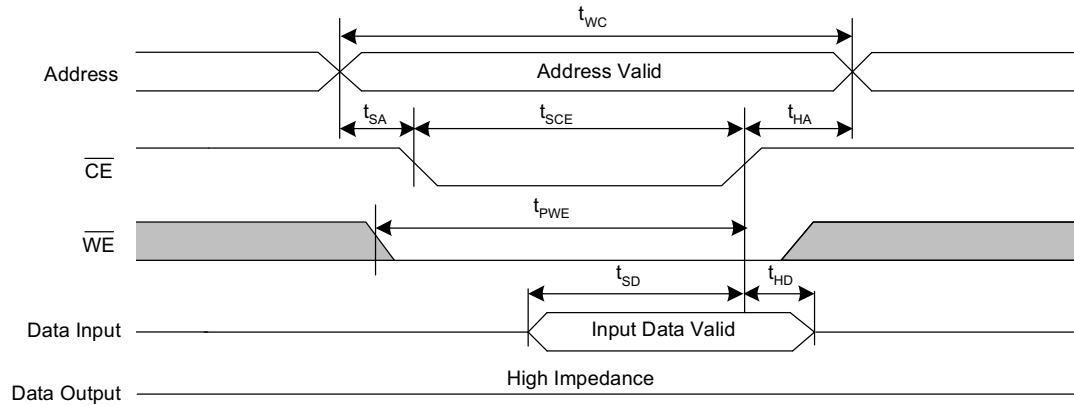
Figure 7. SRAM Write Cycle No. 2 ( \overline{\text{CE}} Controlled) [18, 19, 20]
