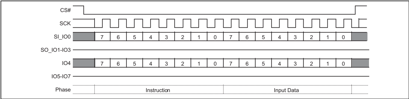
Figure 38 Bank Register Write (BRWR 17h) command
