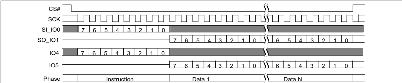
Figure 51 Dual-Quad DLP Read (DLPRD 41h) command sequence
