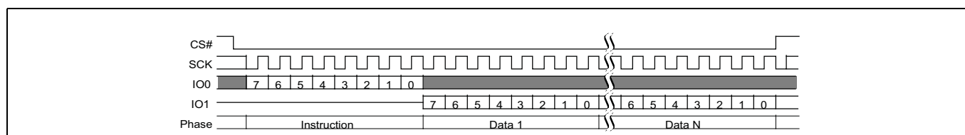
Figure 32 Read Identification (RDID 9Fh) command sequence
