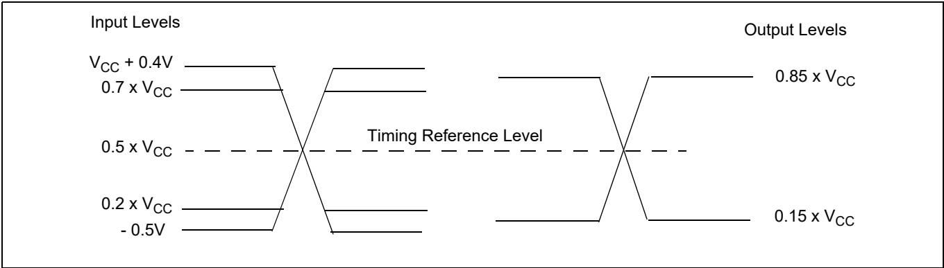
Figure 16 Input, output, and timing reference levels
