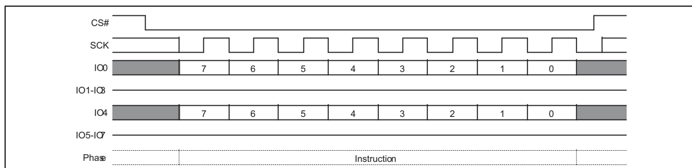
Figure 39 BRAC (B9h) command sequence
