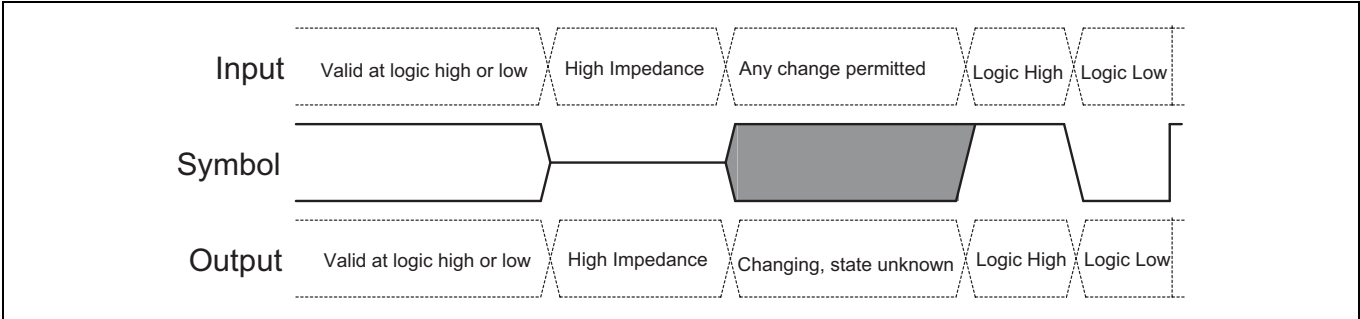
Figure 15 Waveform element meanings
