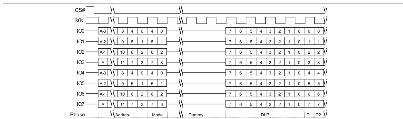
Figure 58 Dual-Quad Continuous DDR Quad I/O Read subsequent access [41, 42]
