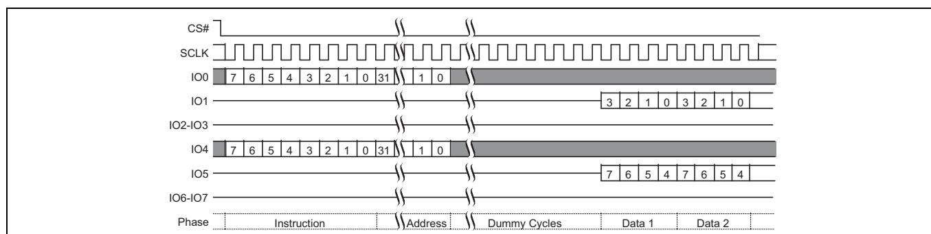
Figure 53 Dual-Quad SPI Fast Read (FAST_READ) command sequence
