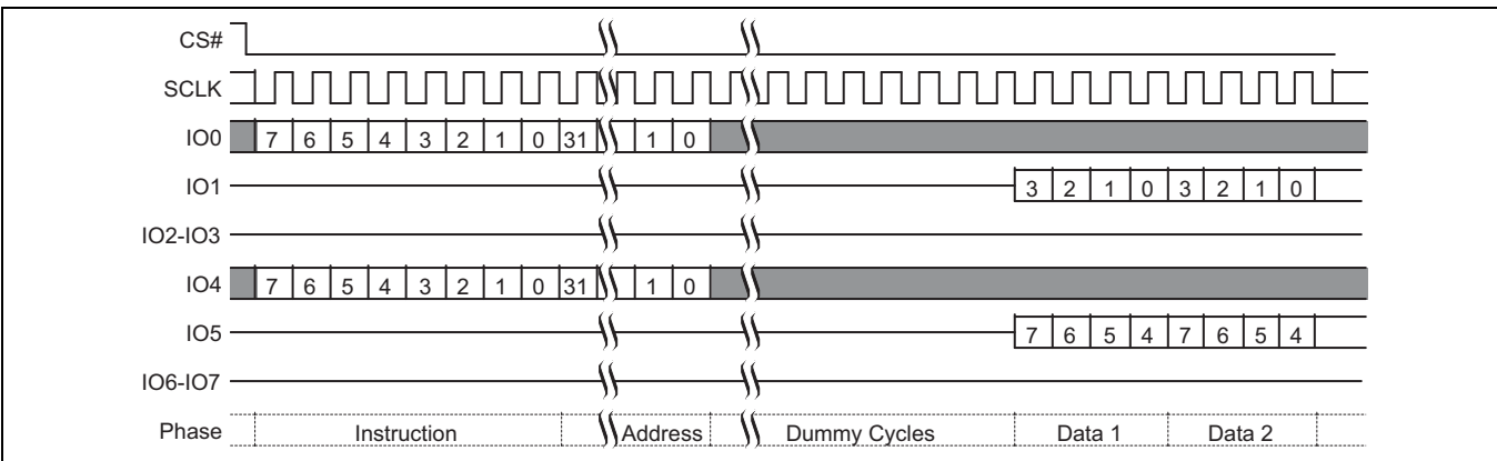
Figure 68 Read OTP (OTPR 4Bh) command sequence
