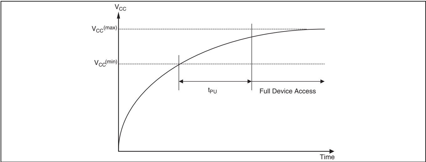
Figure 13 Power-up
