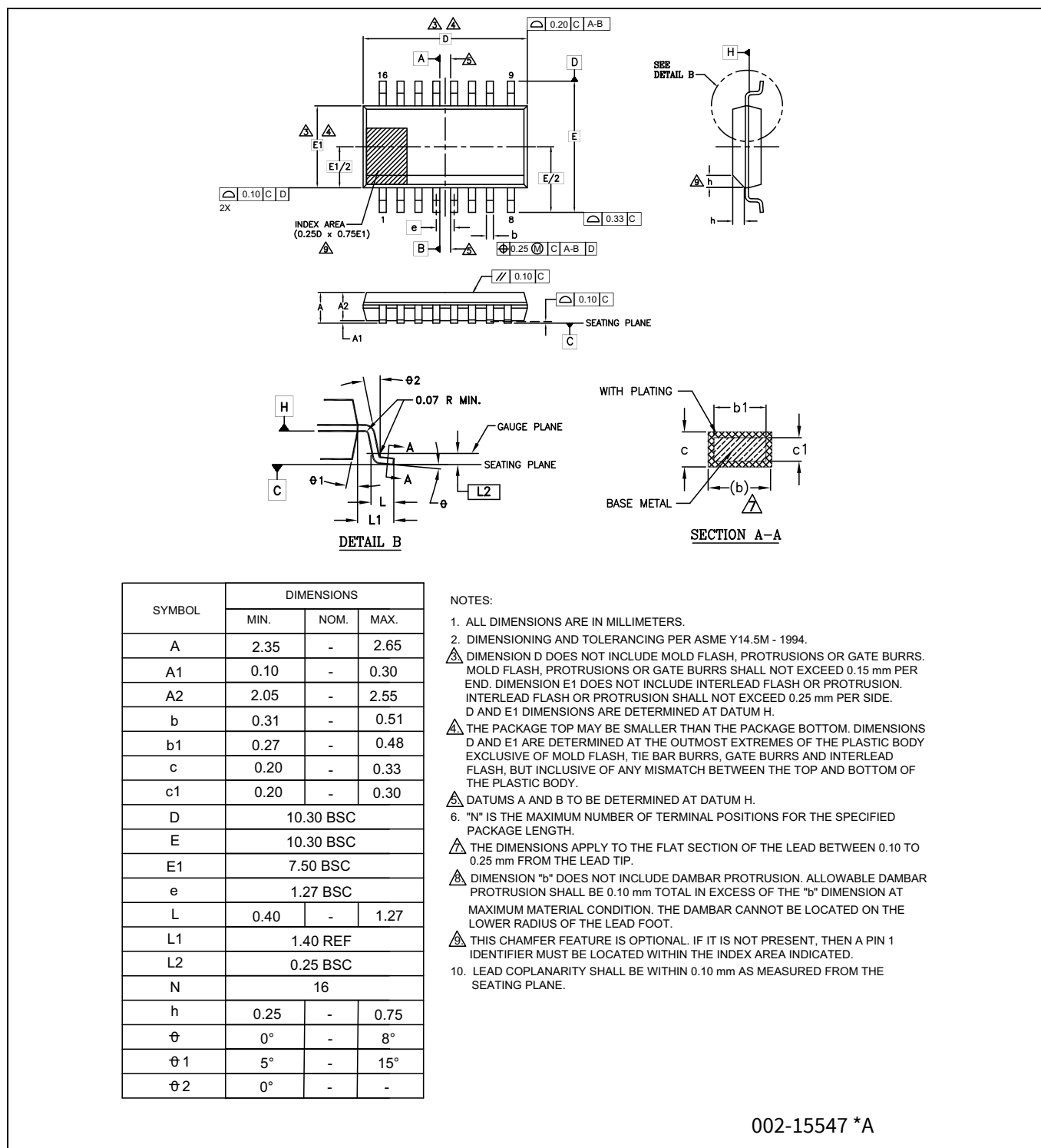
Figure 28 16-pin SOIC (10.30 × 7.50 × 2.65 mm) package outline, (PG-DSO-16)
