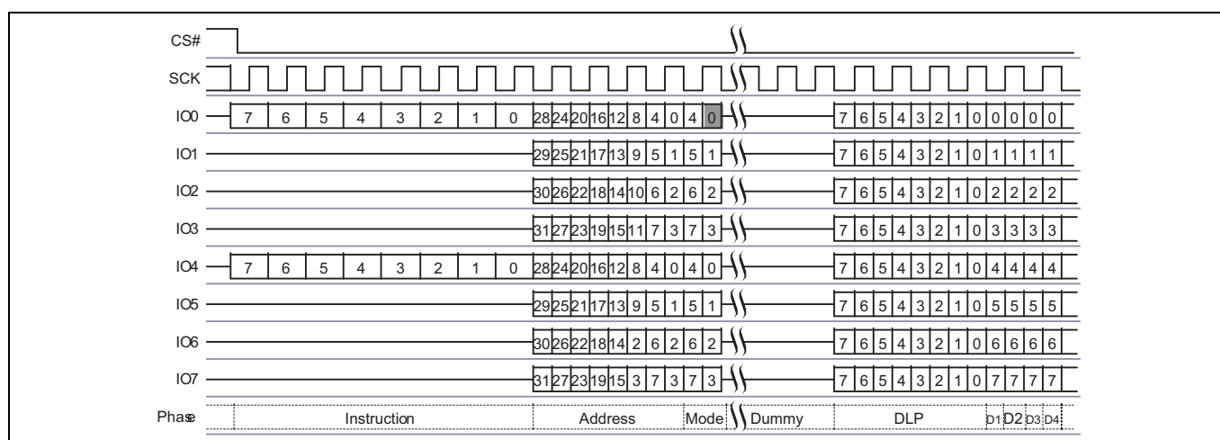
Figure 10 Dual-Quad DDR Quad I/O Read command
