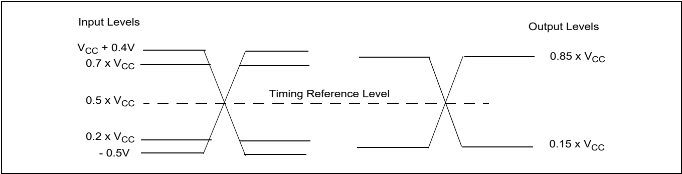
Figure 16 Input, output, and timing reference levels
