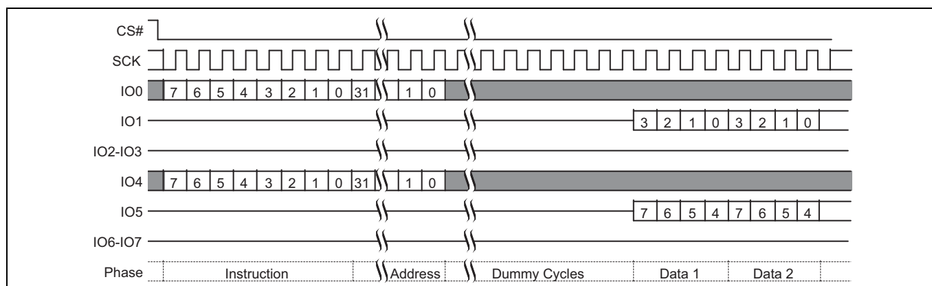
Figure 54 Dual-Quad SPI Fast Read (FAST_READ) command sequence
