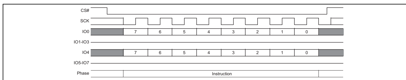
Figure 62 Dual-Quad Program Suspend command sequence
