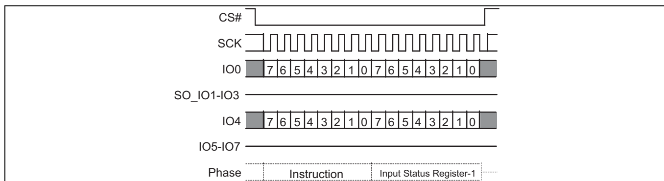
Figure 41 Dual-Quad Write Registers
