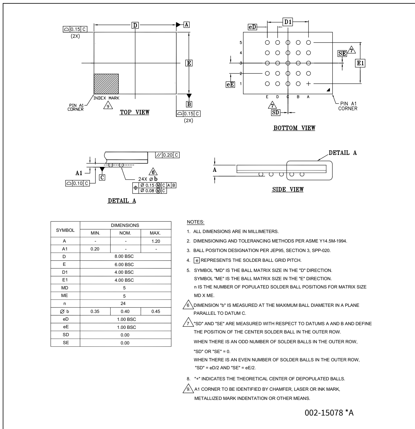
Figure 28 24-ball FBGA (8.0 × 6.0 × 1.2 mm) package outline, (PG-TFBGA-24)
