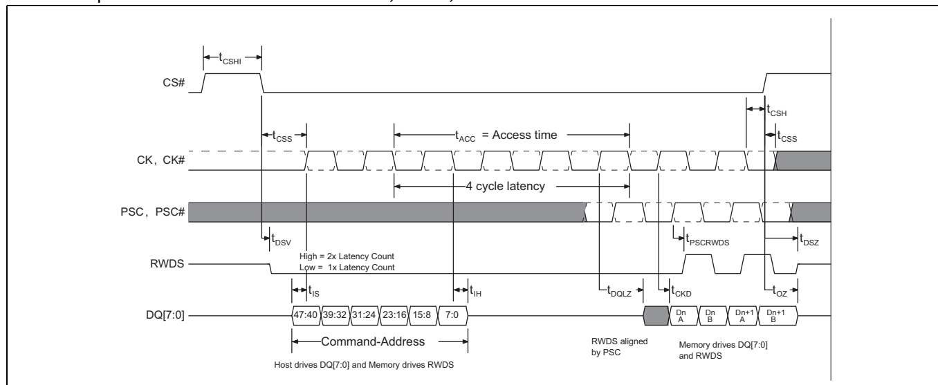
Figure 12-3 HyperRAM Memory DCARS Timing Diagram [67, 68, 69]
