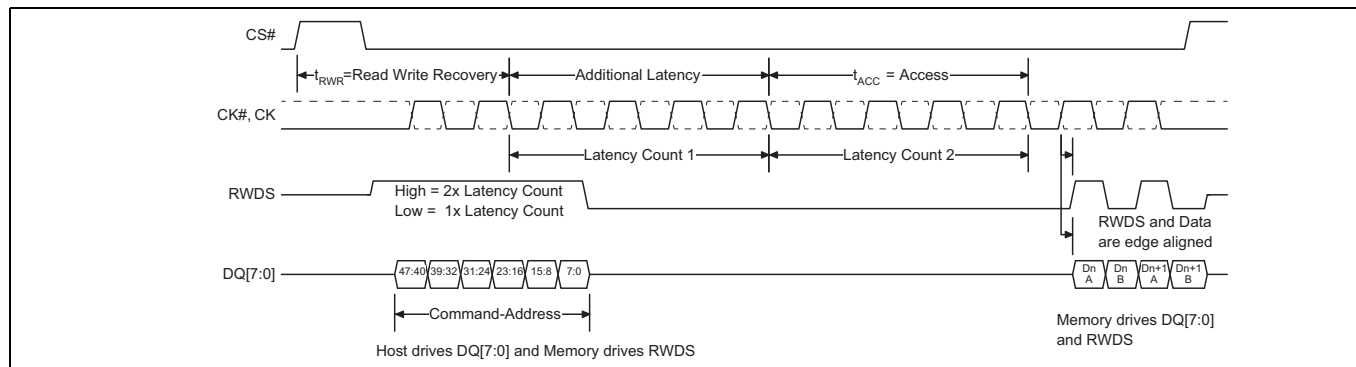
Figure 1-2 Read Transaction
