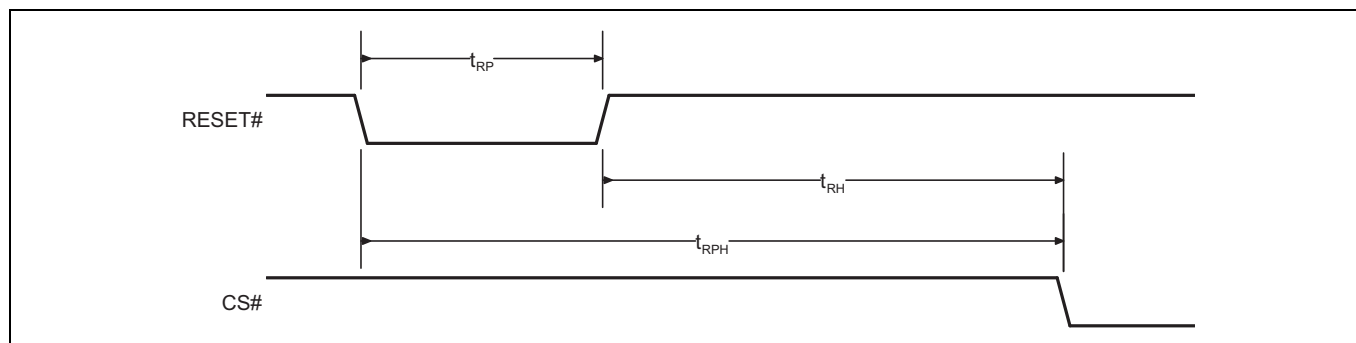
Figure 9-5 Hardware Reset Timing Diagram
