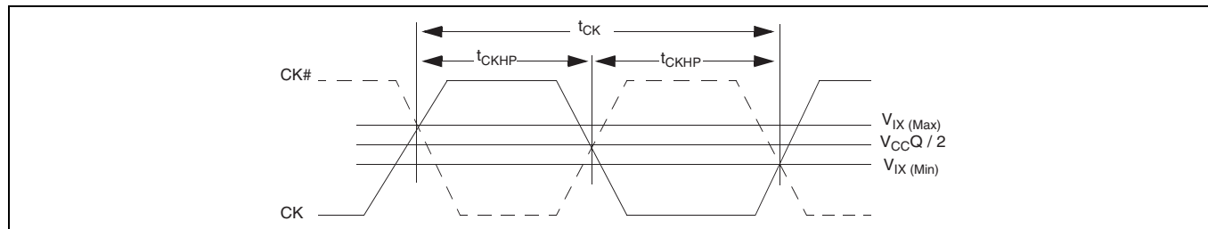
Figure 10-3 Clock Characteristics
