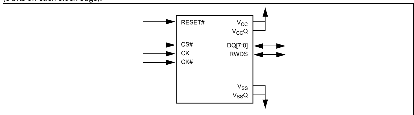
Figure 2-1 HyperRAM Interface [3]
