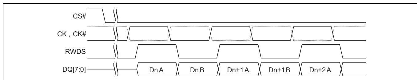
Figure 4-2 Data Placement During a Read Transaction [14, 15, 16, 17, 18]
