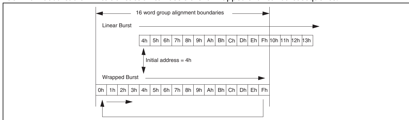
Figure 1-4 Linear Versus Wrapped Burst Sequence
