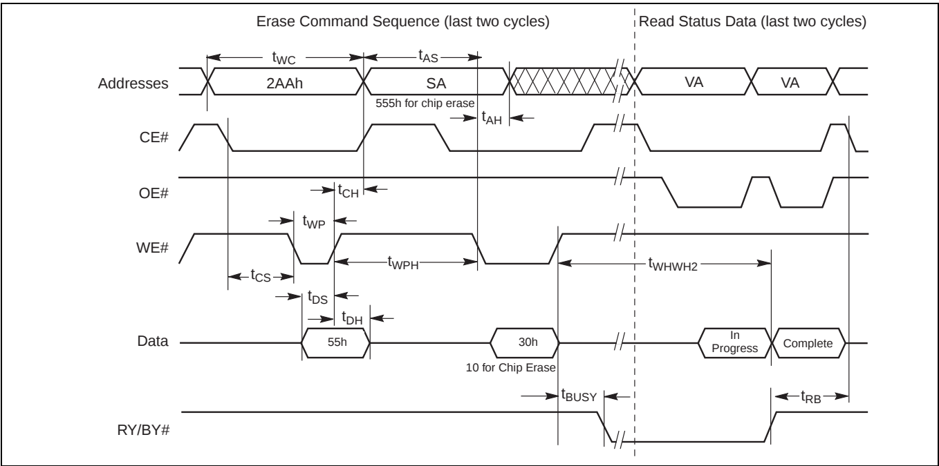
Figure 27 Chip/sector erase operation timing diagram [98]
