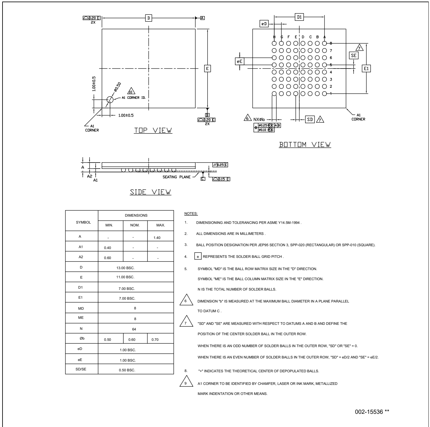
Figure 38 64-ball FBGA 13.0 x 11.0 x 1.4 mm LAA064, package outline (PG-LFBGA-64)
