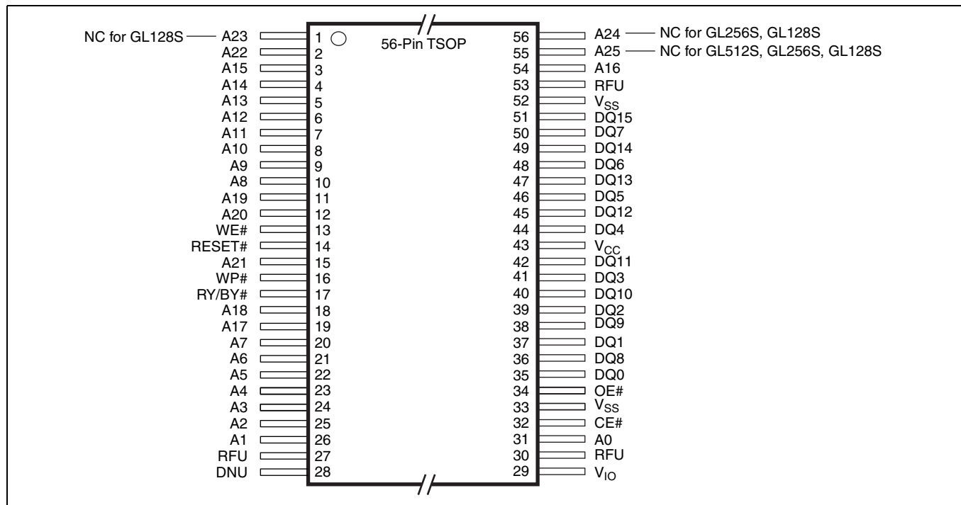
Figure 34 56-lead standard TSOP [105, 106]
