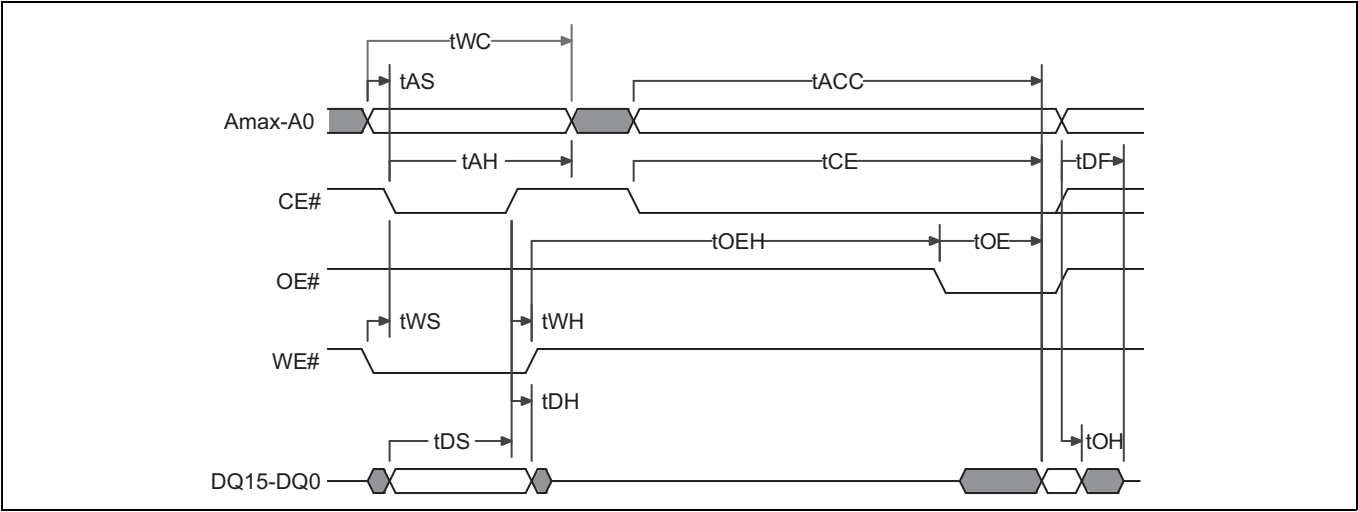
Figure 33 (CE#) write to read operation timing diagram
