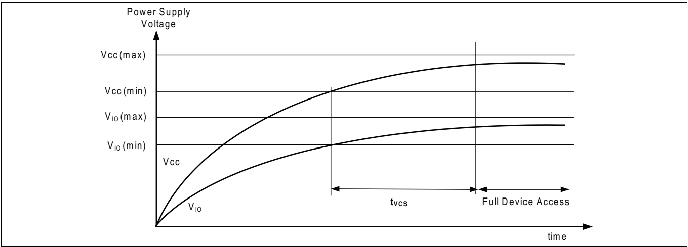
Figure 9 Power-up
