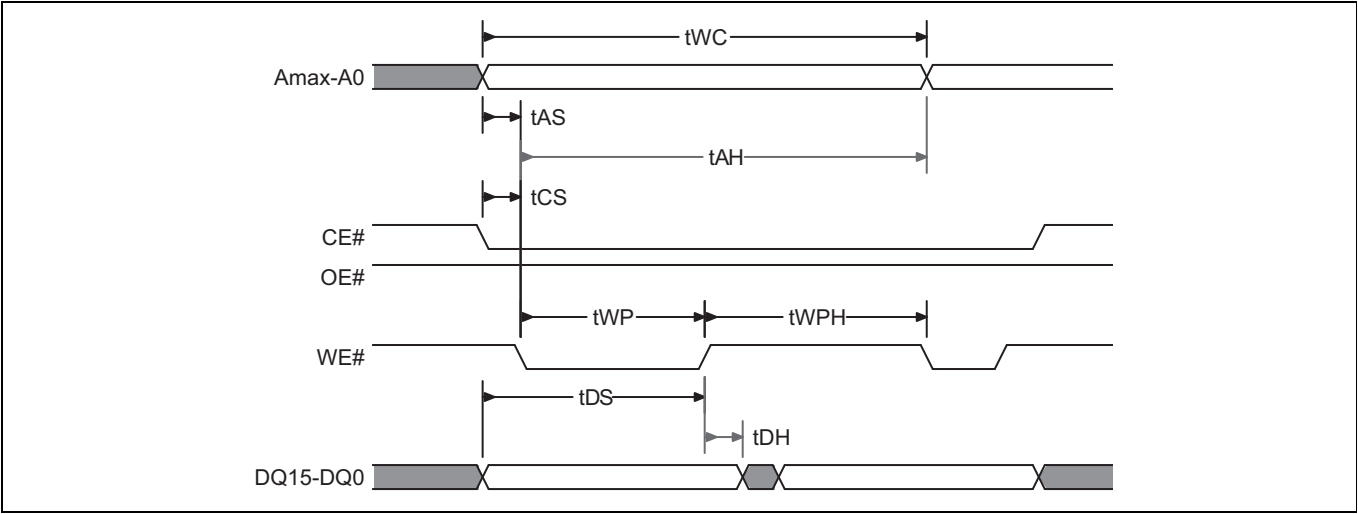
Figure 21 Back-to-back (CE#VIL) write operation timing diagram
