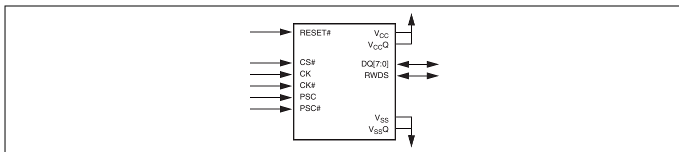
Figure 42 xSPI product with DCARS signal diagram
