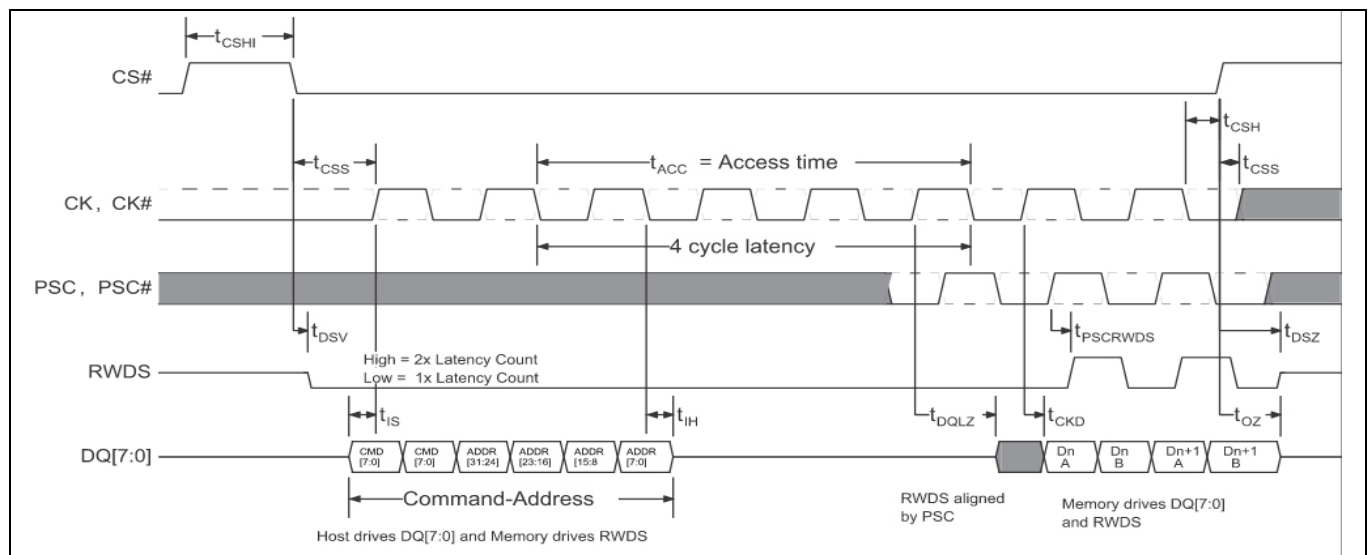
Figure 44 HYPERRAM™ memory DCARS timing diagram [61, 62, 63]
