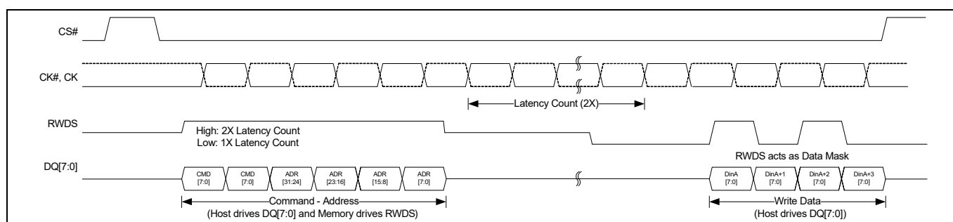
Figure 16 WRITE with 2X latency transaction (DDR) [22, 23]
