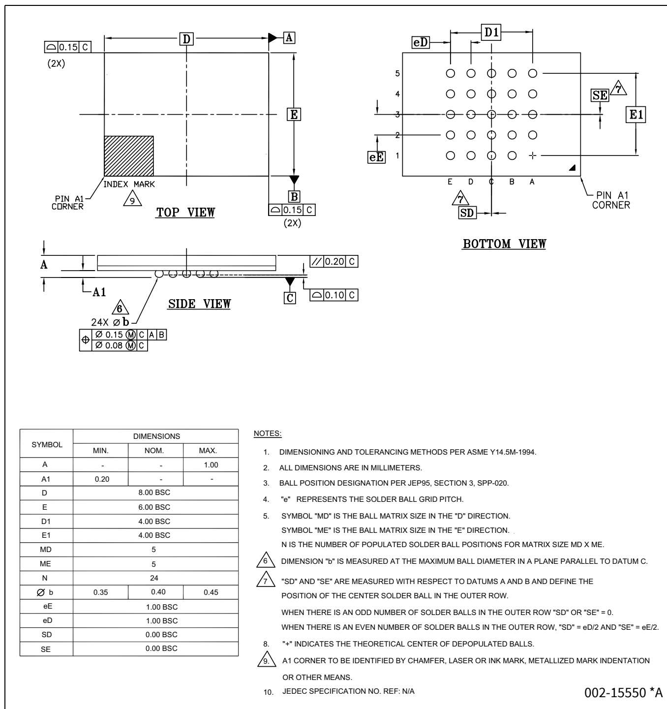
Figure 41 Fortified ball grid array 24-ball 6 × 8 × 1.0 mm (VAA024)
