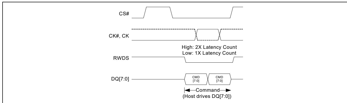
Figure 18 WRITE DISABLE transaction (DDR)
