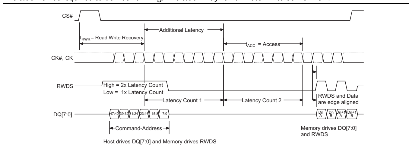
Figure 4-4 Read Transaction with Additional Initial Latency [21-28]
