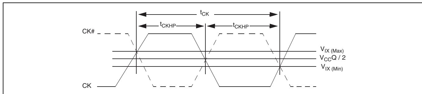
Figure 10-3 Clock Characteristics
