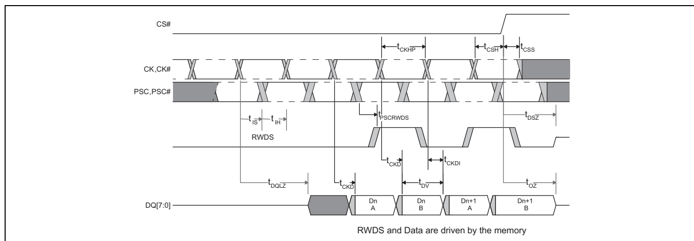
Figure 12-4 DCARS Data Valid Timing [72, 70, 70]
