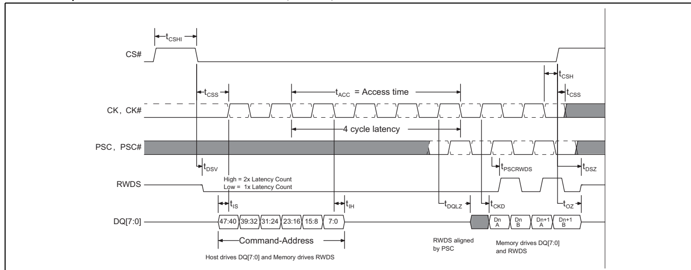
Figure 12-3 HyperRAM Memory DCARS Timing Diagram [65, 66, 67]
