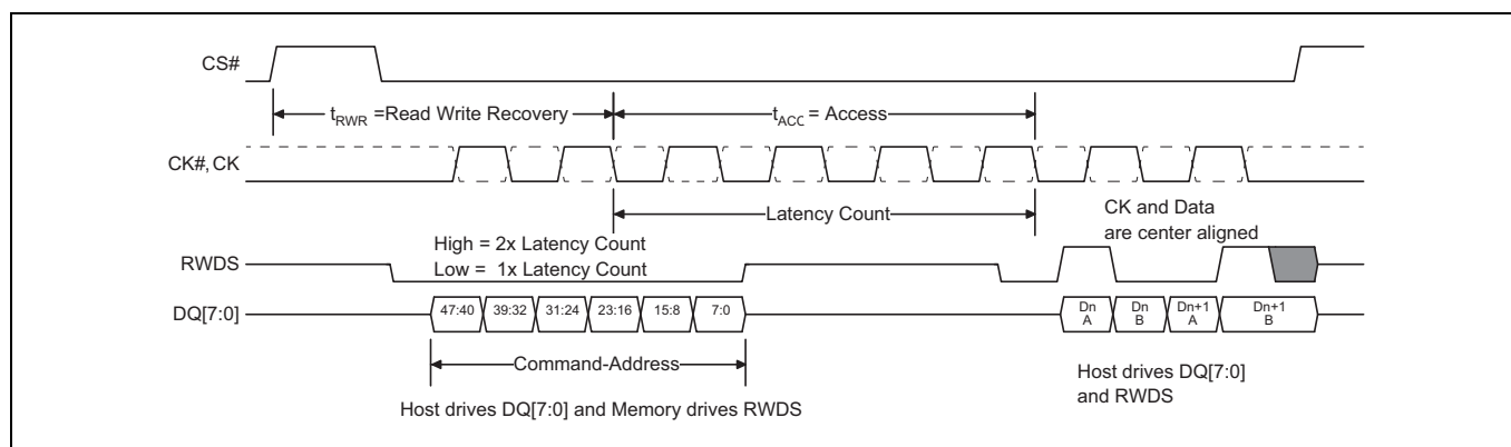
Figure 1-3 Write Transaction, Single Initial Latency Count
