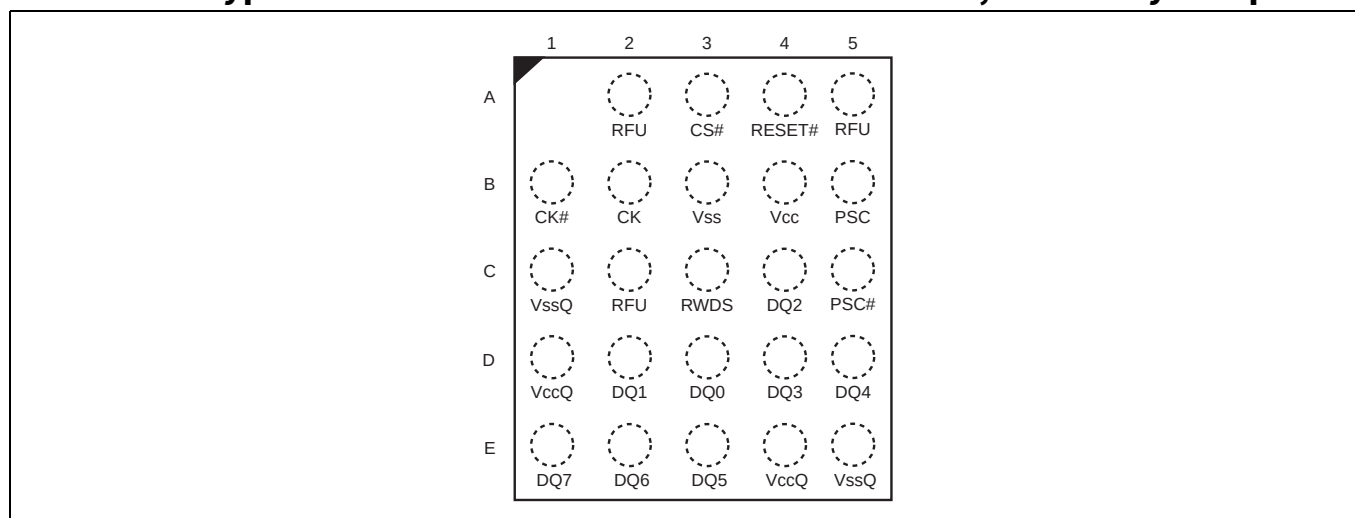
Figure 12-2 24-ball FBGA, 5 x 5 Ball Footprint, Top View
