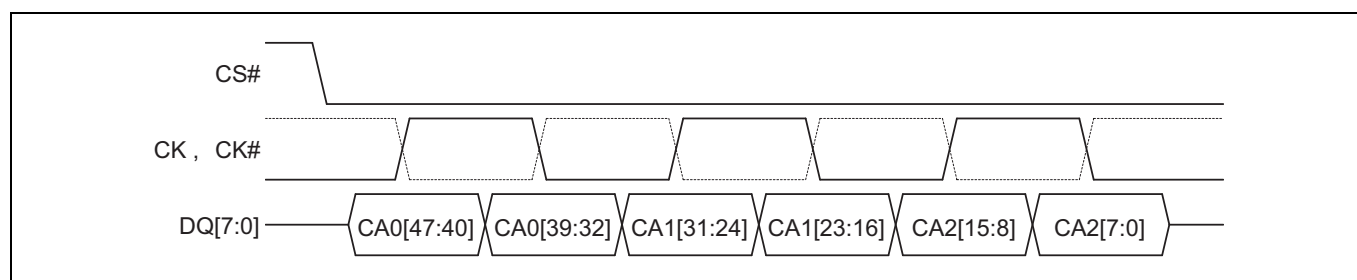
Figure 4-1 Command-Address (CA) Sequence [4, 5, 6, 7]
