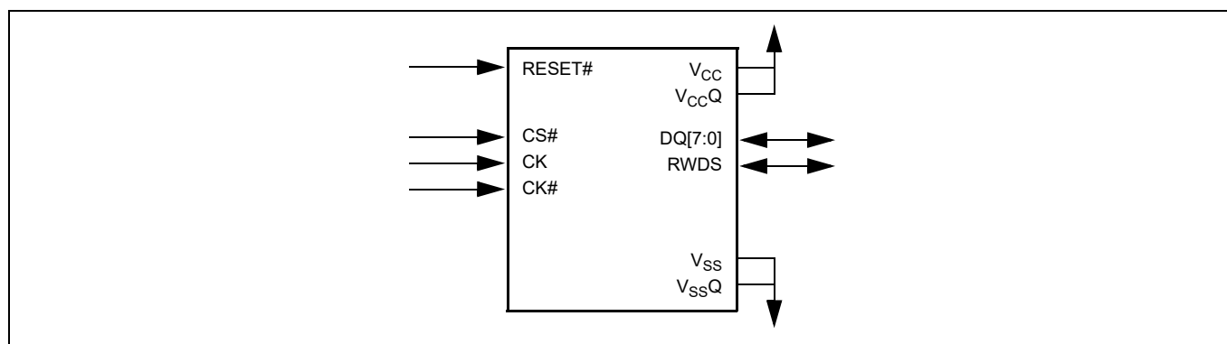
Figure 2-1 HyperRAM Interface [1]
