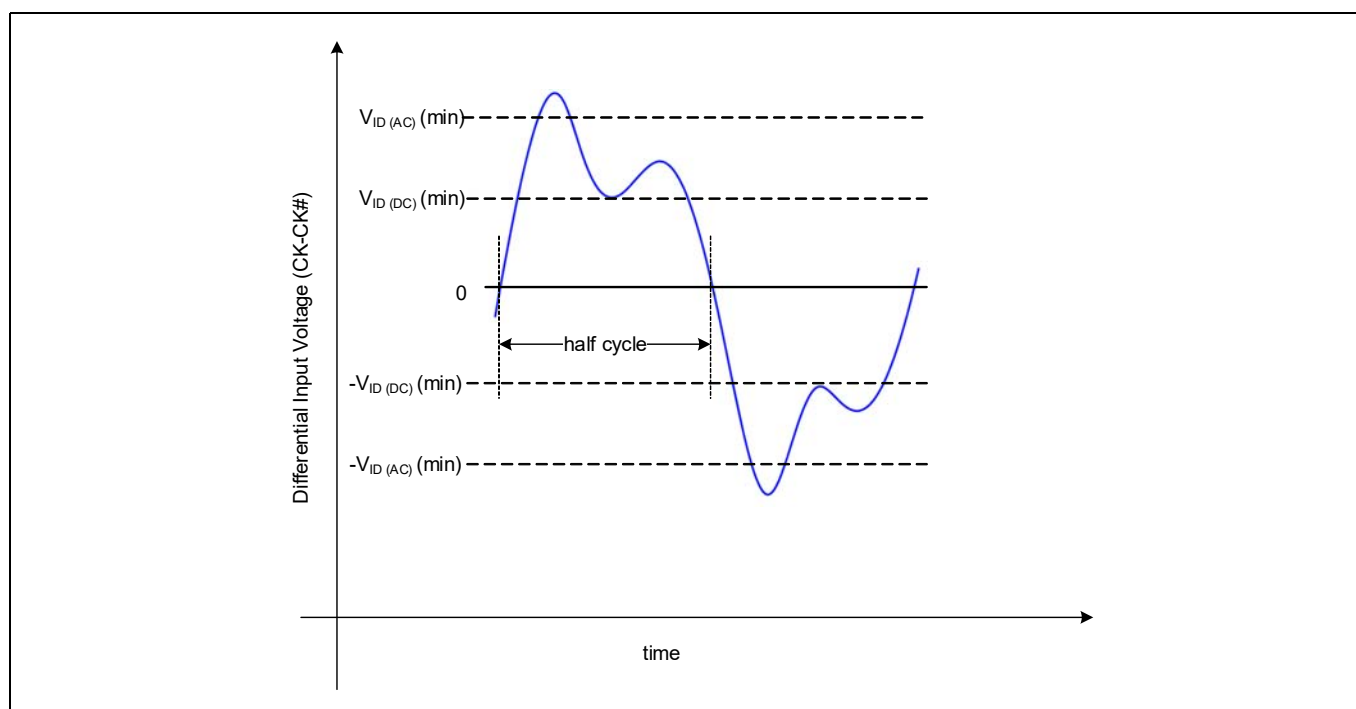
Figure 10-4 Differential Clock (CK/CK#) Input Swing
