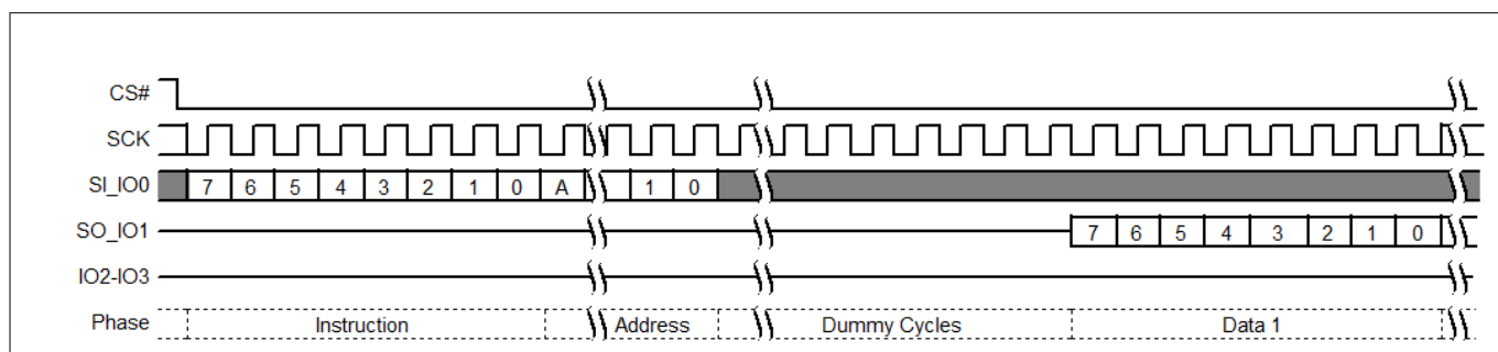
Figure 66 Fast Read (FAST_READ) command sequence
