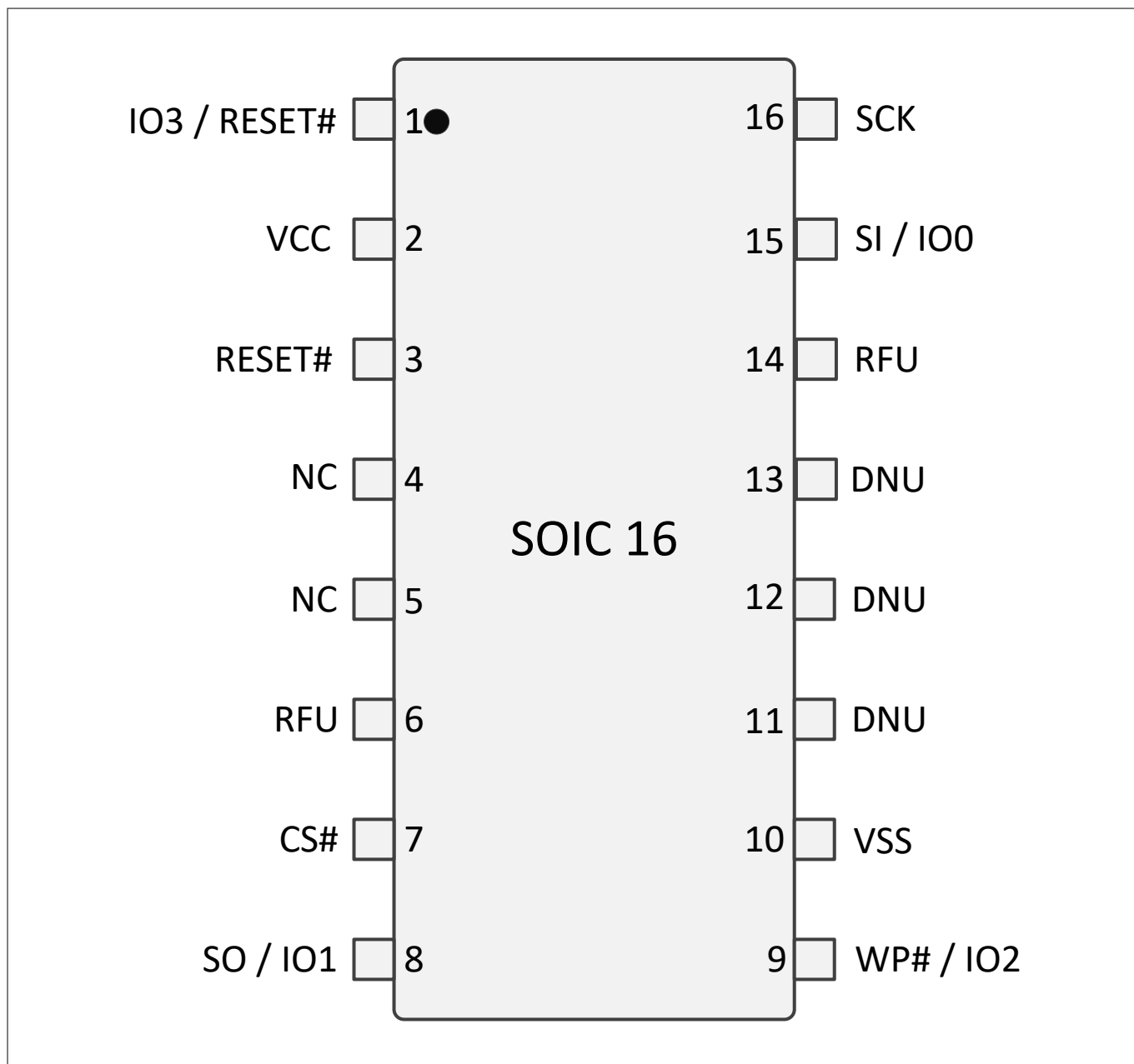
Figure 1 16-lead SOIC package (SO3016), top view
