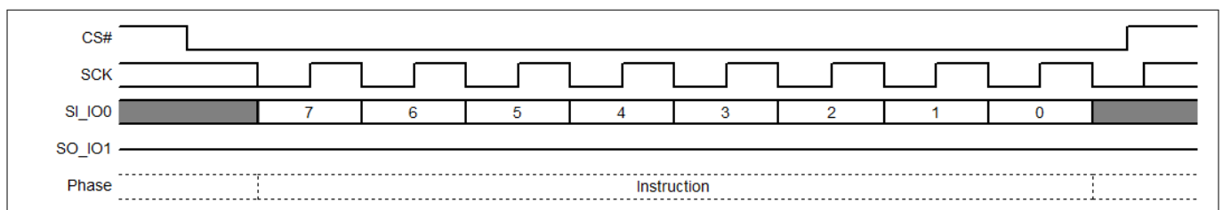
Figure 88 Program or Erase Suspend command sequence
