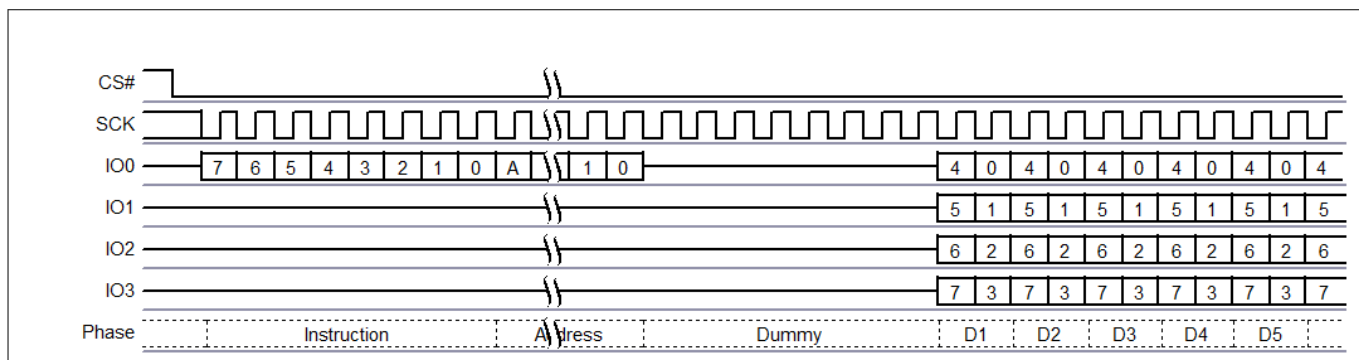
Figure 68 Quad Output Read command sequence
