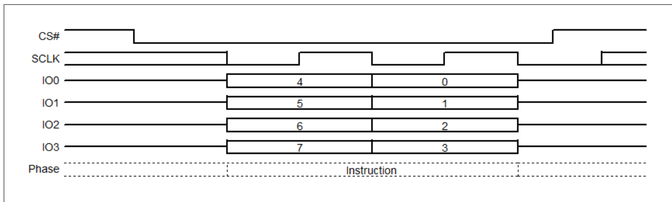
Figure 64 Exit QPI (QPIEX F5h) command sequence
