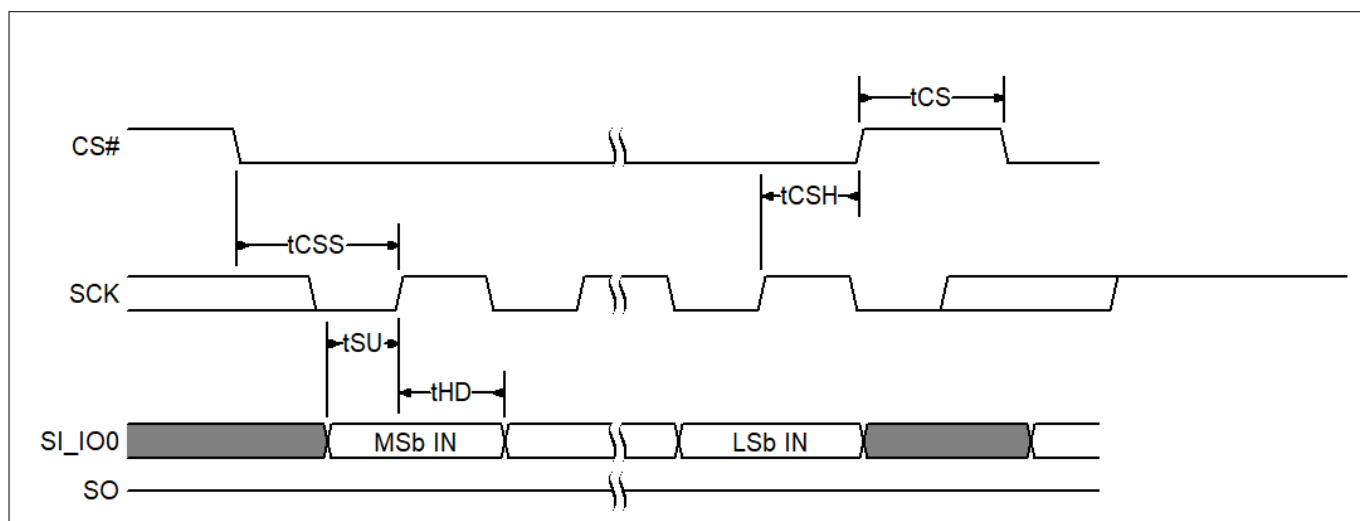
Figure 143 SPI single bit input timing
