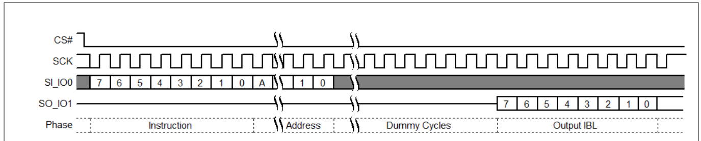
Figure 97 IBL command sequence
