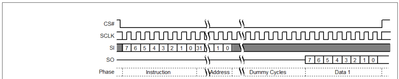
Figure 16 Single Bit Wide I/O command with latency
