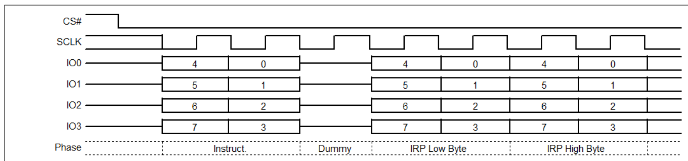
Figure 108 IRPRD command sequence – QPI mode
