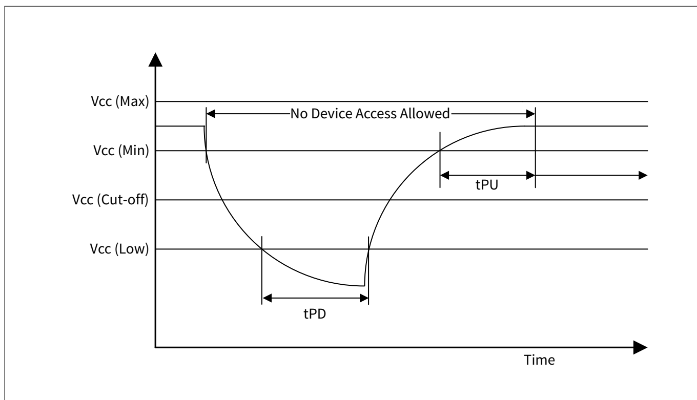
Figure 132 Power-down and voltage drop
