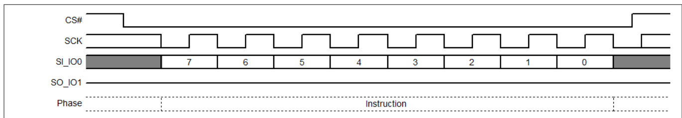
Figure 47 Clear Status Register (CLSR) command sequence
