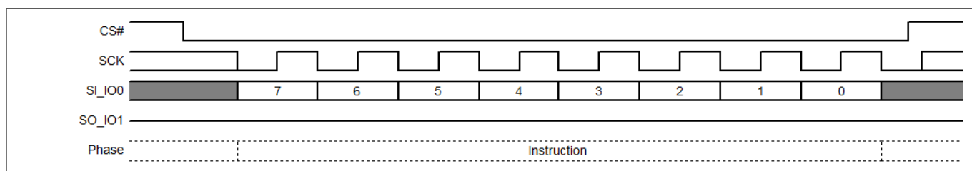
Figure 63 Enter QPI Mode (QPIEN 38h) command sequence
