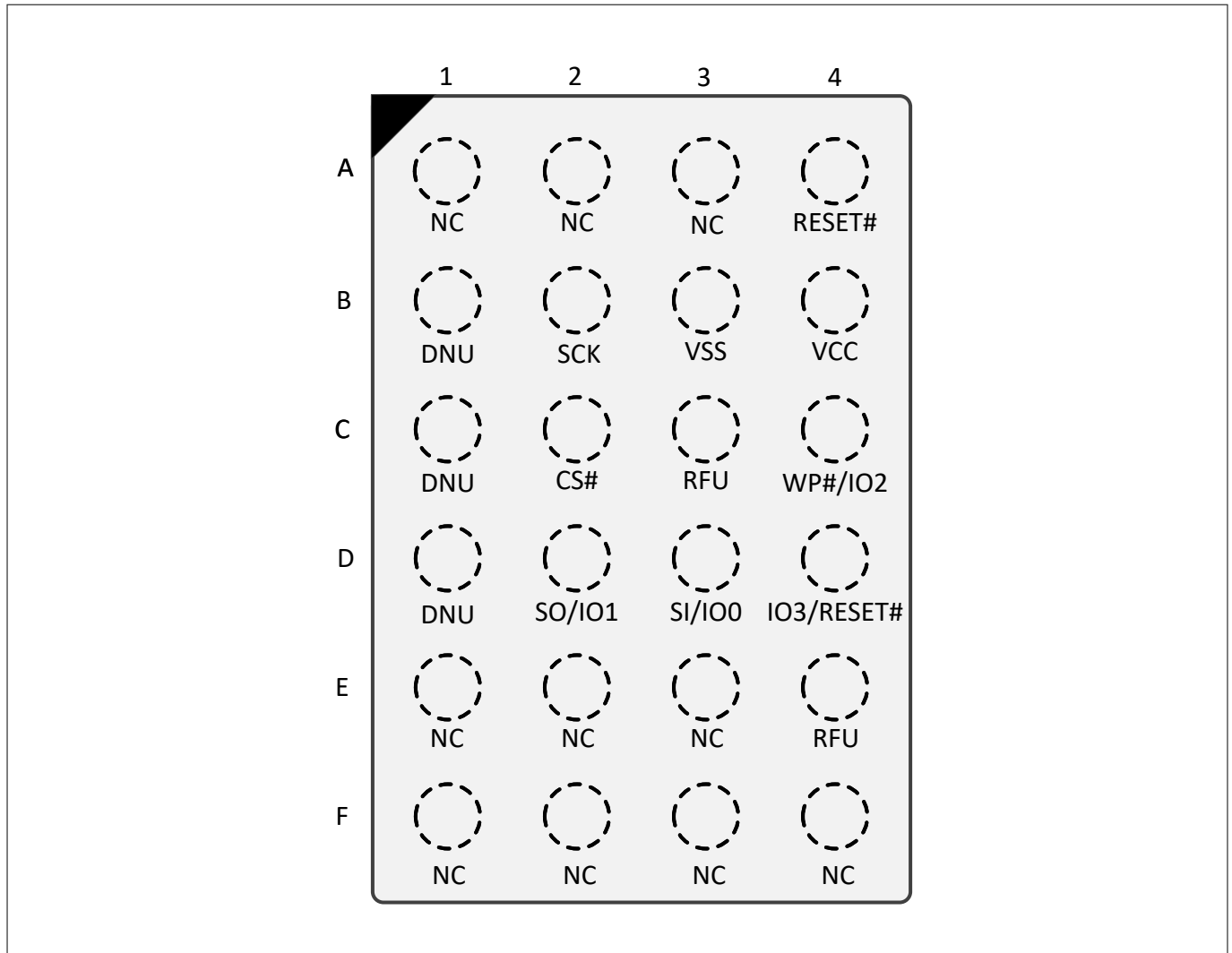
Figure 5 24-ball BGA, 4 x 6 ball footprint (FAC024), top view
