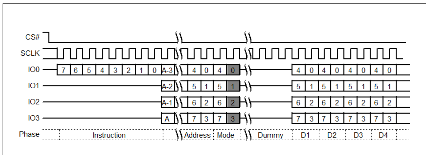
Figure 71 Quad I/O Read initial access command sequence
