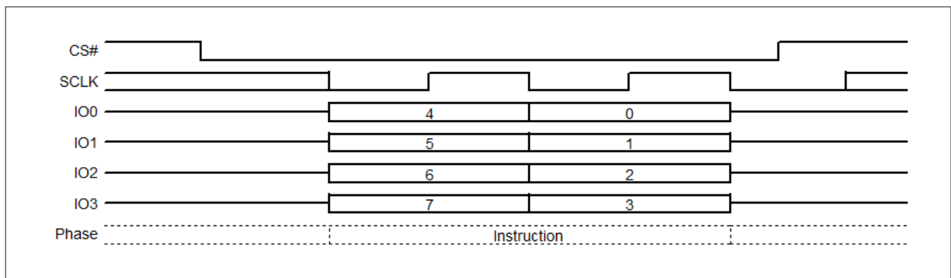
Figure 124 Deep Power Down (DPD) command sequence – QPI mode
