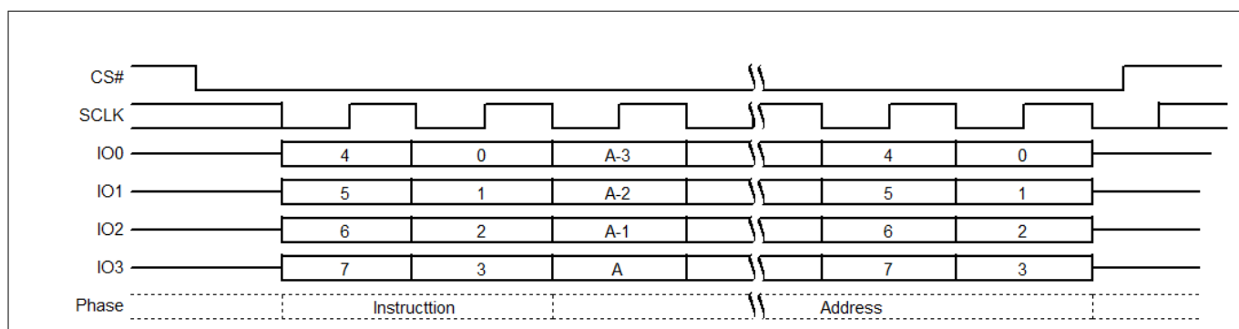
Figure 85 Block Erase (BE D8h or 4BE DCh) QPI mode command sequence
