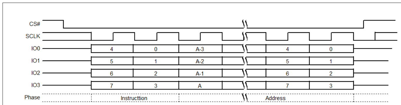
Figure 83 Half Block Erase (HBE 52h or 4HBE 53h) QPI mode command sequence
