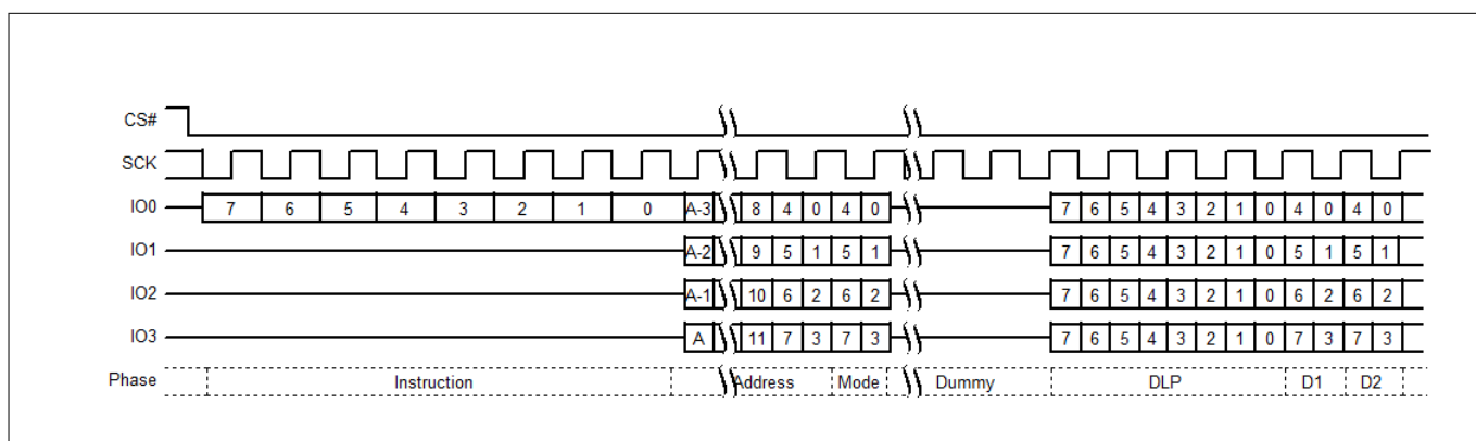
Figure 74 DDR Quad I/O Read initial access
