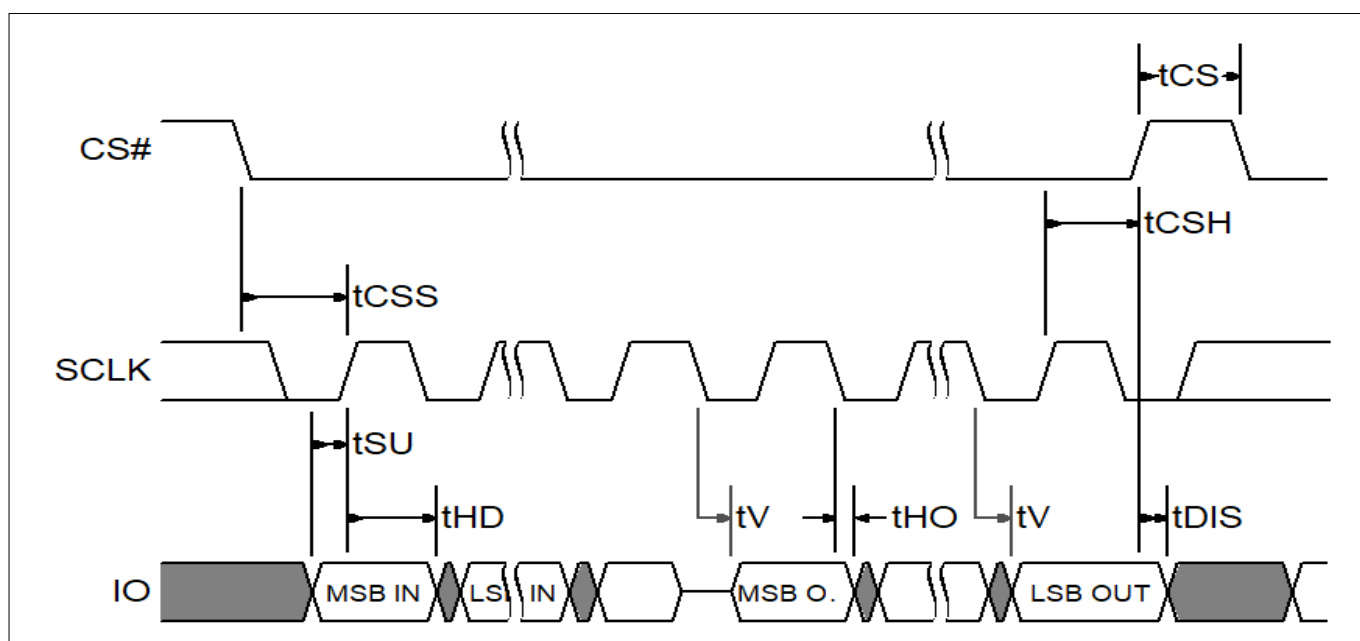
Figure 145 SDR MIO timing
