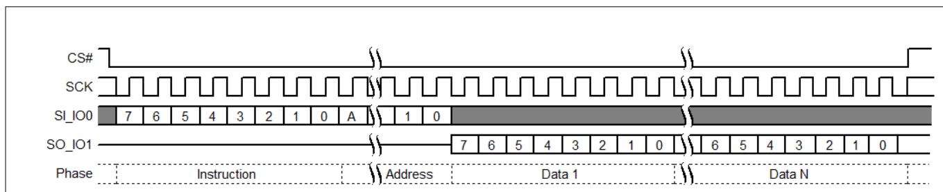
Figure 65 Read command sequence
