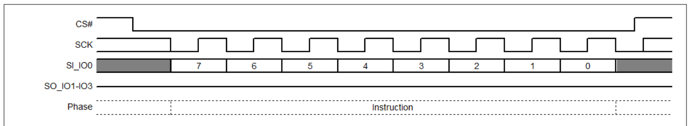
Figure 13 Standalone Instruction command
