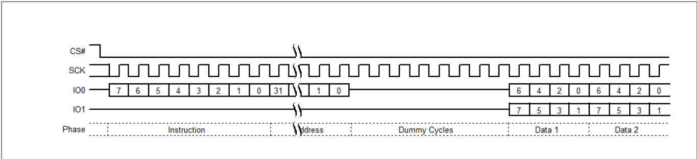
Figure 17 Dual Output Read command
