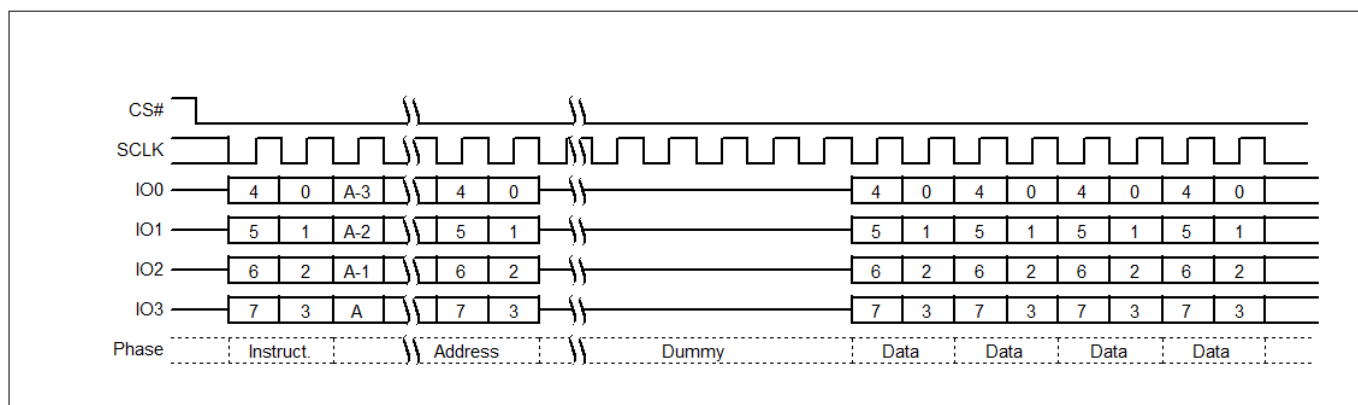
Figure 60 Read Any Register, QPI mode, command sequence
