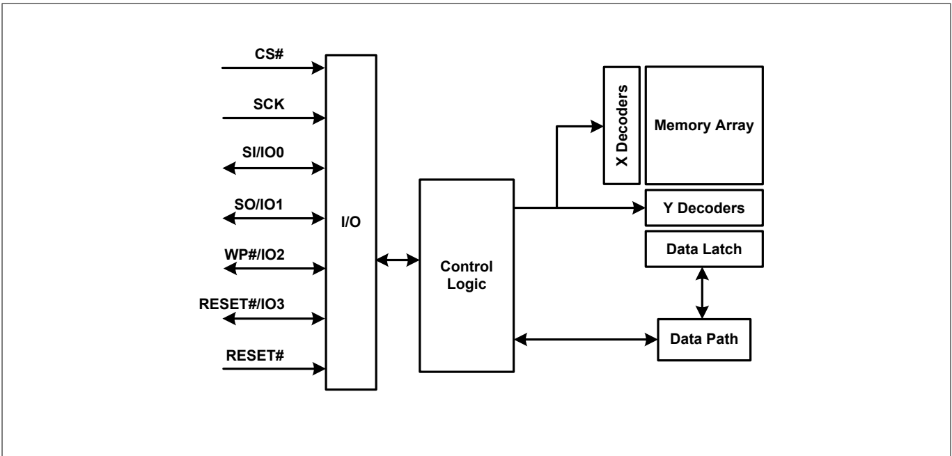
Figure 6 Logic block diagram
