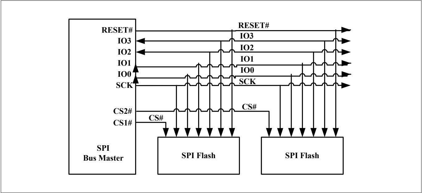
Figure 9 Bus master and memory devices on the SPI bus - quad bit data path - Separate RESET#
