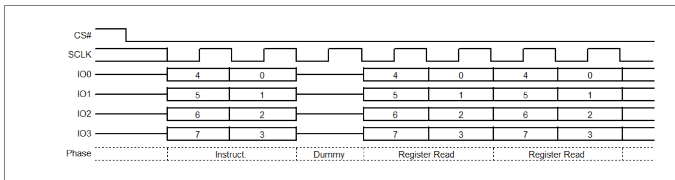
Figure 54 DLP Read (DLPRD) command sequence – QPI mode
