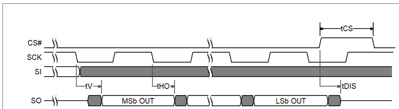
Figure 144 SPI single bit output timing
