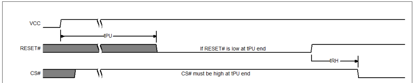
Figure 136 Reset low at the end of POR
