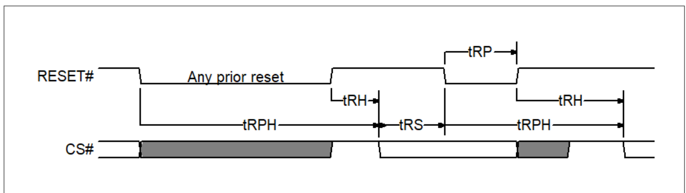
Figure 139 Hardware reset using RESET# input
