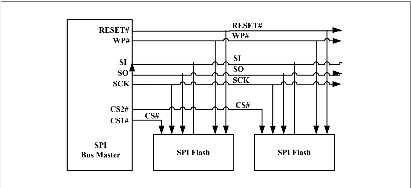
Figure 7 Bus master and memory devices on the SPI bus - single bit data path
