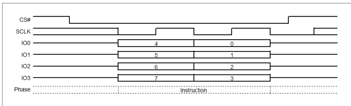
Figure 87 Chip Erase command sequence QPI mode
