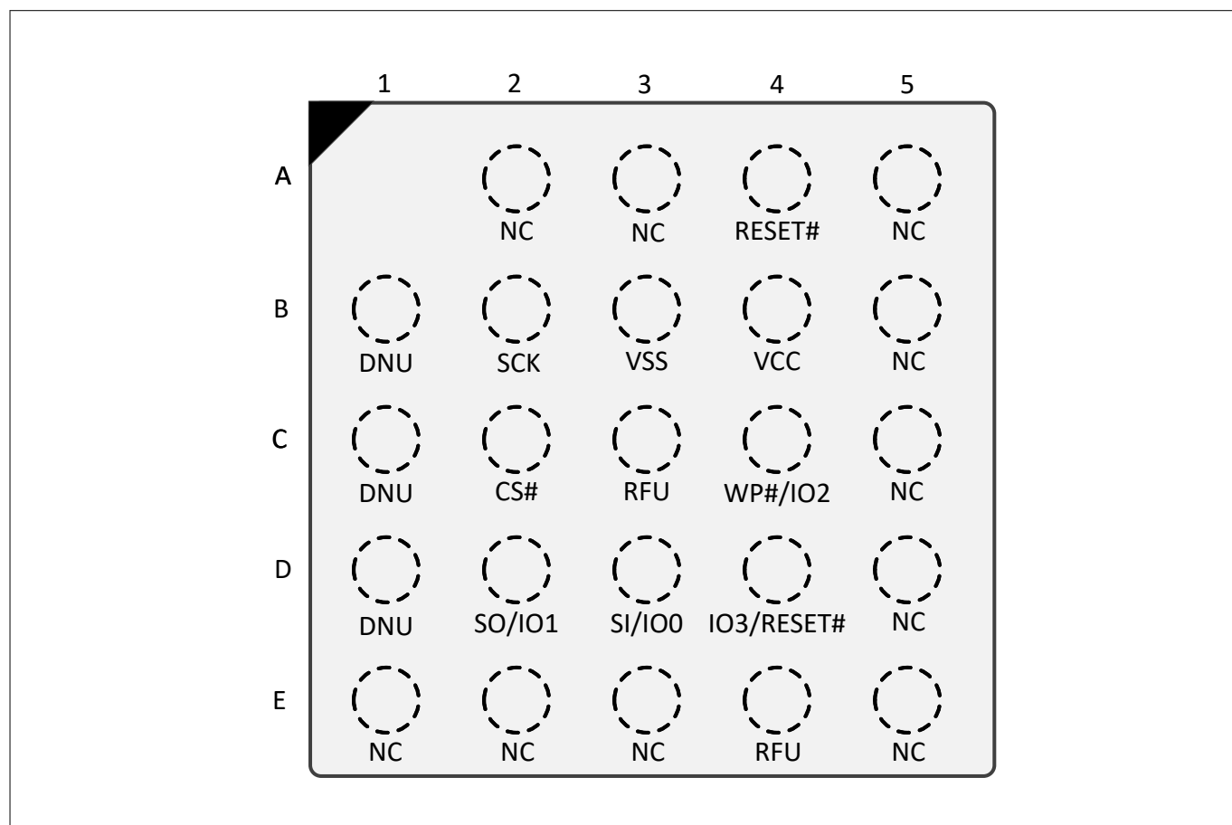
Figure 4 24-ball BGA, 5 x 5 ball footprint (FAB024), top view
