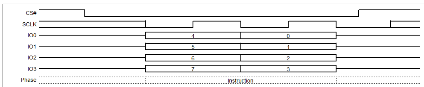
Figure 56 Enter 4 Byte Address QPI mode
