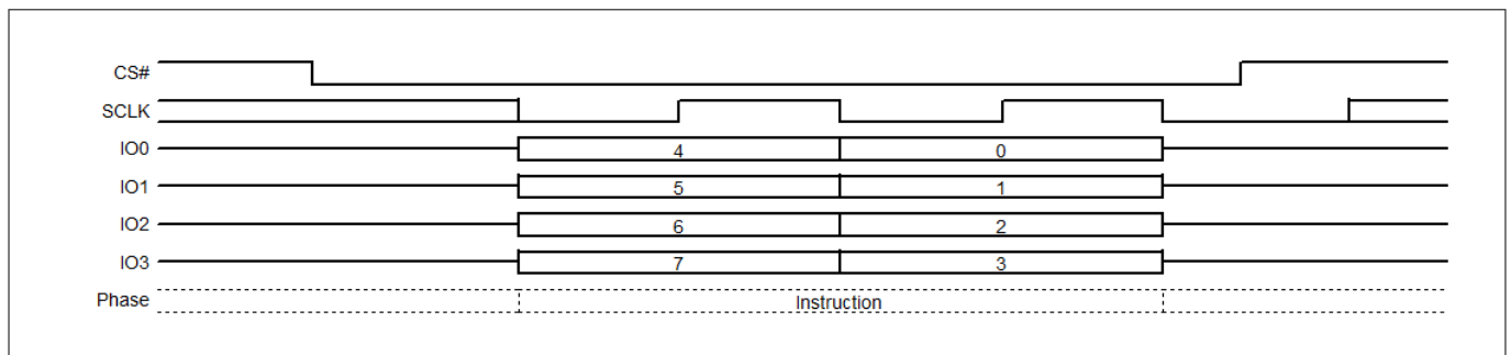
Figure 42 Write Enable (WREN) command sequence QPI mode
