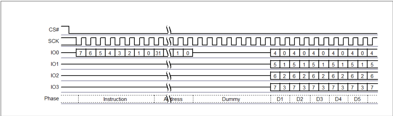
Figure 18 Quad Output Read command
