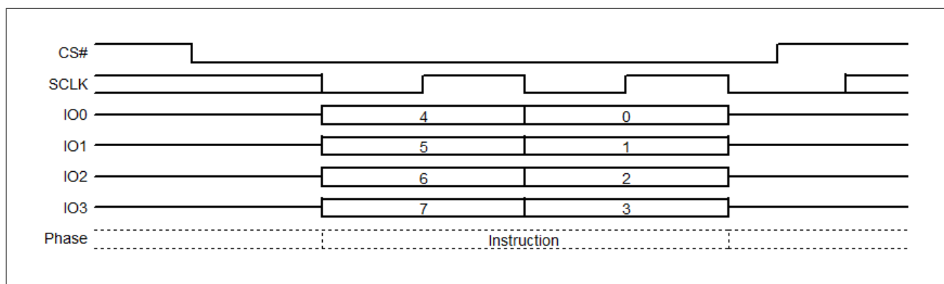
Figure 89 Program or Erase Suspend command sequence QPI mode
