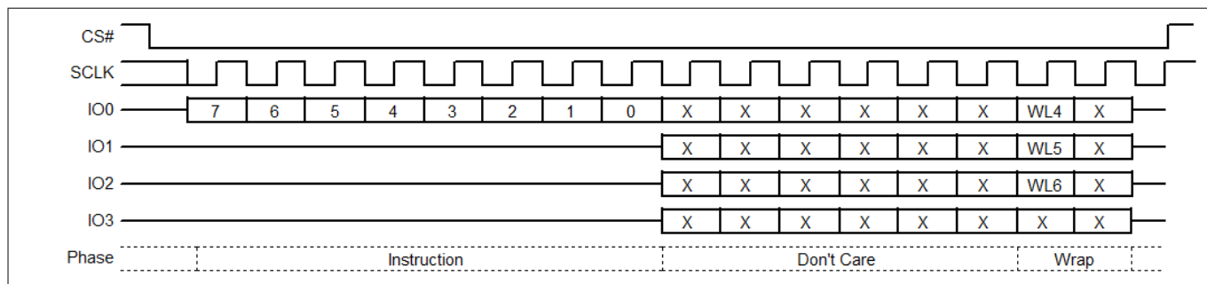
Figure 61 Set Burst Length command sequence quad I/O mode
