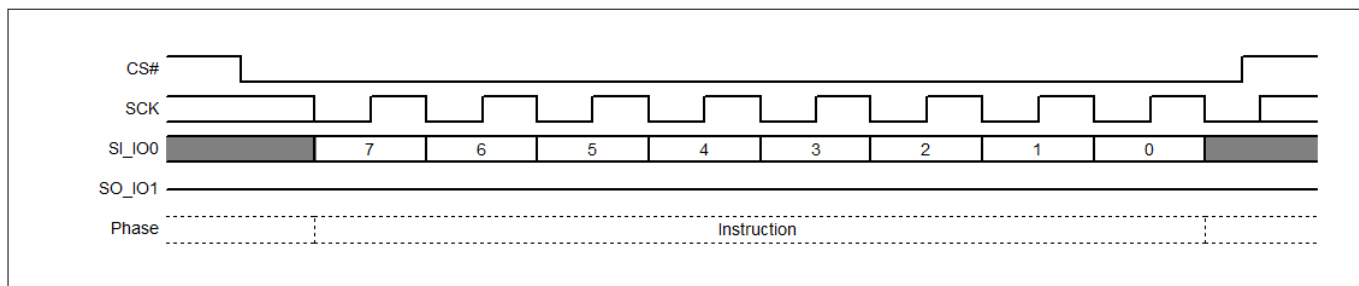
Figure 91 Erase or Program Resume command sequence
