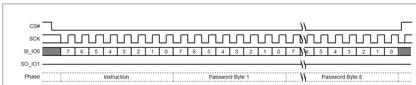
Figure 119 Password Unlock (PASSU) command sequence
