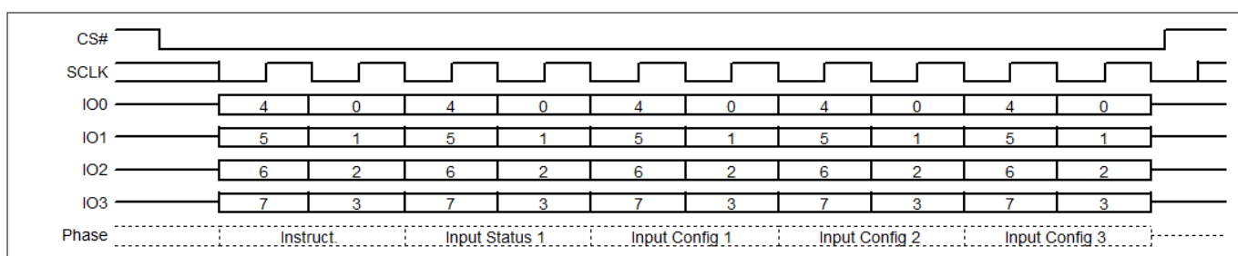
Figure 40 Write Register (WRR) command sequence QPI mode
