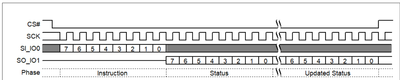
Figure 35 Read Status Register 1 (RDSR1) command sequence
