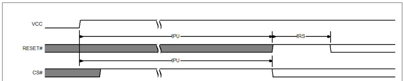
Figure 138 POR followed by hardware reset
