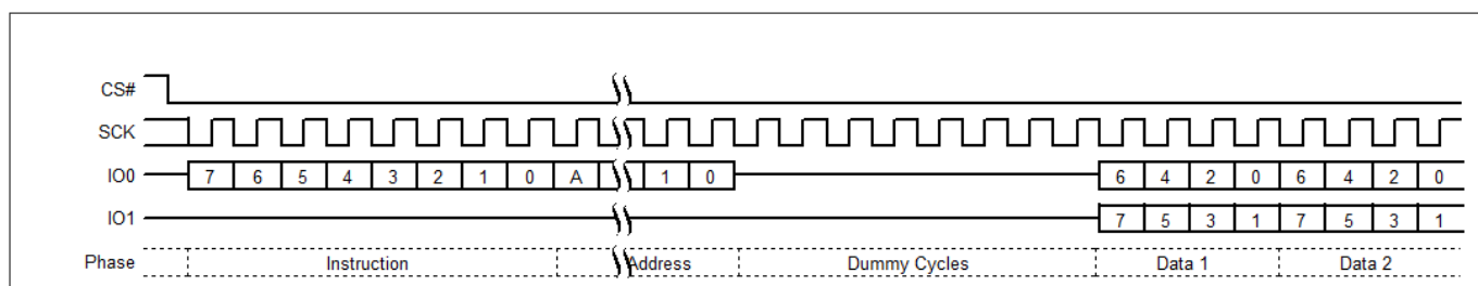
Figure 67 Dual Output Read command sequence
