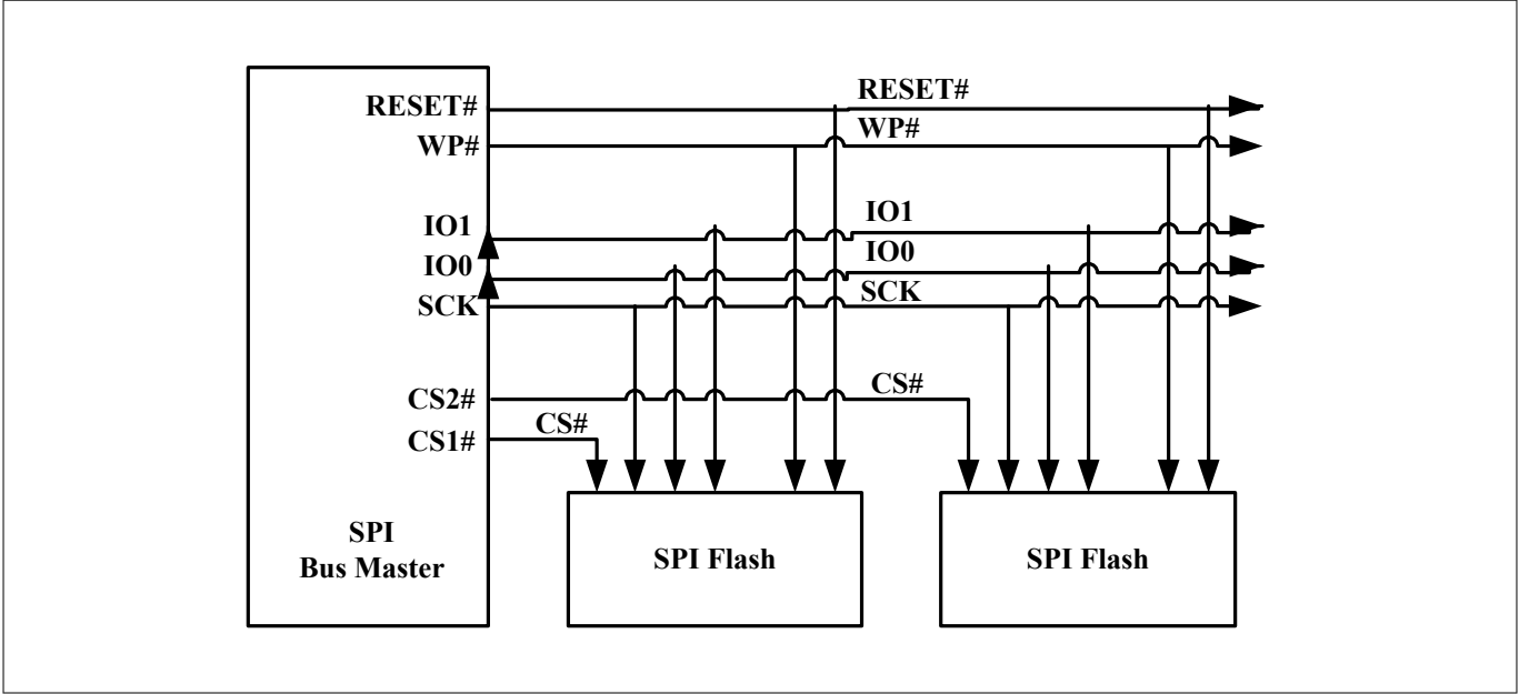
Figure 8 Bus master and memory devices on the SPI bus - dual bit data path
