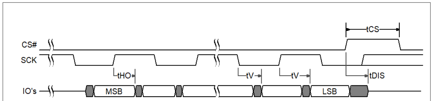
Figure 148 SPI DDR output timing
