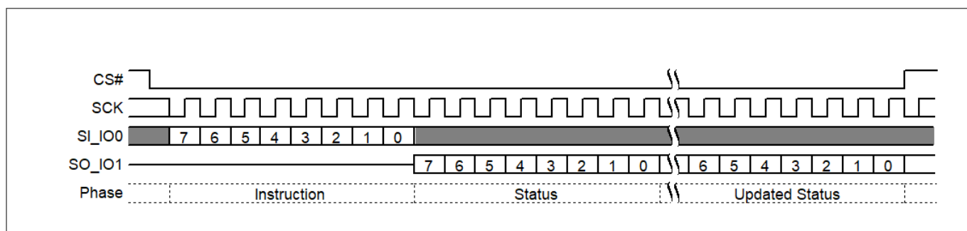
Figure 37 Read Status Register 2 (RDSR2) Command
