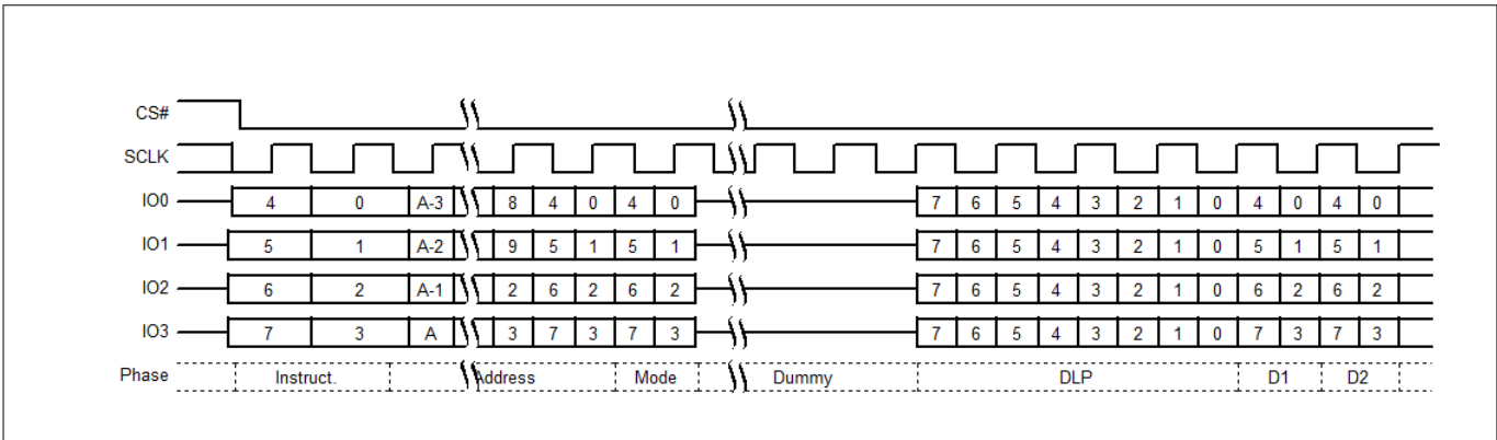
Figure 23 DDR Quad I/O Read command QPI mode
