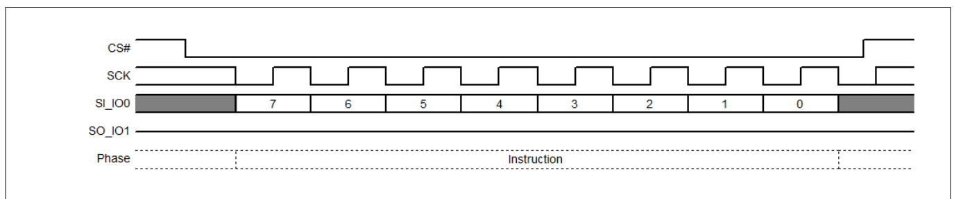
Figure 41 Write Enable (WREN) command sequence
