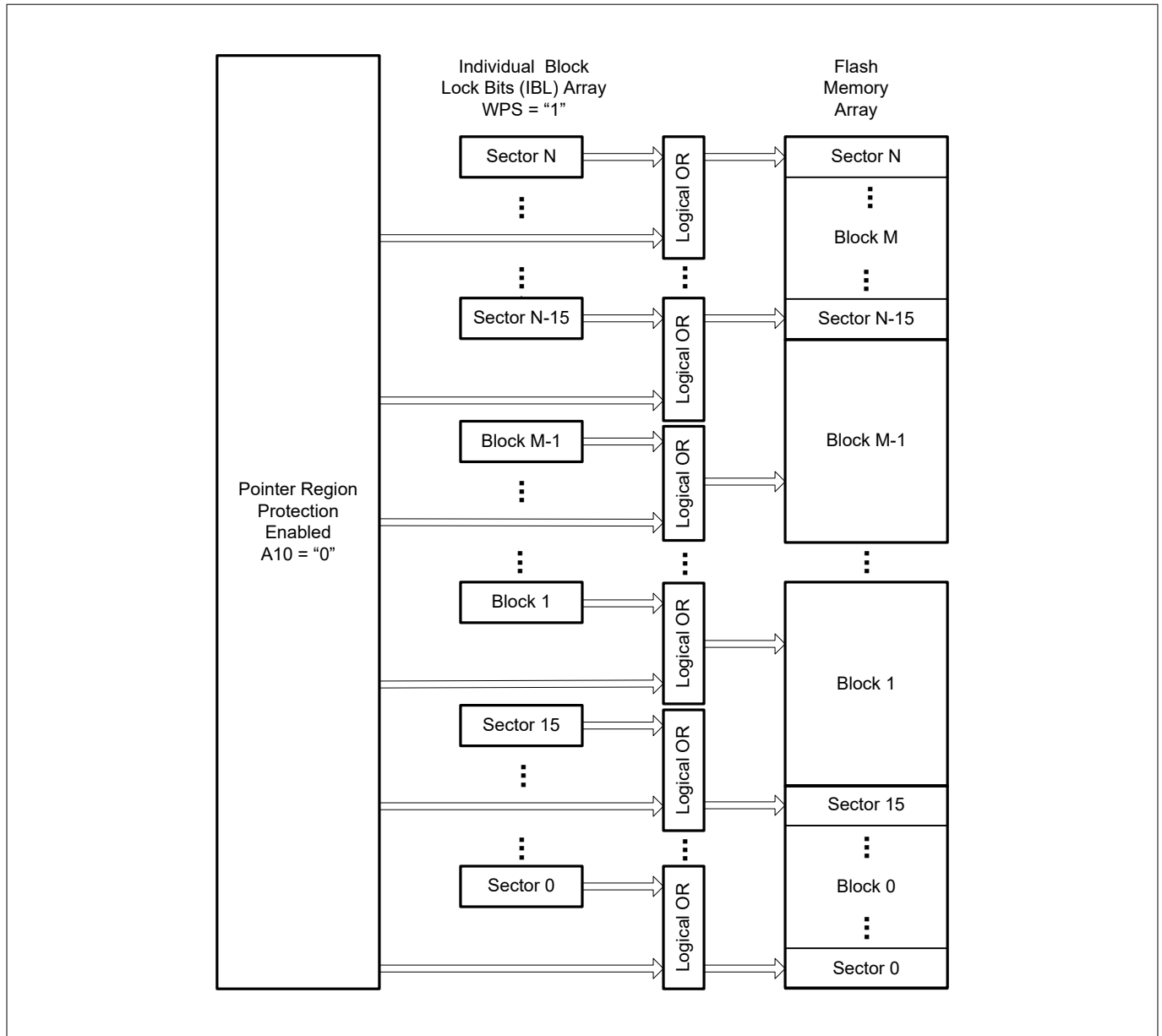
Figure 25 Individual block lock / pointer region protection control
