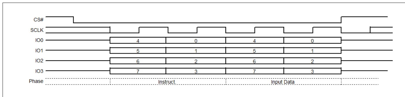
Figure 52 Write DLRV (WDLRV) command sequence – QPI mode
