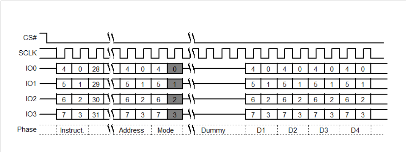
Figure 21 Quad I/O Read command in QPI mode
