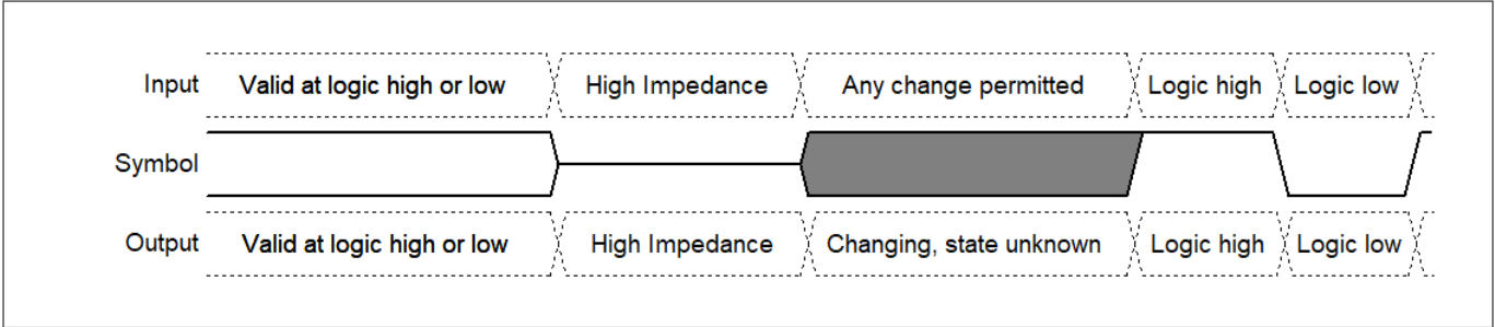
Figure 133 Waveform element meanings
