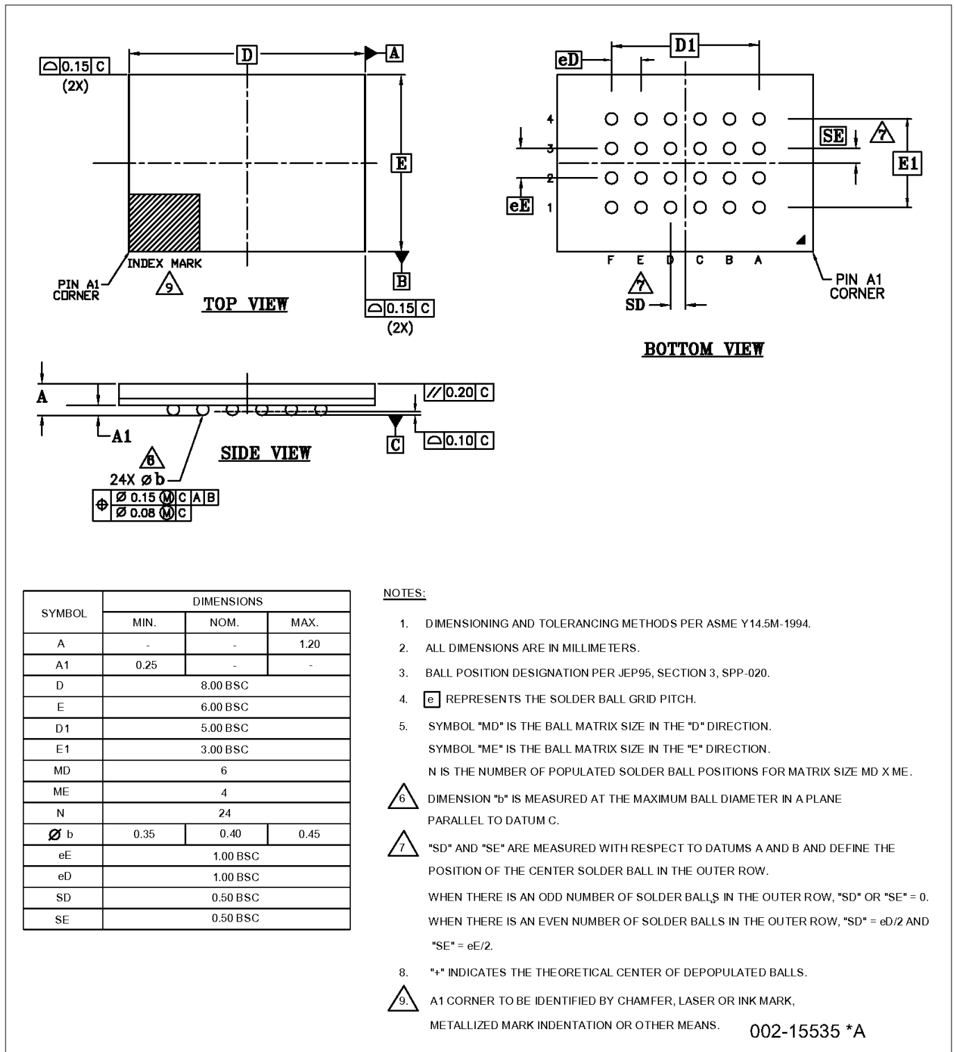
Figure 156 24-ball FBGA (8 x 6 x 1.2 mm) package outline (PG-TFBGA-24), 002-15535
