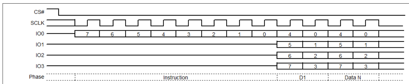
Figure 30 Read Quad Identification (RDQID) command sequence quad mode
