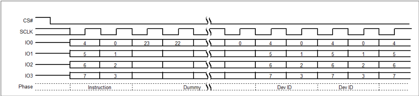
Figure 128 Read Identification (RES) QPI mode command
