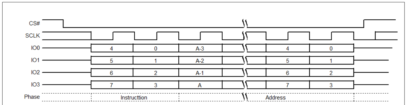
Figure 98 IBL command sequence QPI mode
