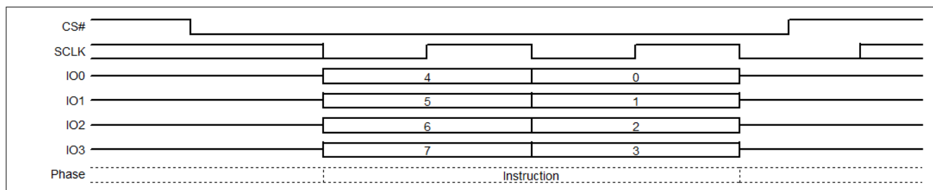
Figure 126 Release from Deep Power Down (RES) command sequence – QPI mode
