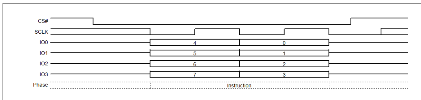
Figure 58 Exit 4 Byte Address QPI mode
