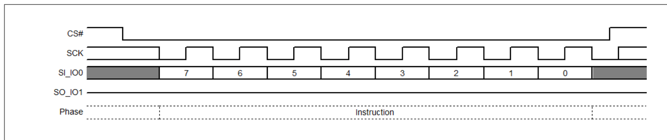
Figure 43 Write Disable (WRDI) command sequence
