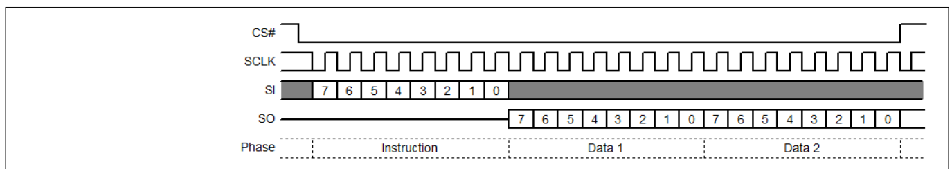
Figure 15 Single Bit Wide Output command without latency
