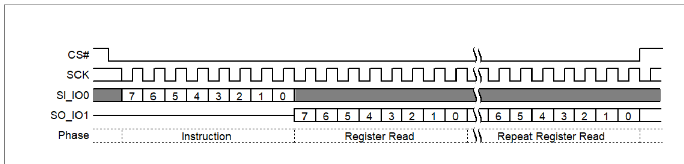
Figure 38 Read Configuration Register (RDCR1) (RDCR2) (RDCR3) command sequence
