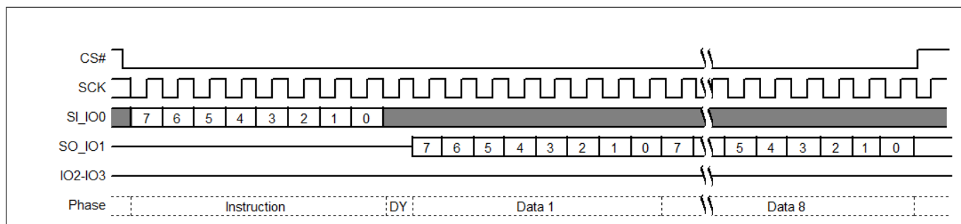
Figure 115 Password Read (PASSRD) command sequence
