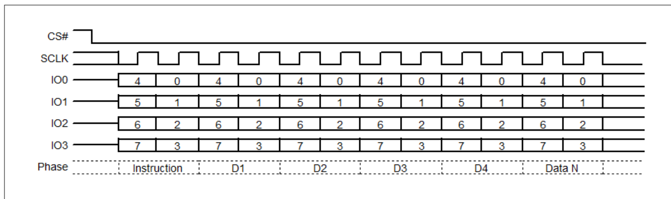
Figure 29 Read Quad Identification (RDQID) command sequence QPI mode
