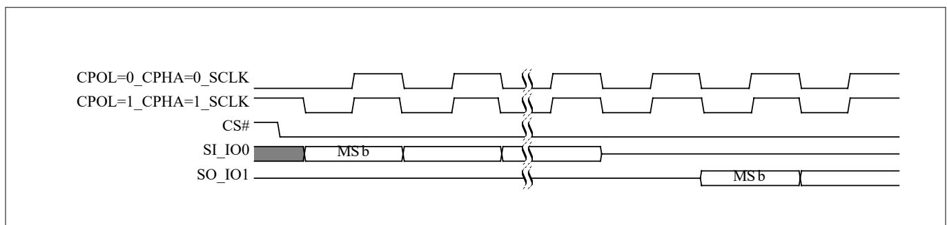
Figure 11 SPI SDR modes supported
