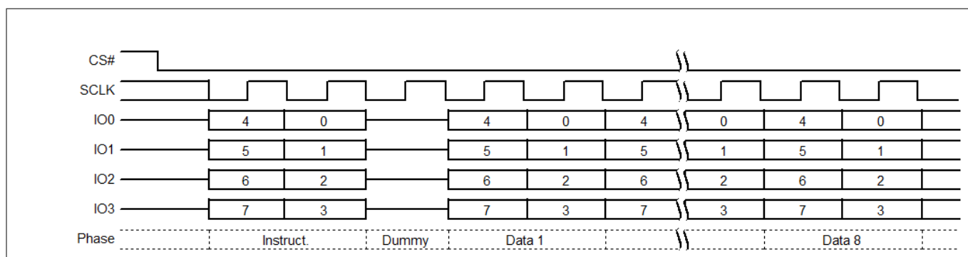
Figure 116 Password Read (PASSRD) command sequence – QPI mode
