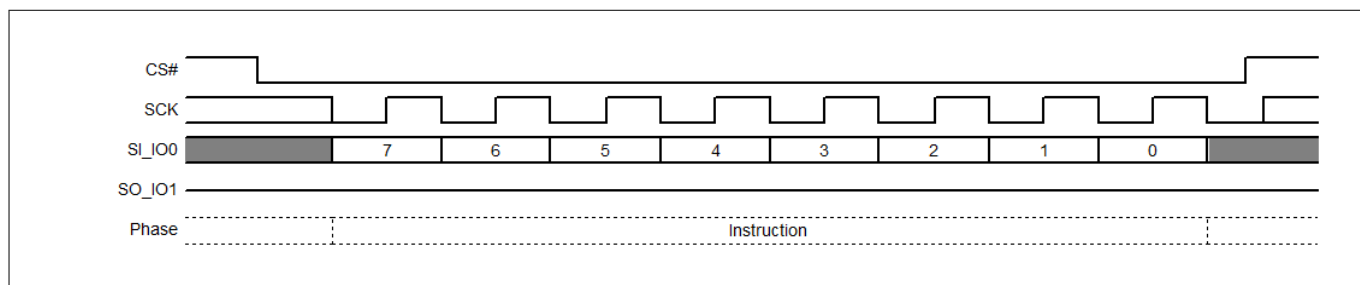
Figure 45 Write Enable for Volatile Registers (WRENV) command sequence
