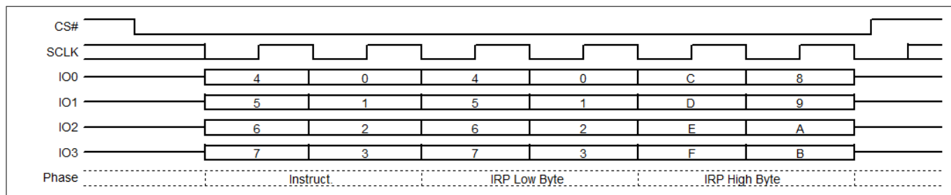
Figure 110 IRP Program (IRPP) command QPI
