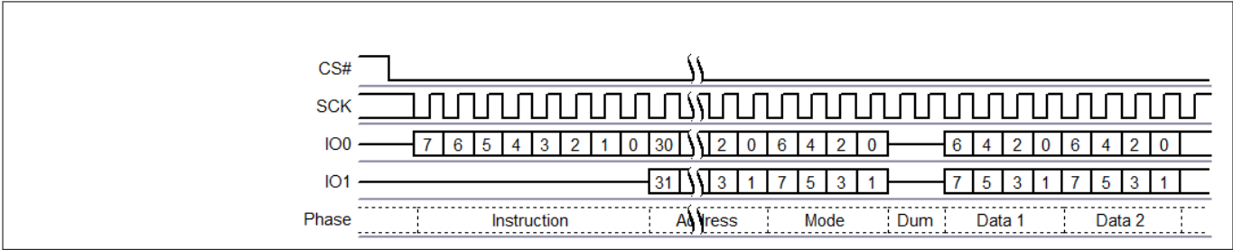
Figure 19 Dual I/O command
