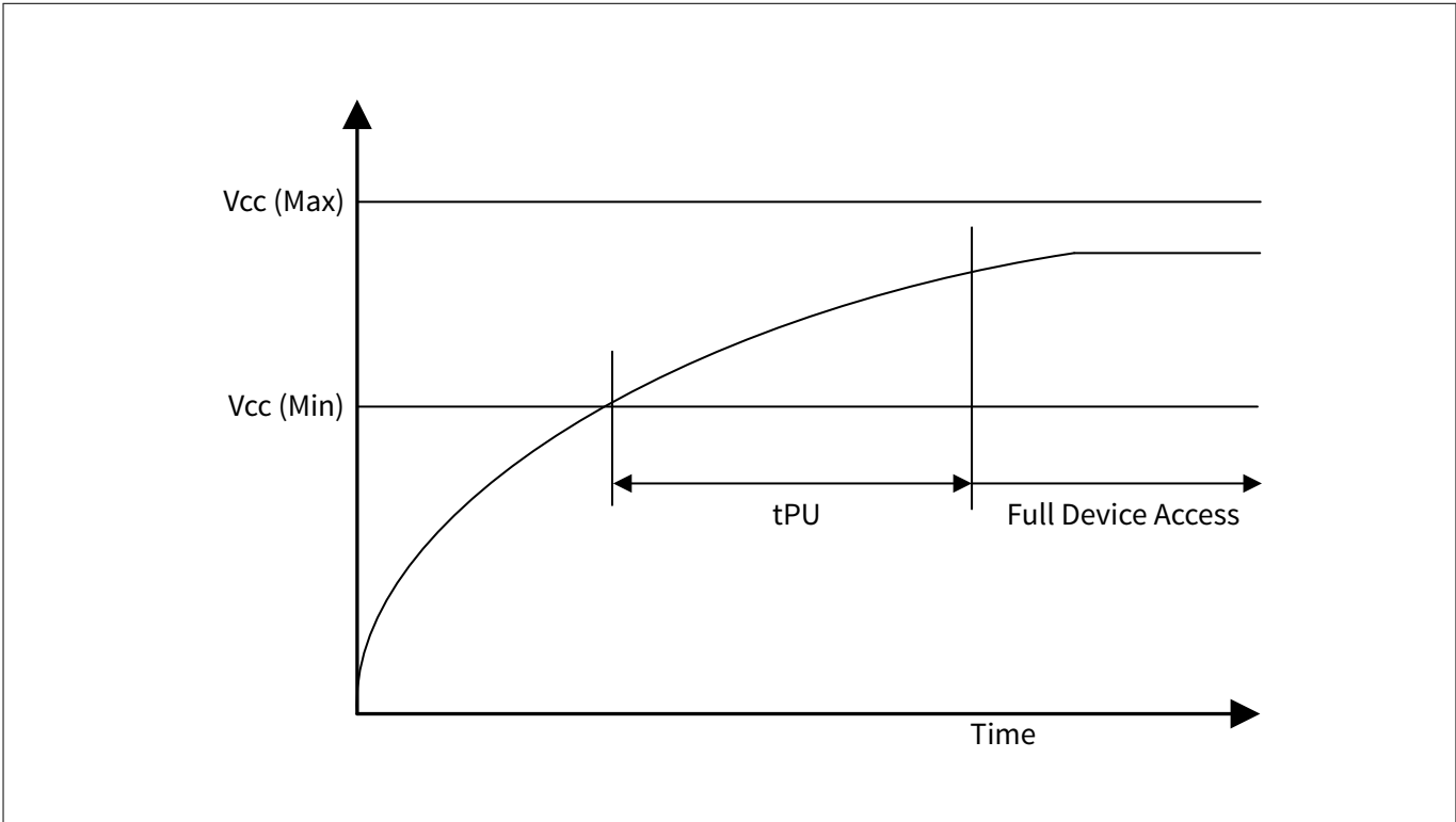
Figure 131 Power-up
