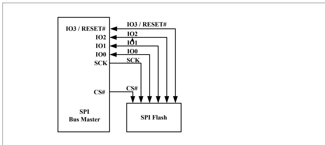
Figure 10 Bus master and memory devices on the SPI bus - quad bit data path - I/O3 / RESET#
