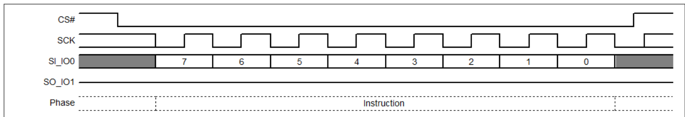
Figure 123 Deep Power Down (DPD) command sequence
