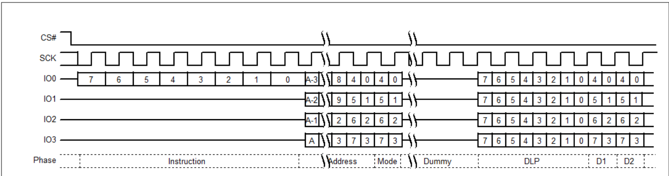
Figure 22 DDR Quad I/O Read command
