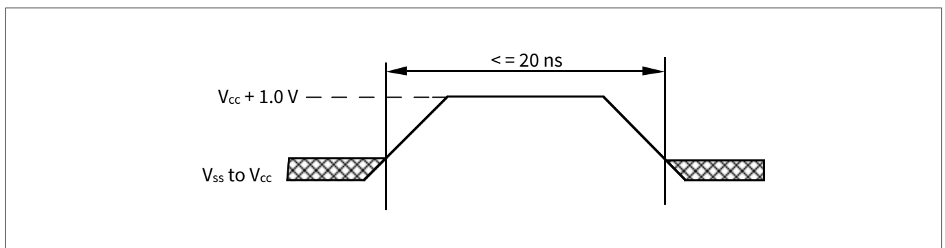
Figure 130 Maximum positive overshoot waveform
