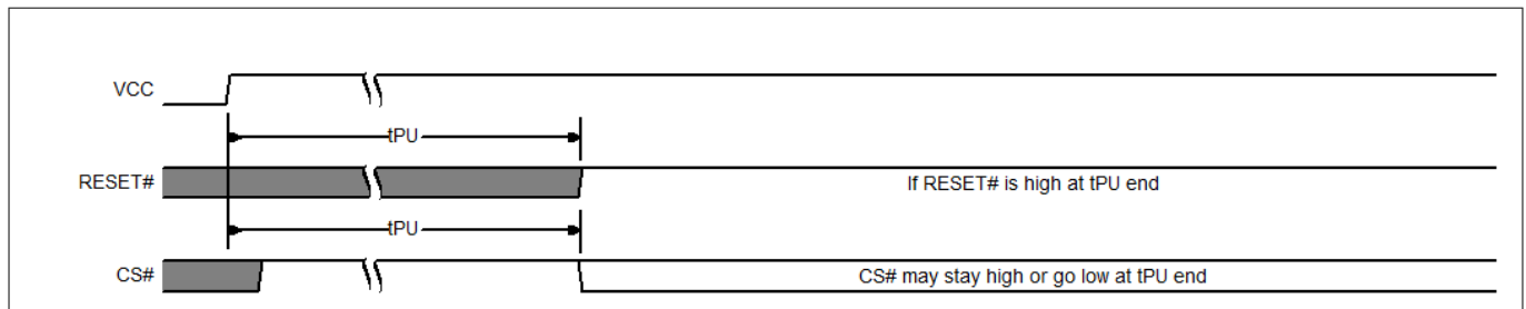
Figure 137 Reset high at the end of POR
