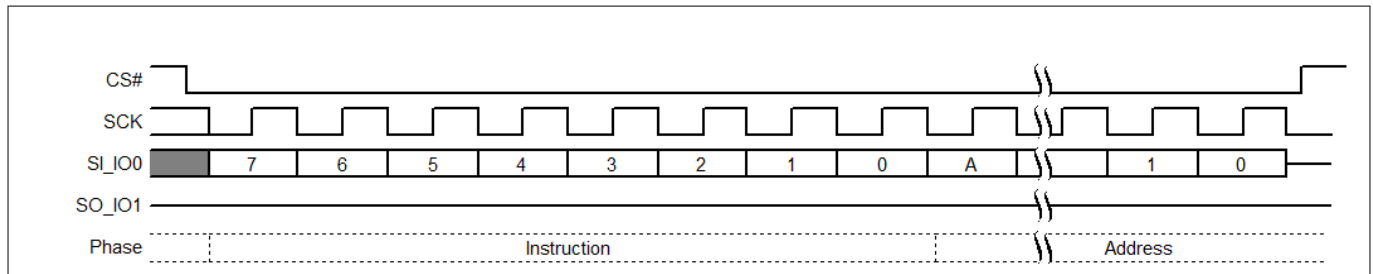
Figure 80 Sector Erase (SE 20h or 4SE 21h) command sequence
