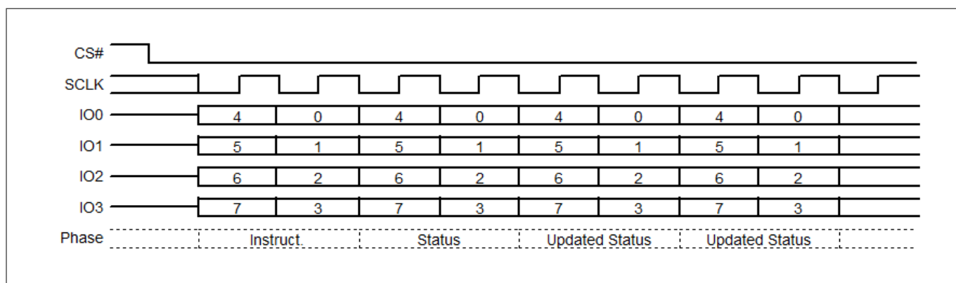
Figure 36 Read Status Register 1 (RDSR1) QPI Mode Command
