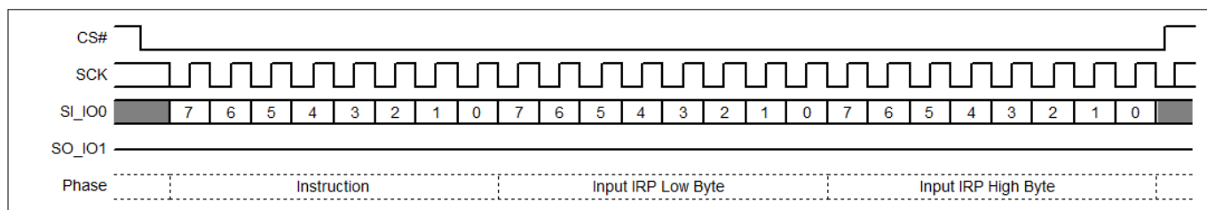
Figure 109 IRP Program (IRPP) command
