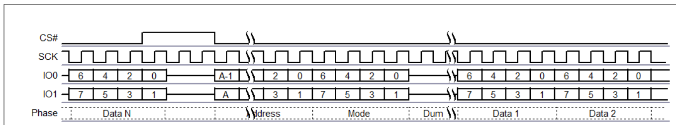
Figure 70 Dual I/O Continuous Read command sequence
