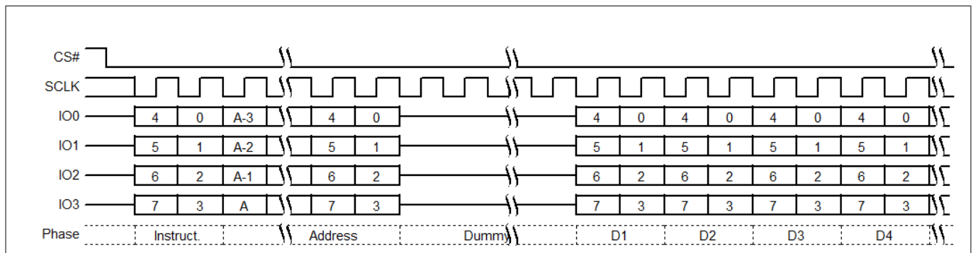
Figure 94 Security Regions Read command sequence QPI mode
