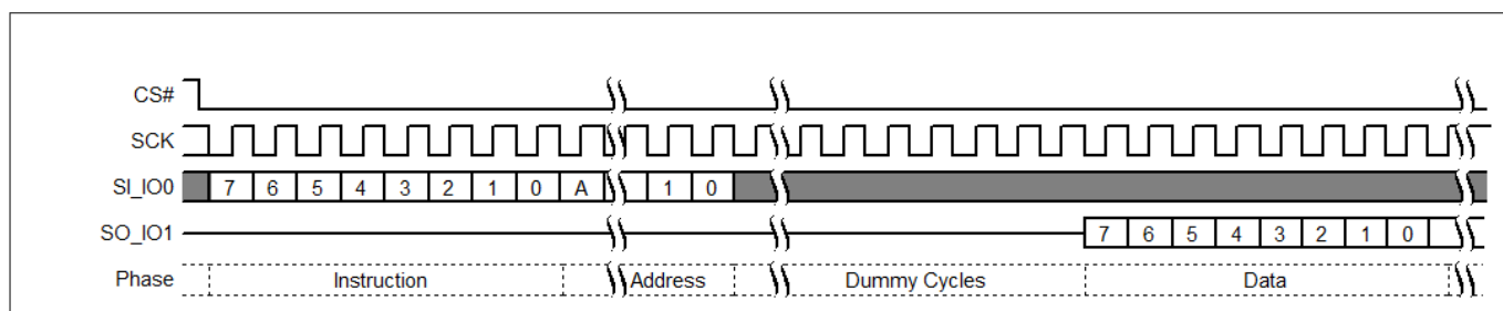
Figure 59 Read Any Register Read command sequence
