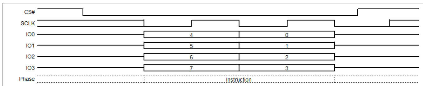
Figure 114 Protection Register Lock (PRL) command sequence – QPI mode
