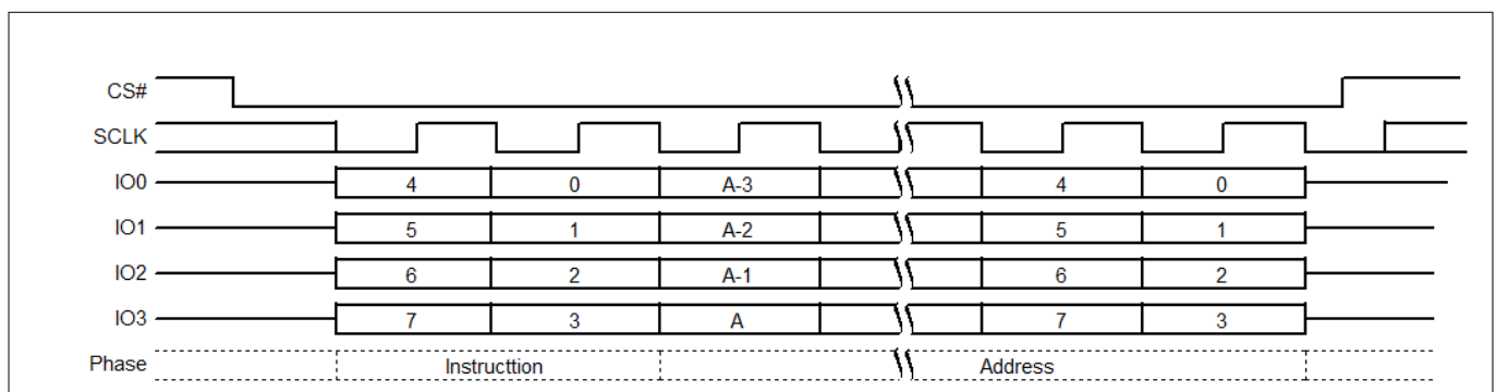
Figure 81 Sector Erase (SE 20h or 4SE 21h) QPI mode command sequence
