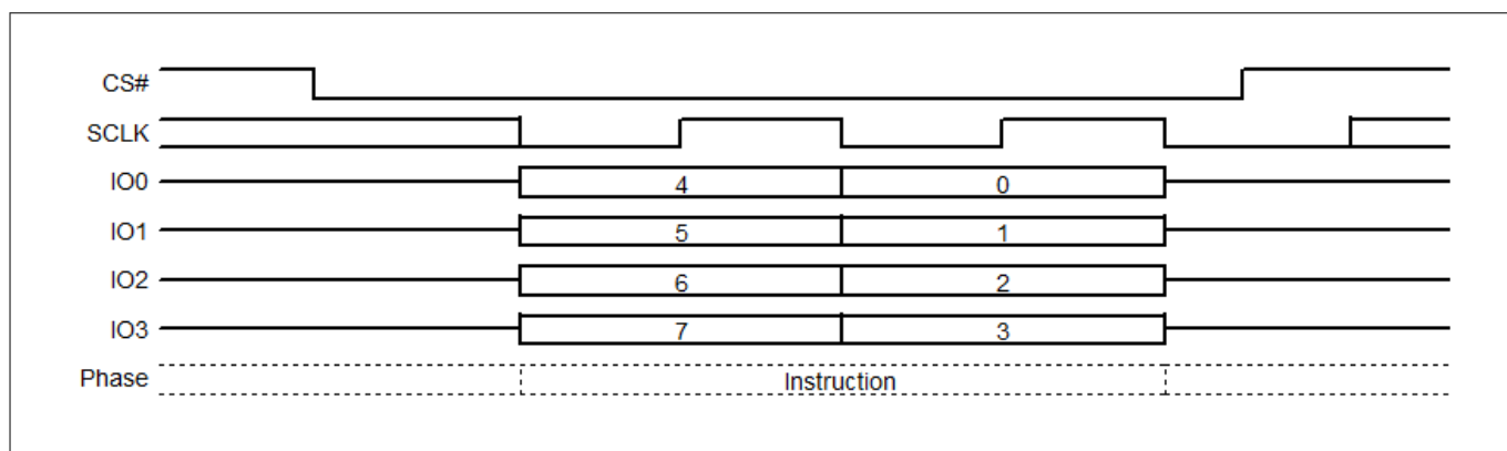
Figure 122 Software reset / Mode Bit command sequence – QPI mode
