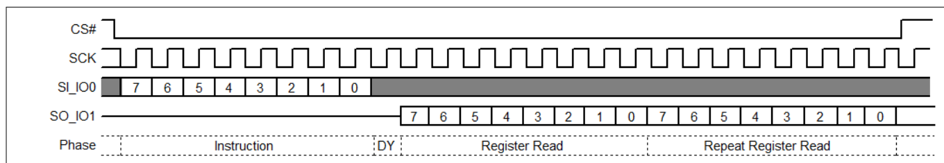
Figure 111 Protection Register Read (PRRD) command sequence
