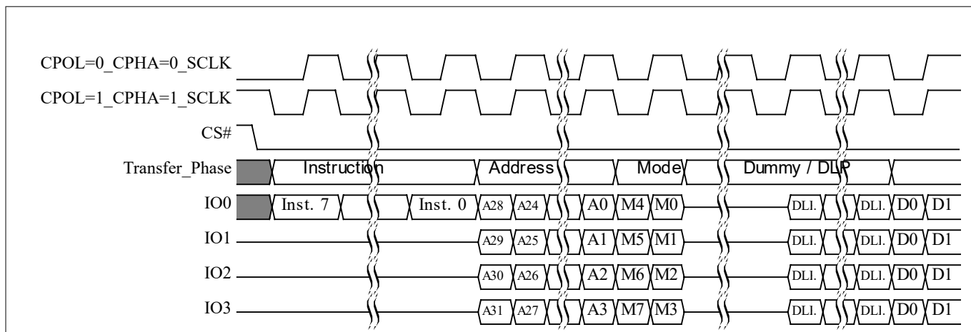
Figure 12 SPI DDR modes supported
