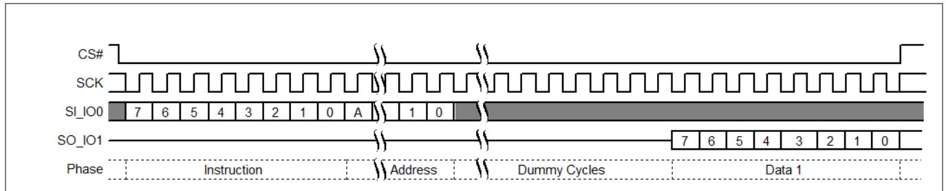
Figure 31 RSFDP command sequence
