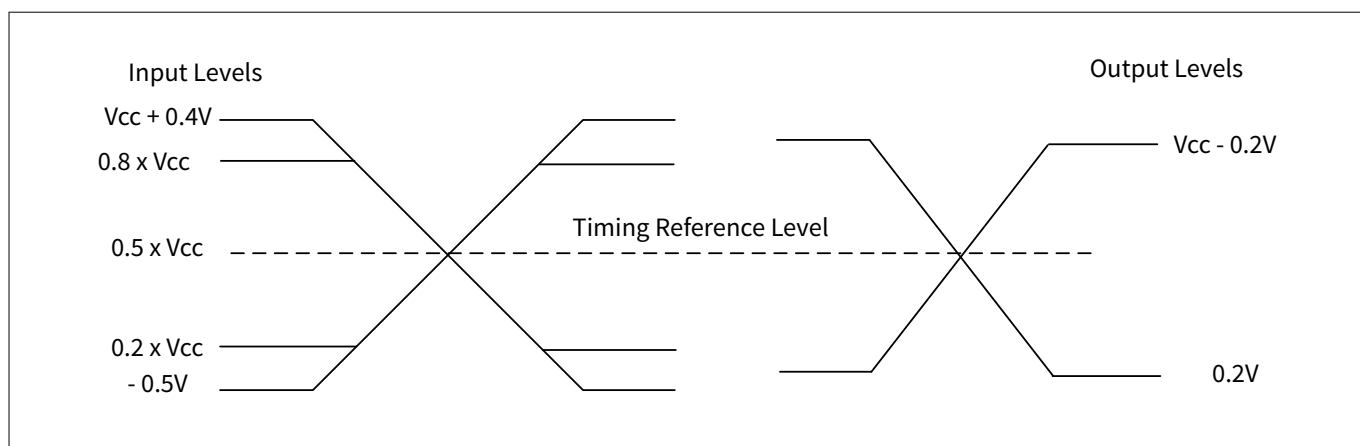
Figure 135 Input, output, and timing reference levels
