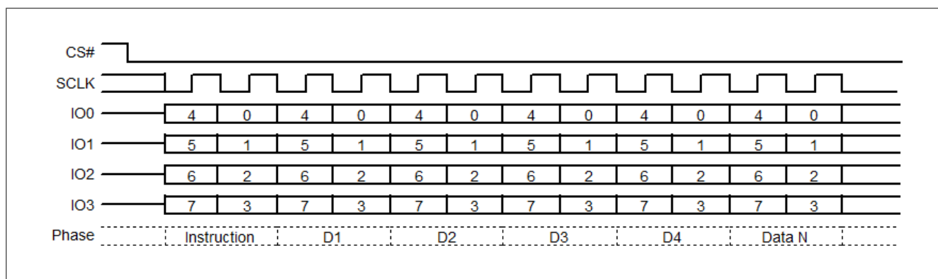
Figure 28 Read Identification (RDID) QPI mode command
