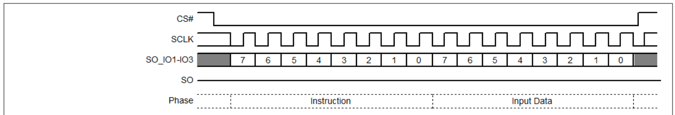
Figure 14 Single Bit Wide Input command
