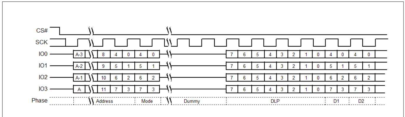
Figure 76 Continuous DDR Quad I/O Read subsequent access
