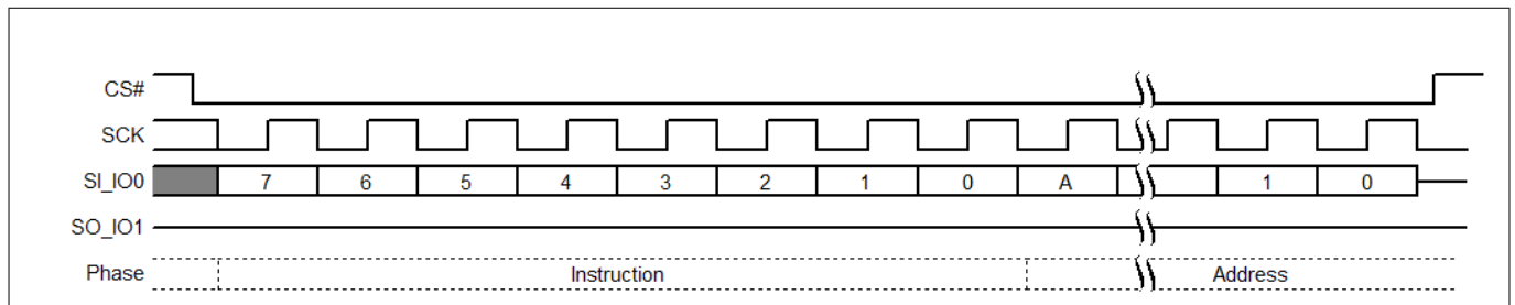
Figure 105 SPRP command sequence
