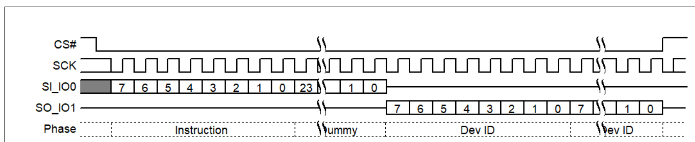
Figure 127 Read Identification (RES) command sequence
