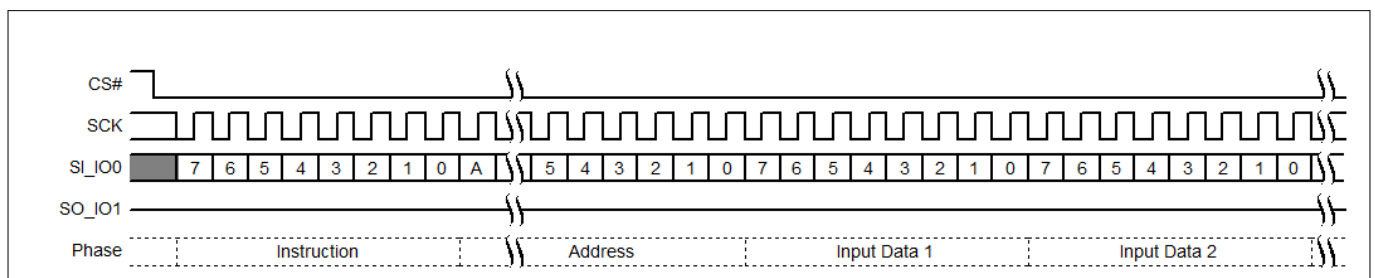
Figure 77 Page Program (PP 02h or 4PP 12h) command sequence
