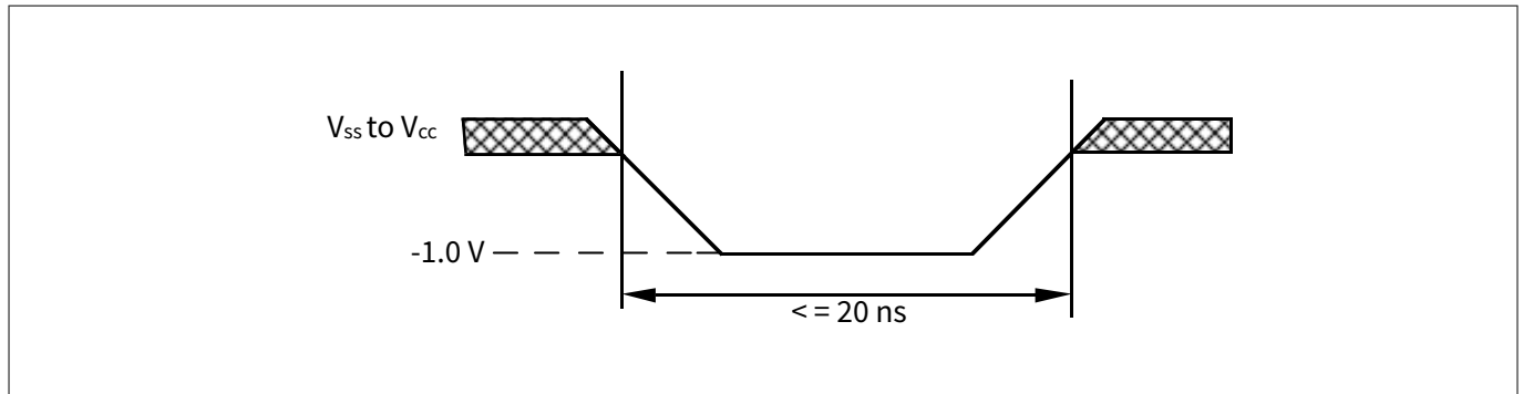
Figure 129 Maximum negative overshoot waveform
