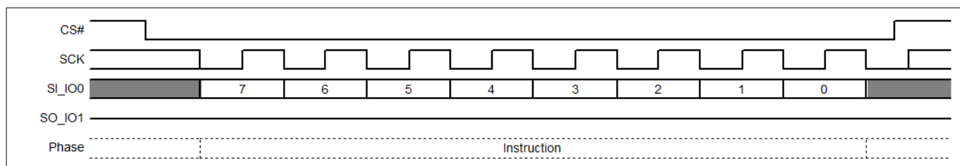
Figure 121 Software / Mode Bit Reset command sequence
