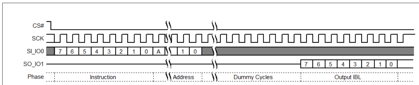
Figure 95 IBLRD command sequence
