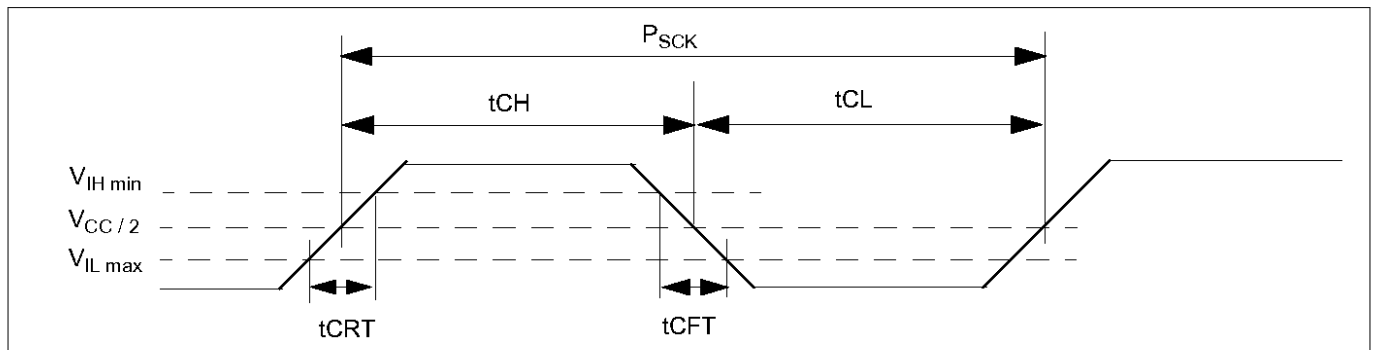
Figure 142 Clock timing
