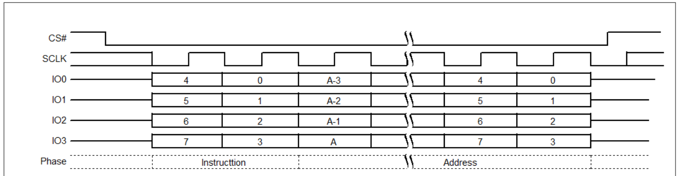
Figure 100 IBUL command sequence QPI mode
