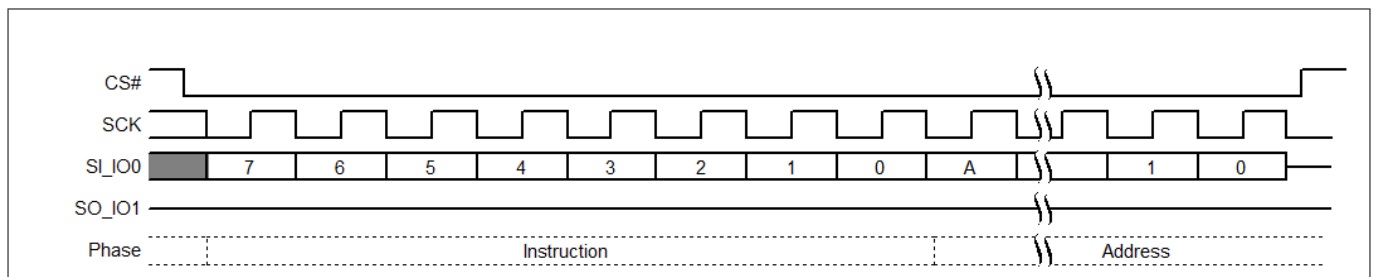
Figure 99 IBUL command sequence
