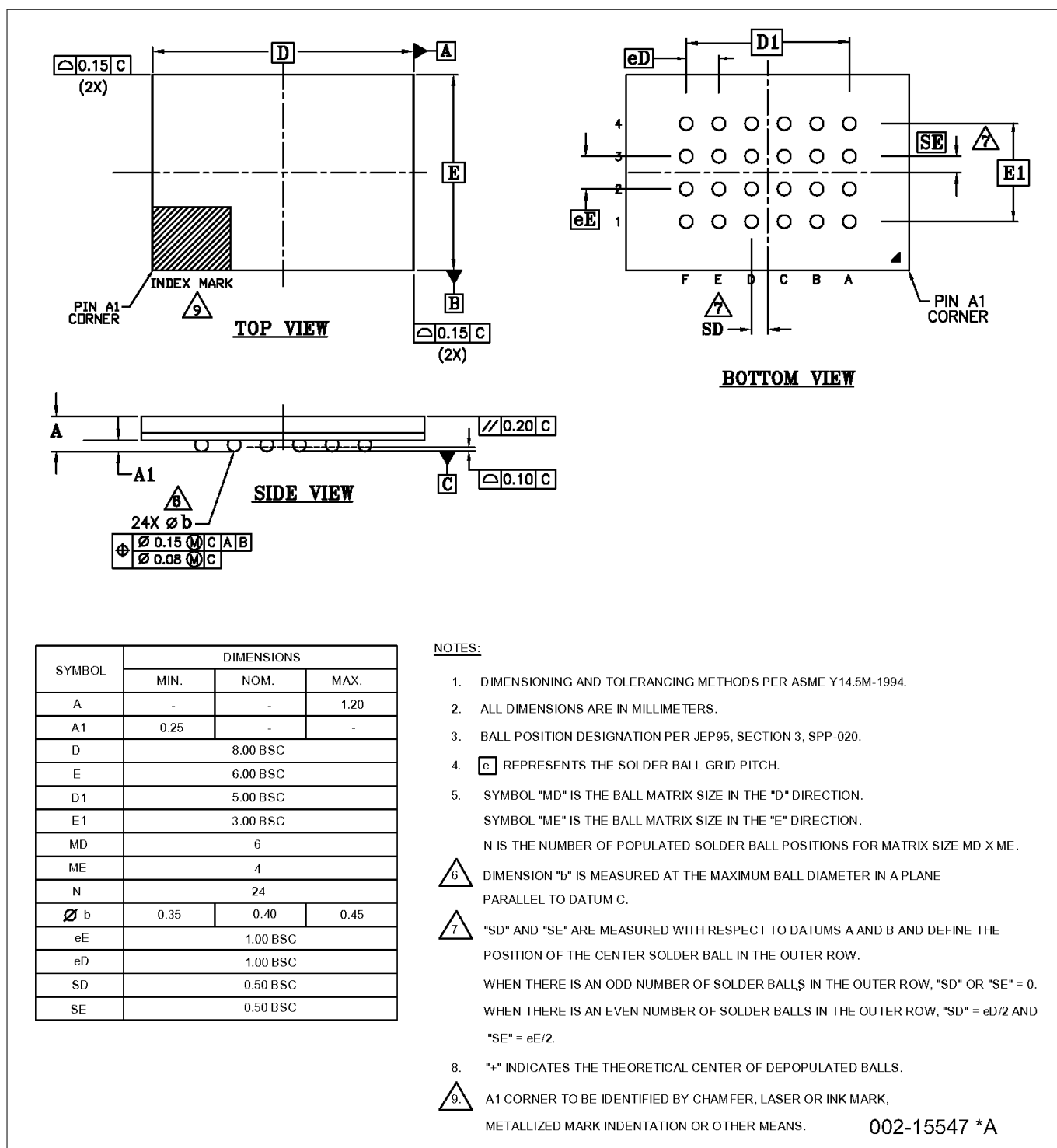
Figure 151 16-lead SOIC (10.30 × 7.50 × 2.65 mm) package outline (PG-DSO-16), 002-15547
