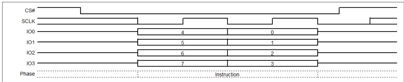
Figure 46 Write Enable for Volatile Registers (WRENV) command sequence QPI mode
