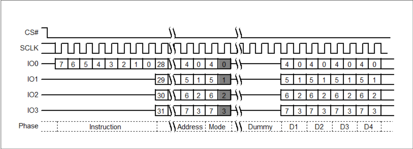
Figure 20 Quad I/O command
