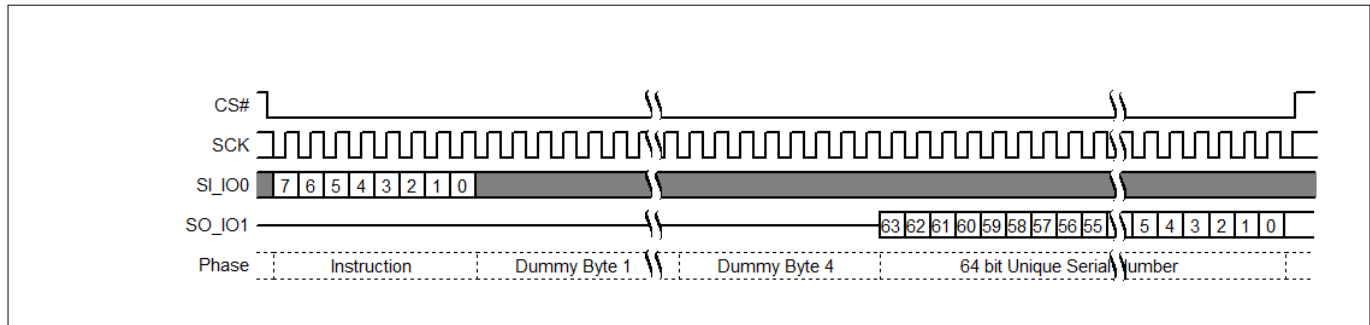
Figure 33 Read Unique ID (RUID) command sequence
