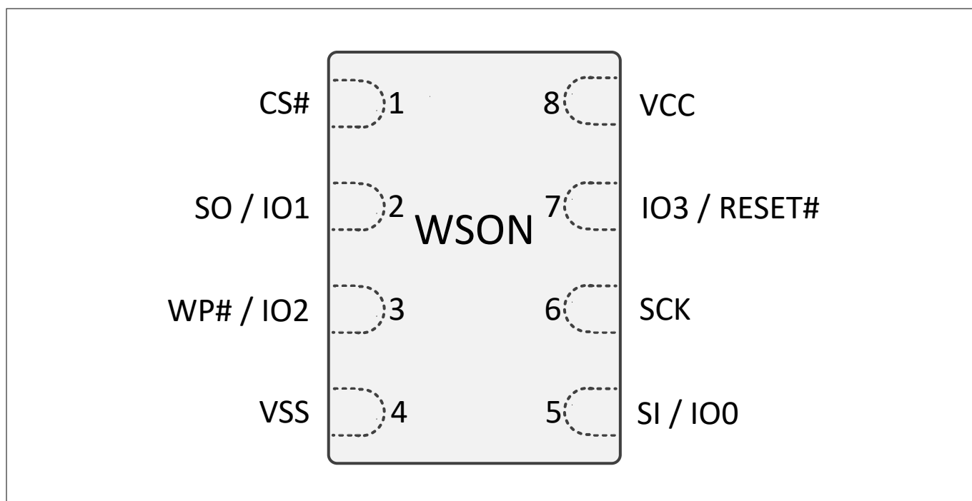
Figure 3 8-Connector package (WSO6) (WSO5), top view
