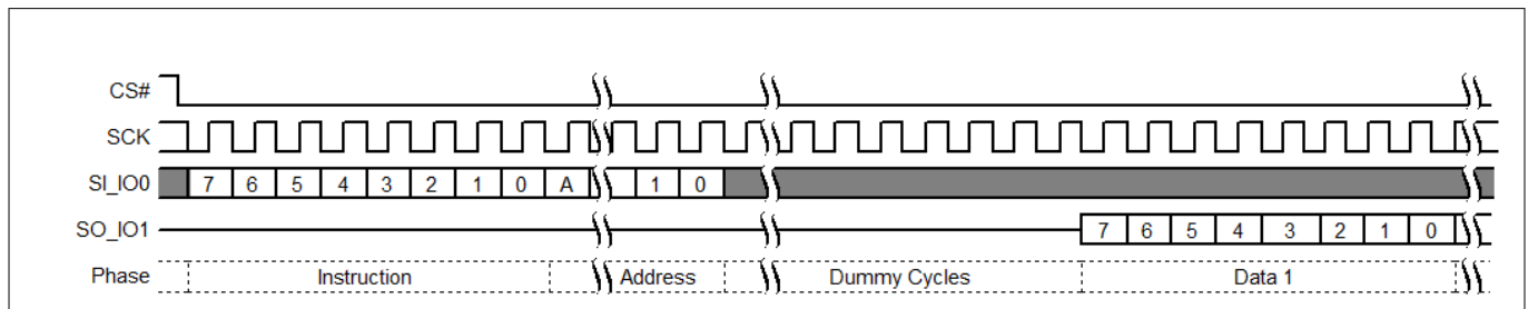
Figure 93 Security Regions Read command sequence
