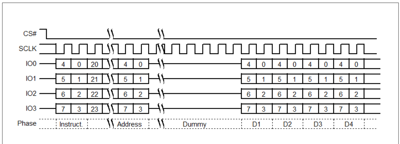
Figure 32 RSFDP QPI mode command sequence
