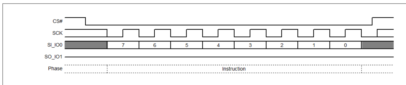
Figure 55 Enter 4 Byte Address Mode (4BEN B7h) command sequence
