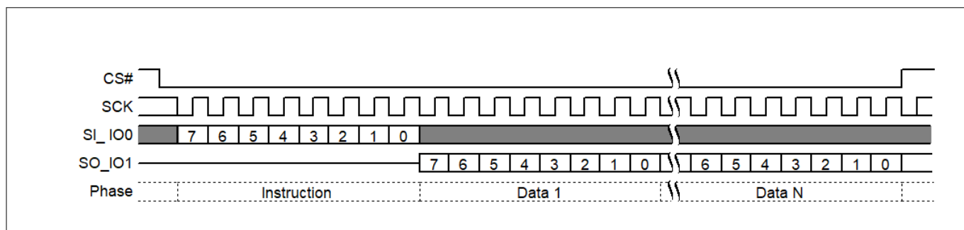
Figure 27 Read Identification (RDID) command sequence
