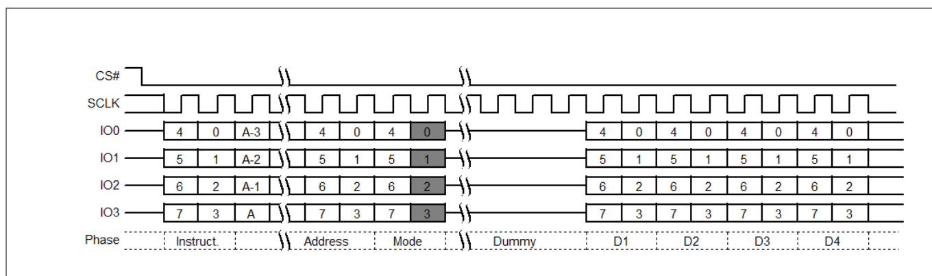
Figure 72 Quad I/O Read initial access command sequence QPI mode
