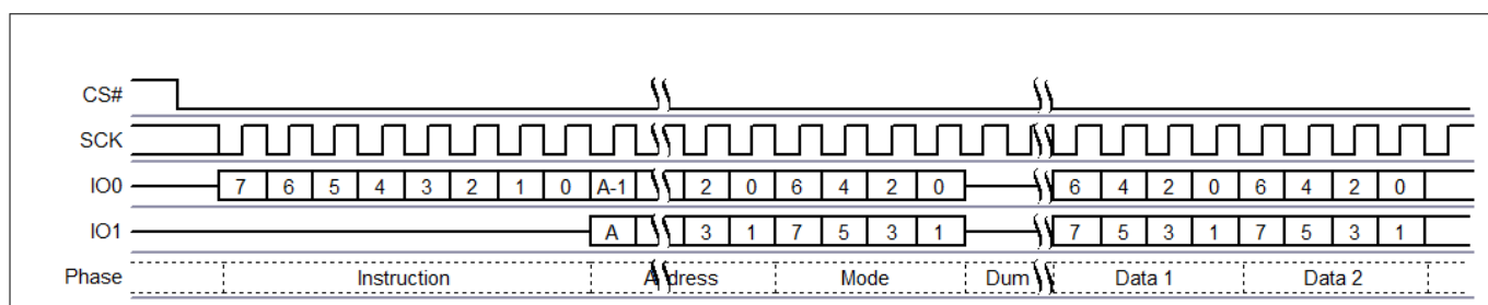
Figure 69 Dual I/O Read command sequence
