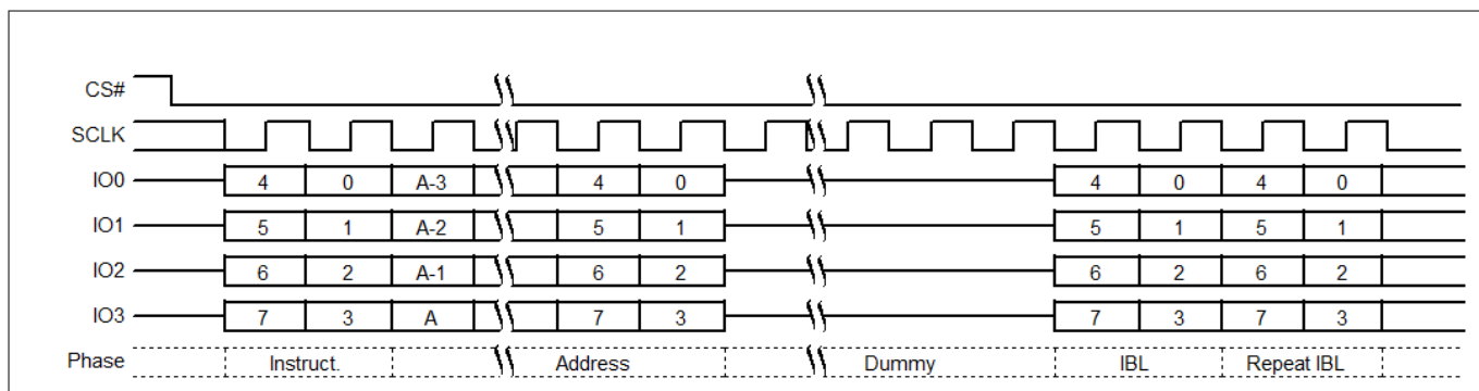
Figure 96 IBLRD command sequence QPI
