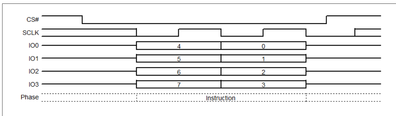
Figure 92 Erase or Program Resume command sequence QPI mode
