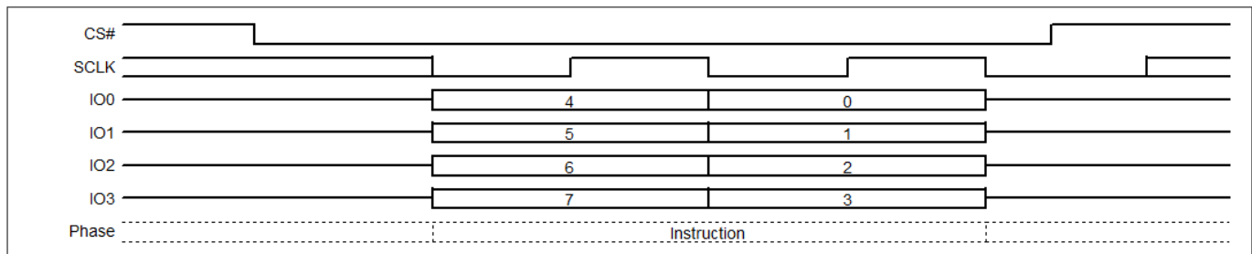
Figure 48 Clear Status Register (CLSR) QPI mode
