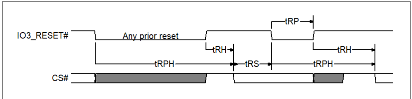
Figure 140 Hardware reset when quad or QPI mode is not enabled and IO3 / RESET# is enabled
