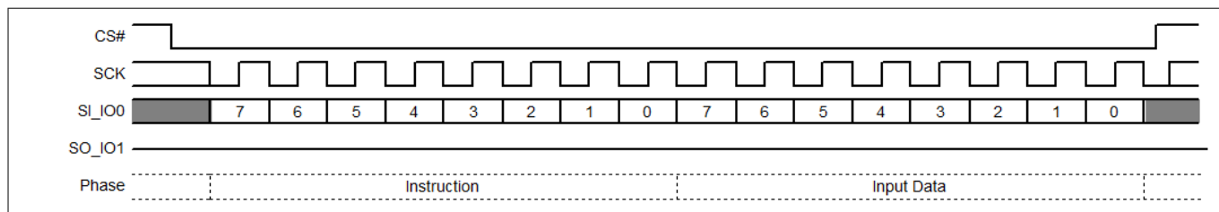
Figure 49 Program DLRNV (PDLRNV) command sequence
