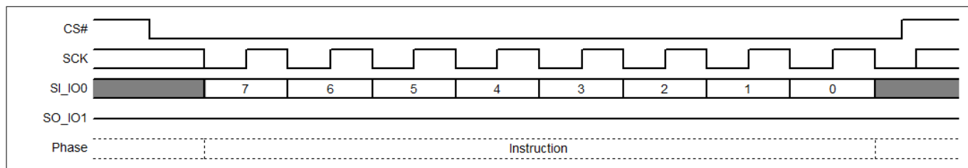
Figure 113 Protection Register Lock (PRL) command sequence
