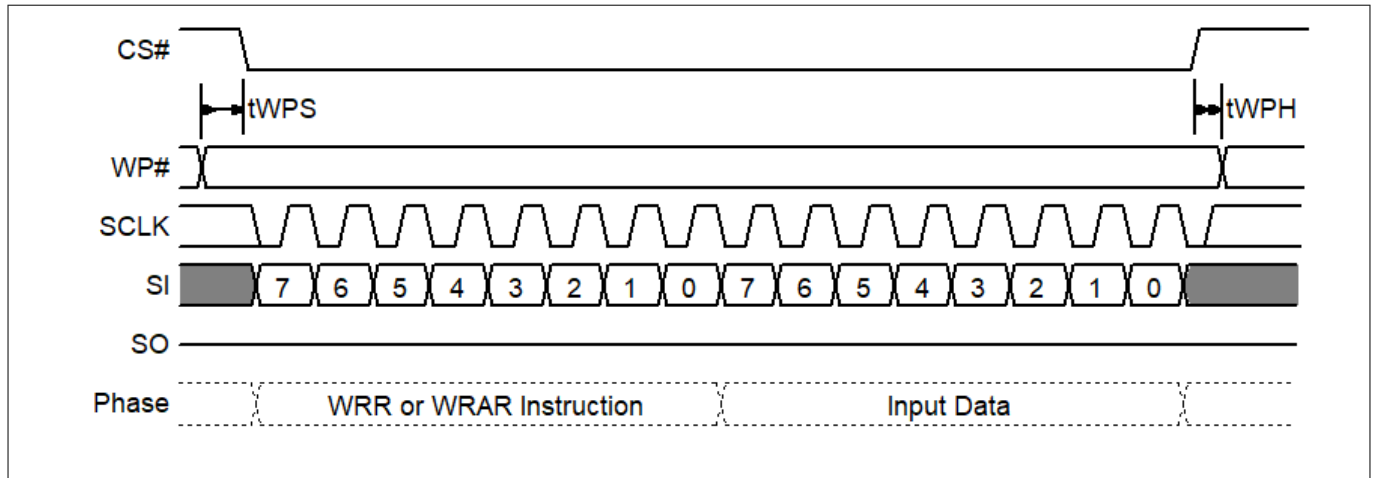
Figure 146 WP# input timing
