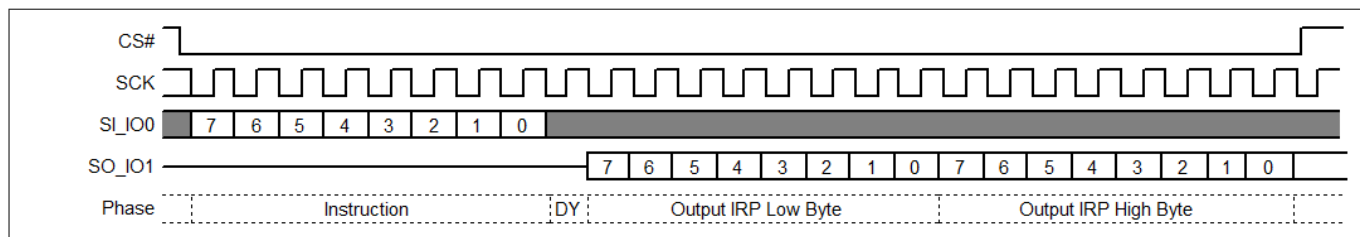
Figure 107 IRPRD command sequence
