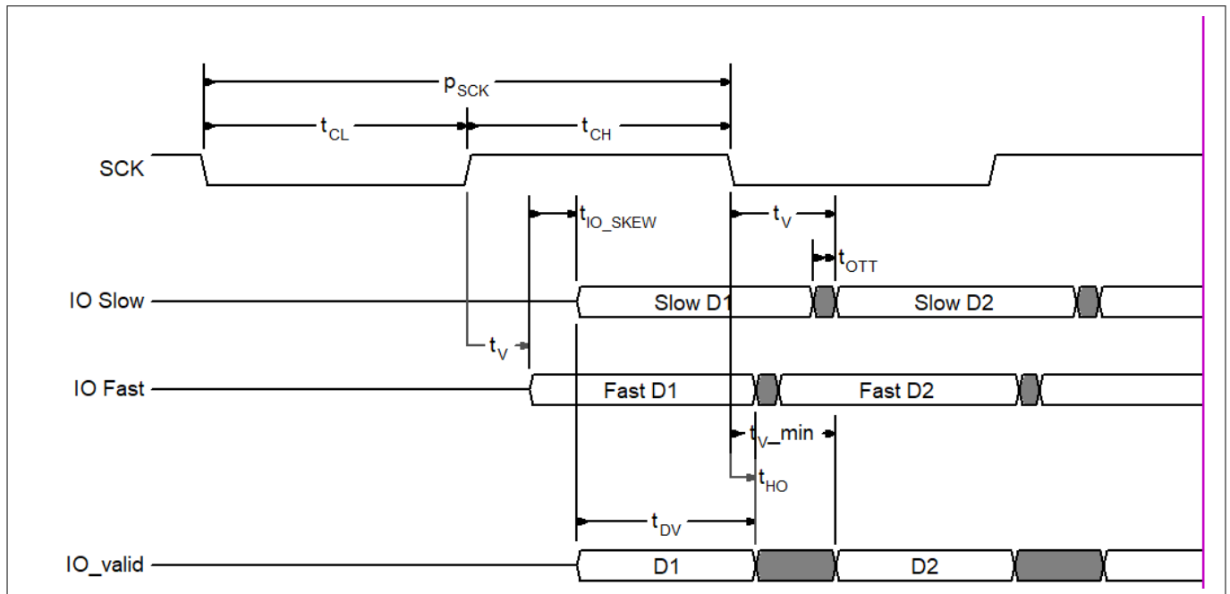
Figure 149 SPI DDR data valid window
