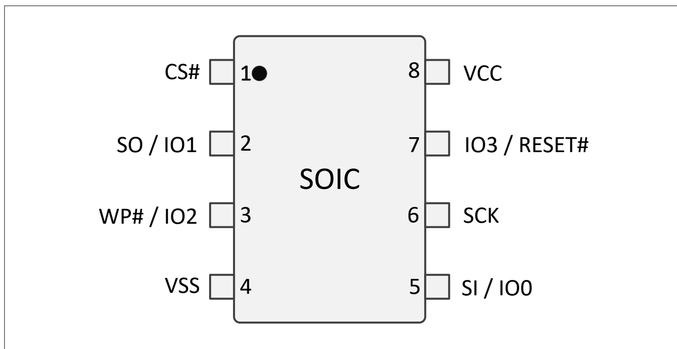
Figure 2 8-Pin plastic small outline package (SOIC8)
