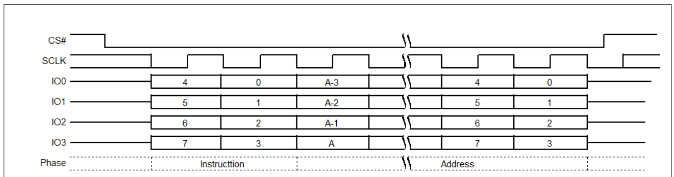
Figure 106 SPRP command sequence QPI mode
