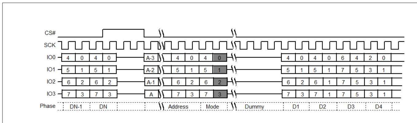
Figure 73 Continuous Quad I/O Read command sequence
