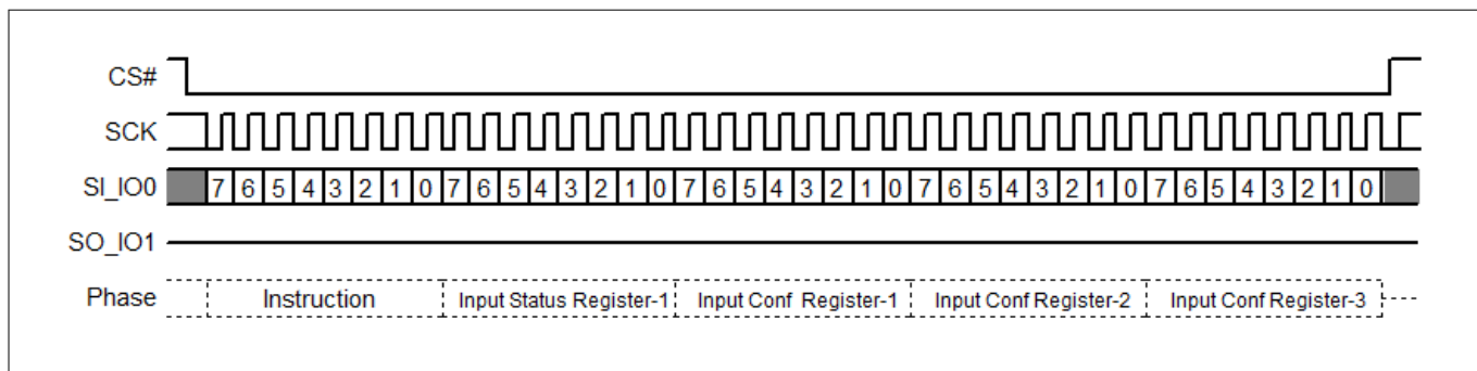
Figure 39 Write Registers (WRR) command sequence
