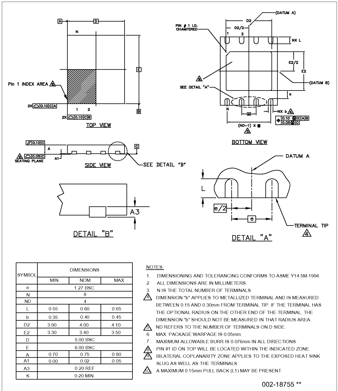
Figure 153 8-lead DFN ((5 × 6 × 0.8 mm) 4.0 × 3.4 mm E-Pad (Sawn)) package outline (PG-WSO8-8), 002-18755
