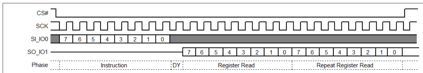
Figure 53 DLP Read (DLPRD) command sequence
