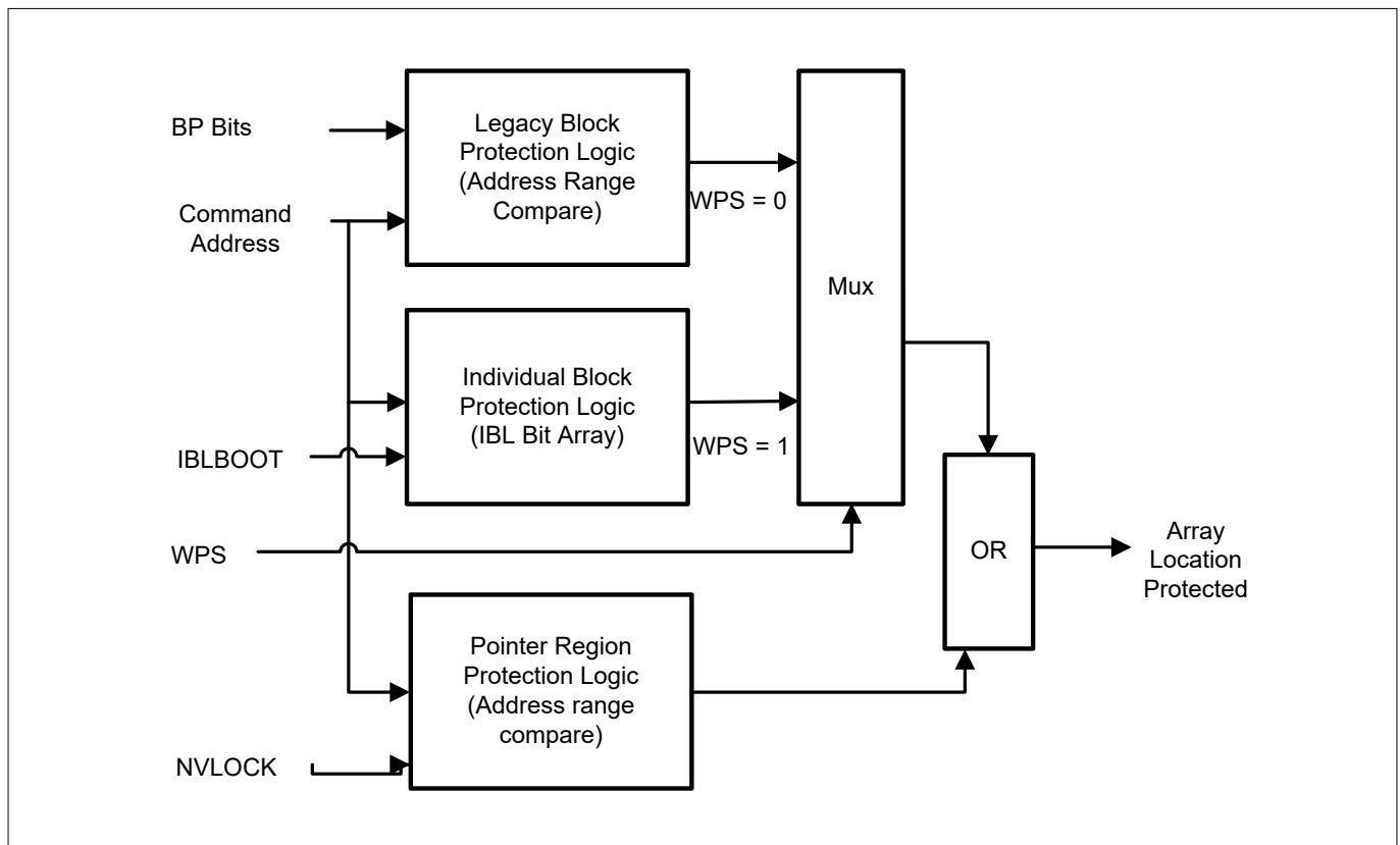
Figure 24 WPS selection of LBP or IBL and PRP array protection
